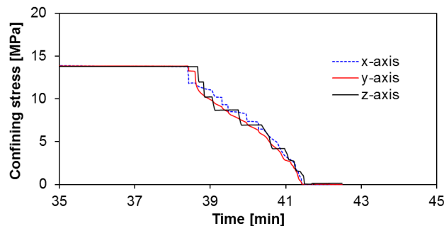
Figure 16. An example of synchronized unloading to avoid large stress anisotropy, using pressure relief valves in the hydraulic system.
