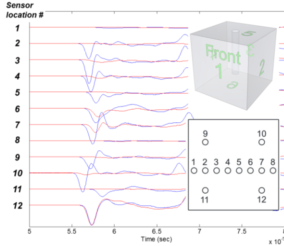
Figure 20. An example of P-wave signatures before (blue lines) and after (red lines) liquid nitrogen treatment in a concrete specimen (wave transmission between Faces 1&3).
