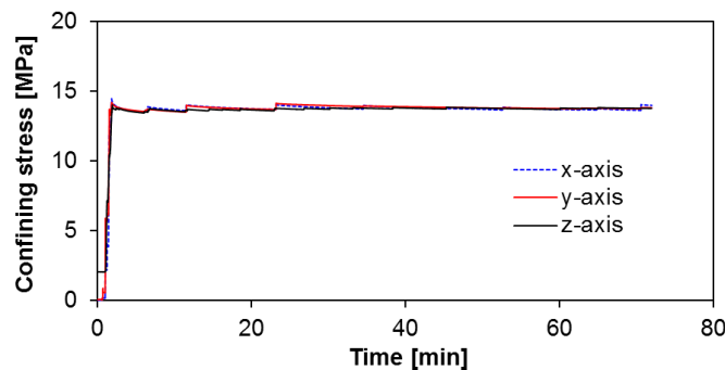
Figure 14. Confining load tests – manual control of constant stress (isotropic 14 MPa).
