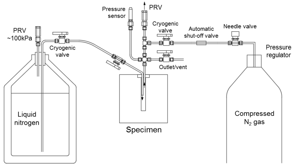
Figure 2. Basic schematic of lab cryogenic stimulation setup under low-pressure LN flow (the triaxial loading device not shown). Compressed nitrogen gas can be used to pressurize boreholes.
