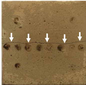
Figure 15. Prominent fracture along the centers at the sides in a concrete specimen created due to repeated, acute anisotropic conditions (sudden unloading of z-axis only).
