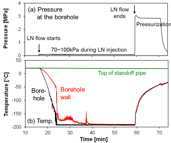
Figure 17. Borehole pressure and temperature during low-pressure LN flow followed by borehole pressurization in a concrete specimen under 14 MPa isotropic confining stress.
