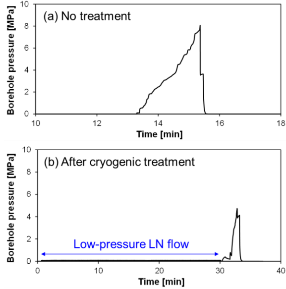
Figure 21. Post-stimulation breakdown fracturing of a concrete specimen by nitrogen gas pressure.
