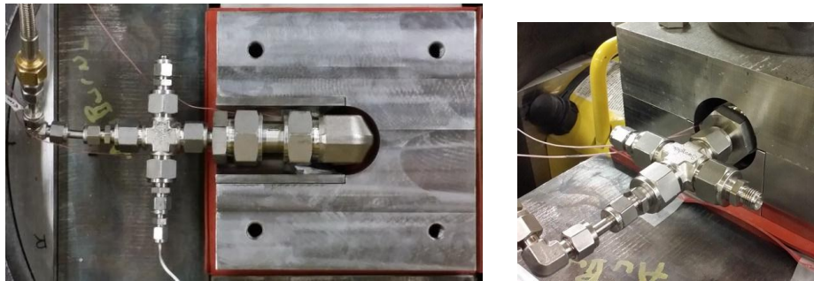
Figure 7. Setup for coaxial cryogen flow through – for confined specimen tests.
