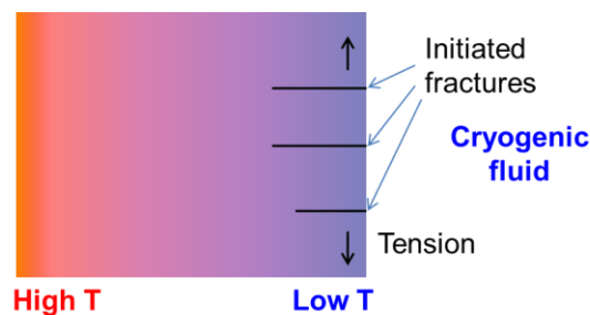
Figure 1. The basic concept of cryogenic fracturing.
