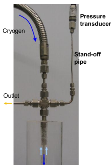
Figure 10. Stand-off pipe placed vertically to support measurements of borehole pressure.
