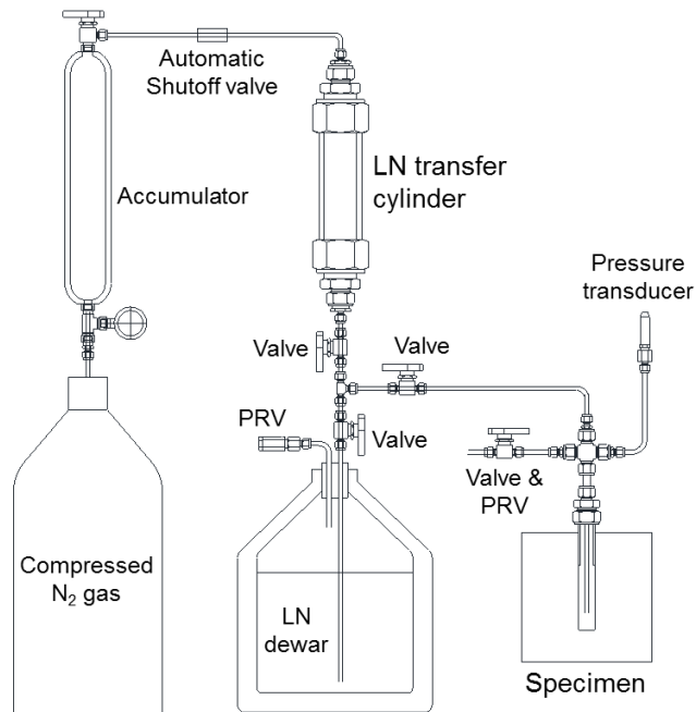
Figure 3. Schematic of lab cryogenic stimulation setup for higher-pressure LN flow. LN is temporarily stored in the transfer cylinder from the dewar, and compressed nitrogen gas is used to push LN to specimen boreholes.
