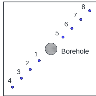
Figure 9. Locations of TC tips inside a concrete block at its mid-height for temperature measurements.
