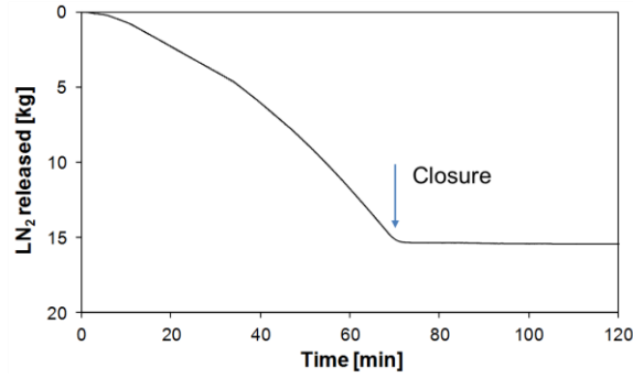
Figure 11. Typical liquid nitrogen consumption vs. time.
