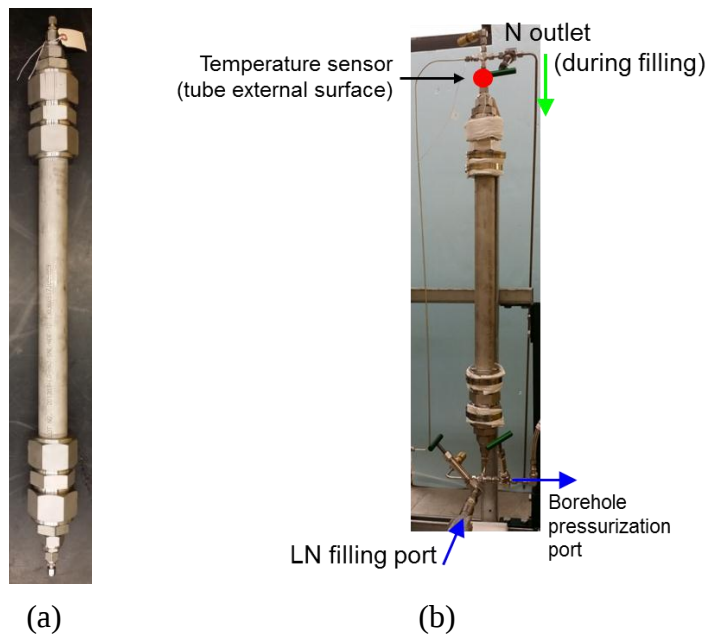
Figure 4. Liquid nitrogen transfer cylinder for higher-pressure LN flow. (a) 5.1cm-OD stainless steel tubing. (b) Assembled to the system. (Photo taken before applying insulation).
