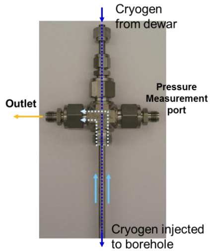
Figure 6. Coaxial design for cryogen flow through the borehole – for unconfined specimen tests (the casing detached to show the inner inlet pipe).
