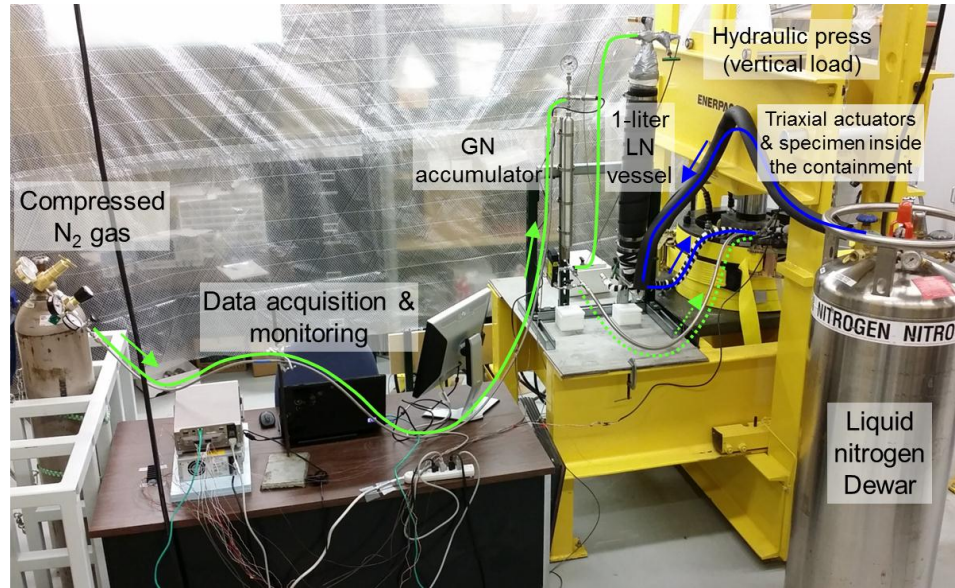
Figure 13. Assembled setup for cryogenic stimulation tests under specimen confining load. Green lines are tubes for pressurized gas nitrogen and blue lines are for tubes for liquid nitrogen.
