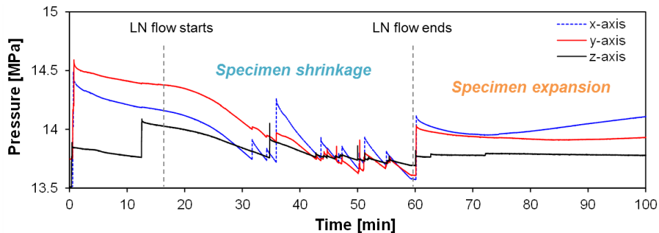
Figure 18. Shrinkage and expansion of a concrete specimen due to specimen cooling and warming, indicated from hydraulic pressure responses during low-pressure LN flow (followed by pressurization).
