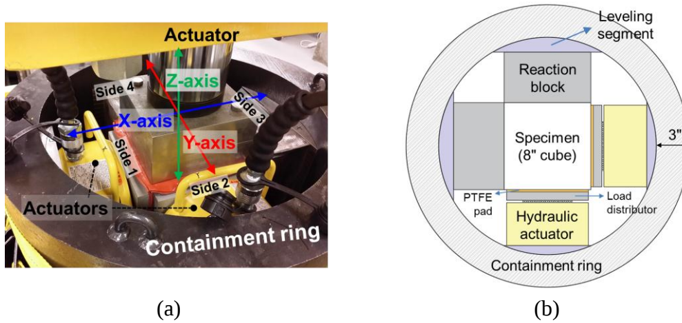
Figure 12. True-triaxial loading system. (a) Actuators and a specimen (not visible) inside the containment ring mounted on the press bed frame. Loading axes and specimen face numbers are indicated. (b) Plan view of the components laid in the containment.
