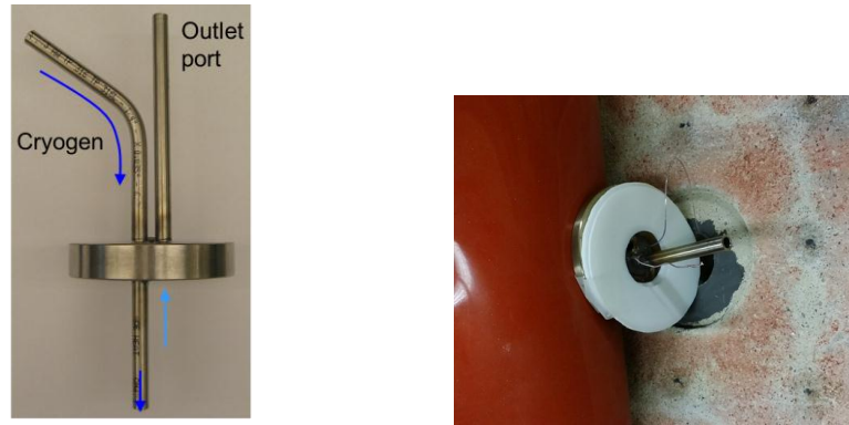
(a) Packer with inlet and outlet tubings (b) Silicone pad, packer and PTFE gasket
