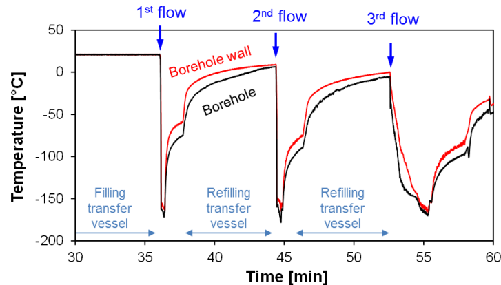
Figure 19. Temperature changes during multiple higher-pressure LN flow-through.
