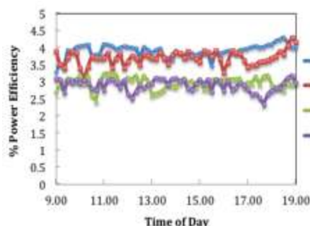
FIG. 9: The efficiency of the East and West-facing Criss Cross LSC panels and Clear panels throughout the day.
