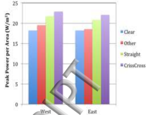
FIG. 7: The comparison of daily peak power over the course of a year produced by panels of varied design for both the West and East sides of the greenhouse. The “other” category on the West-facing side represents the Edge Cells design, and on the East-facing side represents the Polycrystalline Si design.
