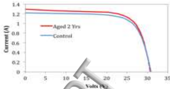
FIG. 6: The I-V curve of one of the panels at the start of the experiment (control) and after two years in the field. The fill factor for this panel is 72%. The other panels exhibit nearly identical I-V curves.
