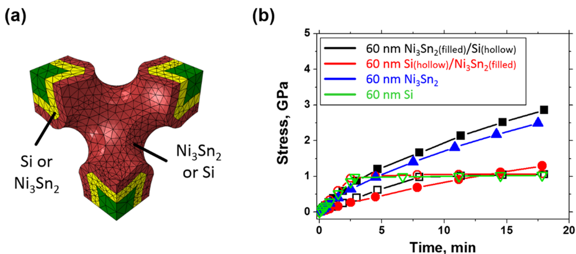
Figure 3. (a) Three-dimensional mesh systems of the RVE having thick active bilayers. Each active layer with 30 nm thickness can be either \text{Ni}_3\text{Sn}_2 or amorphous Si. (b) Comparison of the computed maximum von Mises stress (averaged over the 10% of elements with the highest von Mises values) evolutions in each of the layers of the bilayers: Si/ \text{Ni}_3\text{Sn}_2 (where Si is the outer layer) and \text{Ni}_3\text{Sn}_2 /Si (where Si is the inner layer) during the first lithiation half-cycle. For comparison, the computed maximum von Mises stress evolutions in the single layer cases are also shown.
