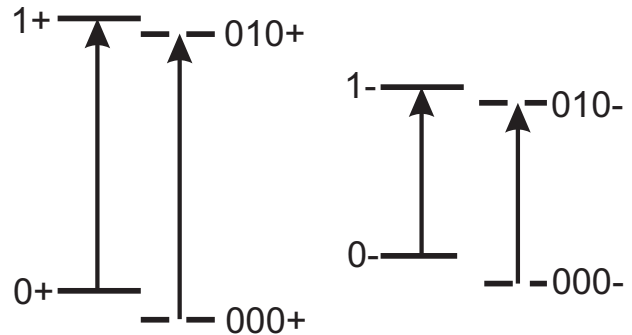
FIG. 4. Cyclotron resonance and MD cyclotron resonance transitions for both spin orientation. It is seen that for the LL number of 0 the 0- is higher as 0+ and in the case of LL number 1 is contrary the 1+ is higher as 1- .
