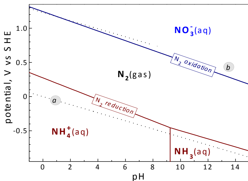
Figure 4. Partial Pourbaix diagram for the \text{N}_2\text{-H}_2\text{O} system showing solid lines corresponding to \text{N}_2 reduction to \text{NH}_4^+/\text{NH}_3 and \text{N}_2 oxidation to \text{NO}_3^- . Dotted lines a and b straddle the region of water stability (reduction to \text{H}_2 and oxidation to \text{O}_2 , respectively). See (14) for details and (15, 19) for primary data.
