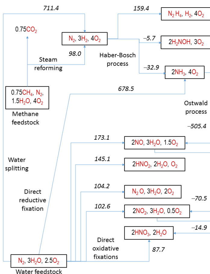
Figure 1. Atom and energy economy of nitrogen fixation. The numerical values represent standard (14) Gibbs free energies in kJ/mol of fixed N_2 in the direction of the arrows. All thermochemical data are from (15), except for H_2NOH (16).
