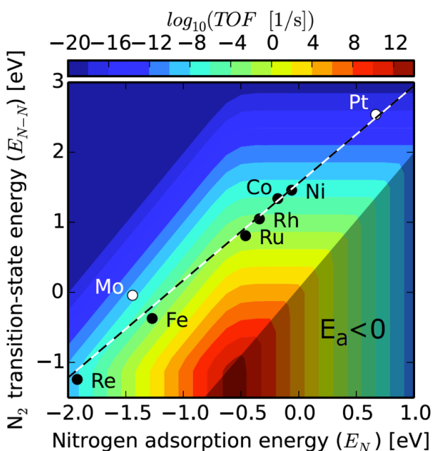
Figure 2. Linear scaling between nitrogen binding energy and activation barrier for N_2 dissociation. TOF = turnover frequency. Reproduced with permission from (22).
