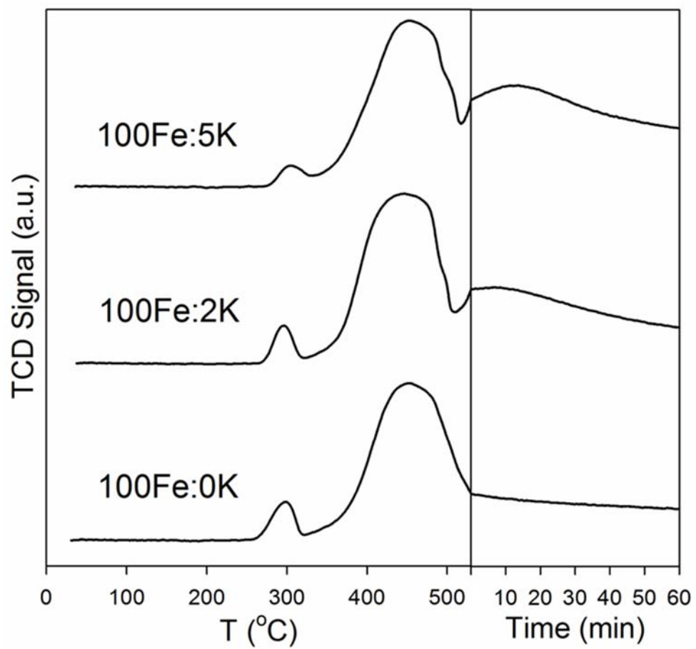
Figure 1: CO TPR profiles of 100Fe:0K, 100Fe:2K, and 100Fe:5K catalysts.
