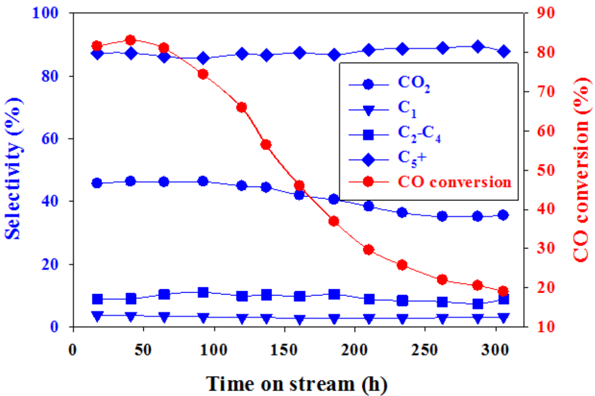
Figure 4: Hydrocarbon and CO 2 selectivity against time on stream for a 100Fe:2.0K catalyst.
