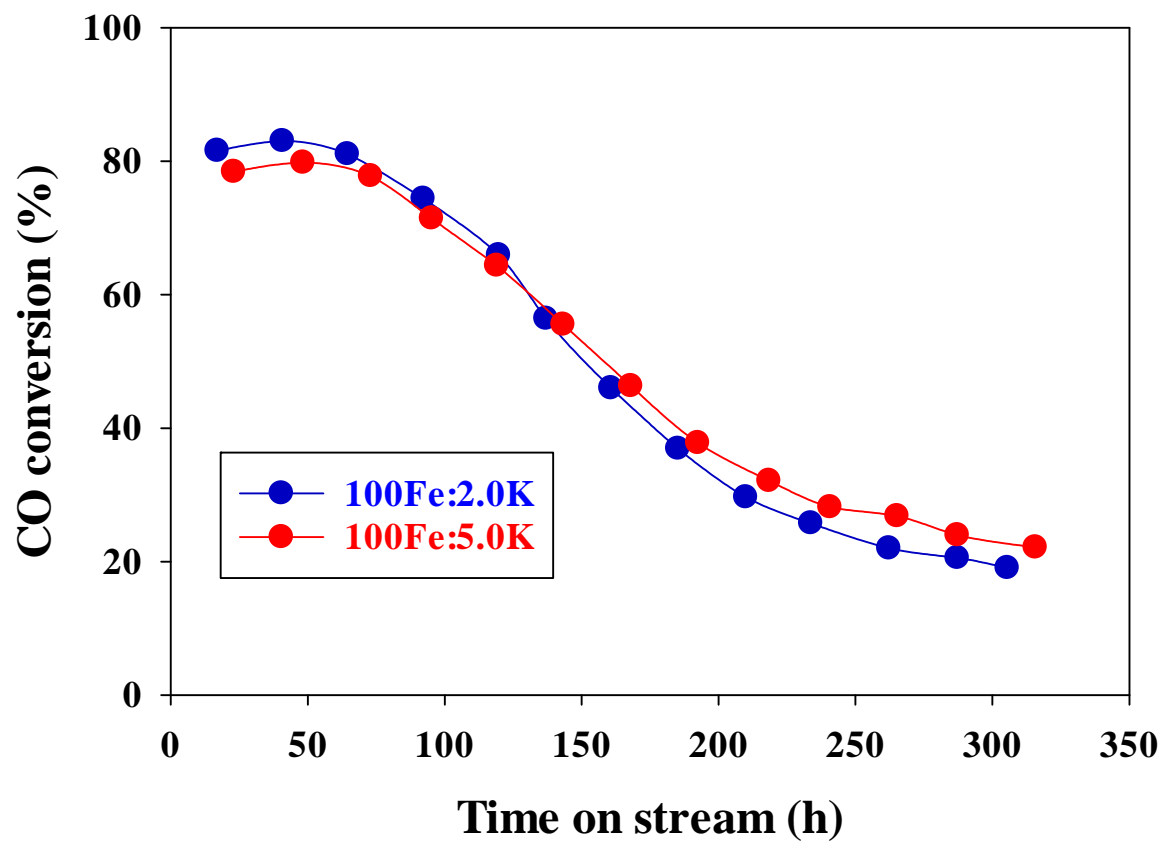
Figure 2: CO conversion against time on stream for various potassium loaded iron catalysts.
