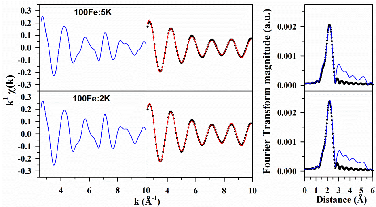
Figure 8: EXAFS spectra at the K-edge of Fe for end-of-run 100Fe:5K and 100Fe:2K catalysts, including (left) raw \chi(k) versus k spectra; (middle) (red) filtered \chi(k) versus k and (filled circles) result of the EXAFS fitting; and (right) (blue) raw k^1 -weighted Fourier transform magnitude and (filled circles) result of the EXAFS fitting.
