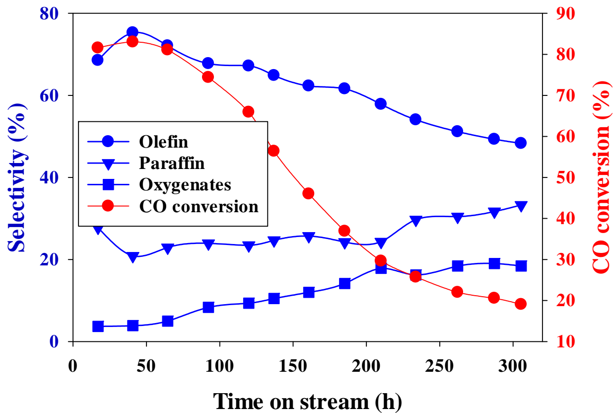
Figure 3: CO conversion and product selectivities against time on stream of 100Fe:2.0K catalyst
