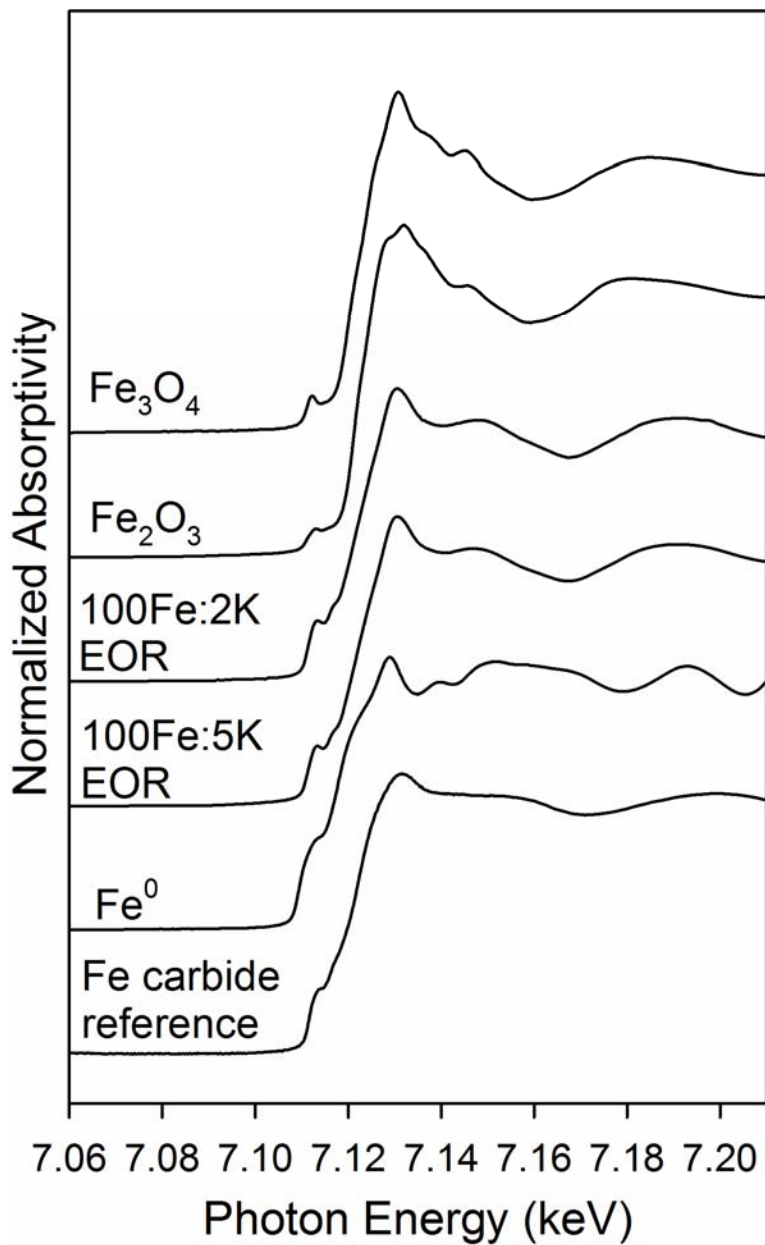
Figure 7: Normalized XANES spectra at the K-edge of Fe for reference compounds and end-of-run (EOR) 100Fe:5K and 100Fe:2K catalysts. Note that the Fe carbide reference was following a CO-TPR/XANES experiment for a Fe:1.5K catalyst (details provided elsewhere [3]).
