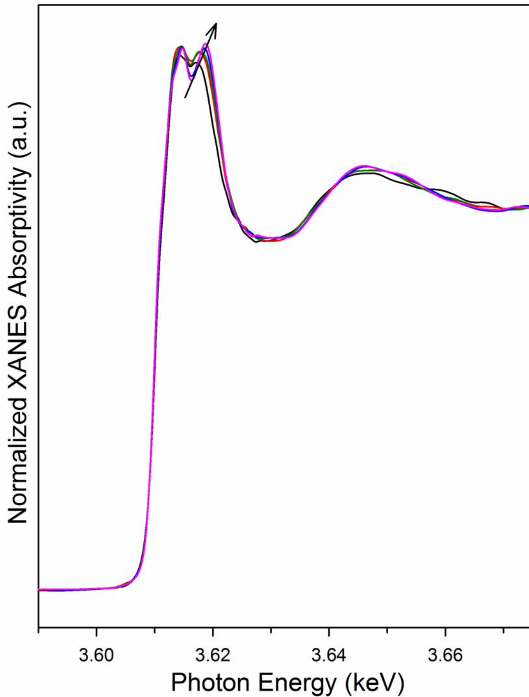
Figure 5: Normalized K K-edge XANES spectra of the 100Fe:2K catalyst (black) following activation in CO at 425°C for 6 h and, moving along the trajectory of the arrow, after running Fischer-Tropsch synthesis for (red) 24 h, (green) 48 h, (blue) 95 h, and (pink) 165 h.
