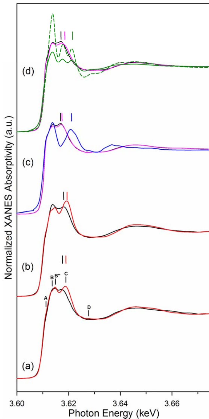
Figure 6: Normalized K K-edge XANES spectra of (a) 100Fe:2K and (b) 100Fe:5K catalysts (black) after activation and (red) following the Fischer-Tropsch synthesis reaction test; (c) (black) 0.97% \text{K}_2\text{CO}_3/\text{SiO}_2 , (pink) 2.38% \text{K}_2\text{CO}_3/\text{SiO}_2 , and (blue) bulk \text{K}_2\text{CO}_3 ; and (d) (black) 0.97% \text{KHCO}_2/\text{SiO}_2 , (pink) 2.38% \text{KHCO}_2/\text{SiO}_2 , and (green) bulk \text{KHCO}_2 .
