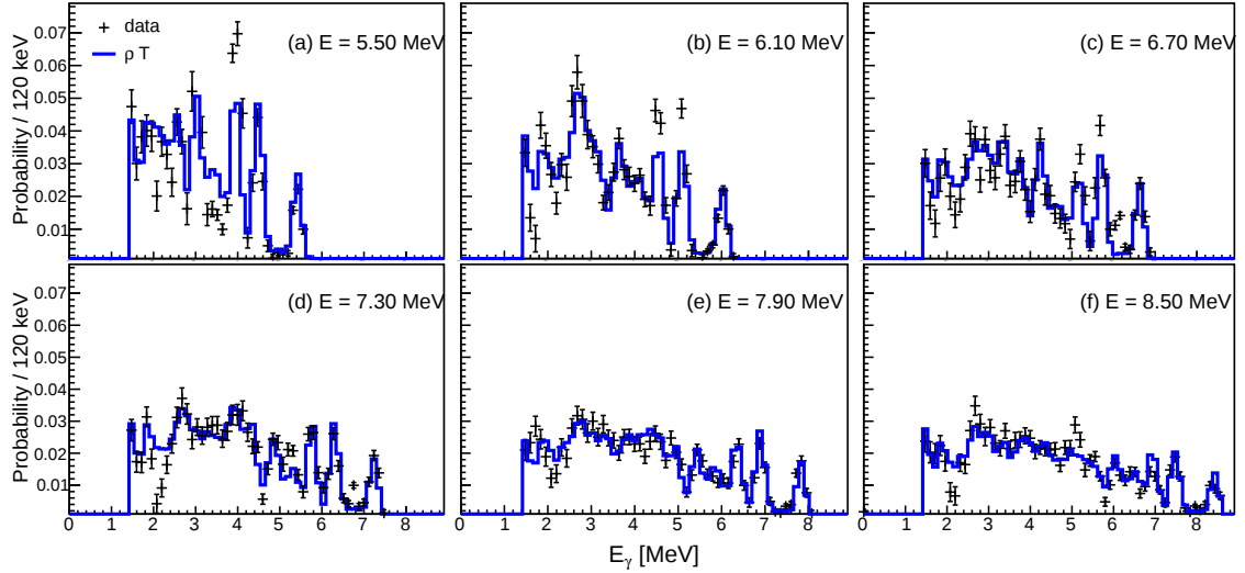
FIG. 5: (Color online) Same as Fig. 4 for ^{92}\text{Zr} . Both the \gamma and excitation energy dispersions are 120 keV/ch.
