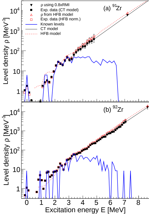
FIG. 6: (Color online) Normalized NLDs of ^{91,92}\text{Zr} extracted from the present experiment. At low excitation energies, the data are normalized to known discrete levels (solid blue line). At higher excitation energies, the data are normalized to \rho at S_n using resonance spacing D_0 . Two normalization procedures for \rho(S_n) are used: (i) the spin cutoff parameter listed in Table III together with the CT NLD parameters (black lines and symbols) and (ii) the HFB plus combinatorial model (red dashed lines and symbols) [31].
