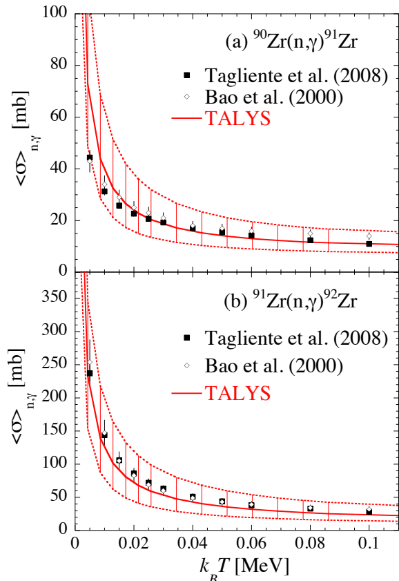
FIG. 10: (Color online) Comparison between the experimental ^{90}\text{Zr}(n,\gamma)^{91}\text{Zr} Maxwellian-averaged cross section [26, 55] and the one obtained with the TALYS code on the basis of the NLD and \gamma SF derived experimentally in the present work. (b) Same for ^{91}\text{Zr}(n,\gamma)^{92}\text{Zr} Maxwellian-averaged cross section with experimental data taken from Refs. [27, 55].
