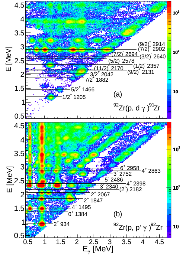
FIG. 1: (Color online) The discrete part of the particle- \gamma coincidence matrices for the (a) ^{92}\text{Zr}(p, d)^{91}\text{Zr} and (b) ^{92}\text{Zr}(p, p')^{92}\text{Zr} reactions. Only excitation energies between 0.5 and 4.5 MeV are shown in order to highlight the decay pattern recognized in the present experiment. The pixel width is 16 keV \times 16 keV.
