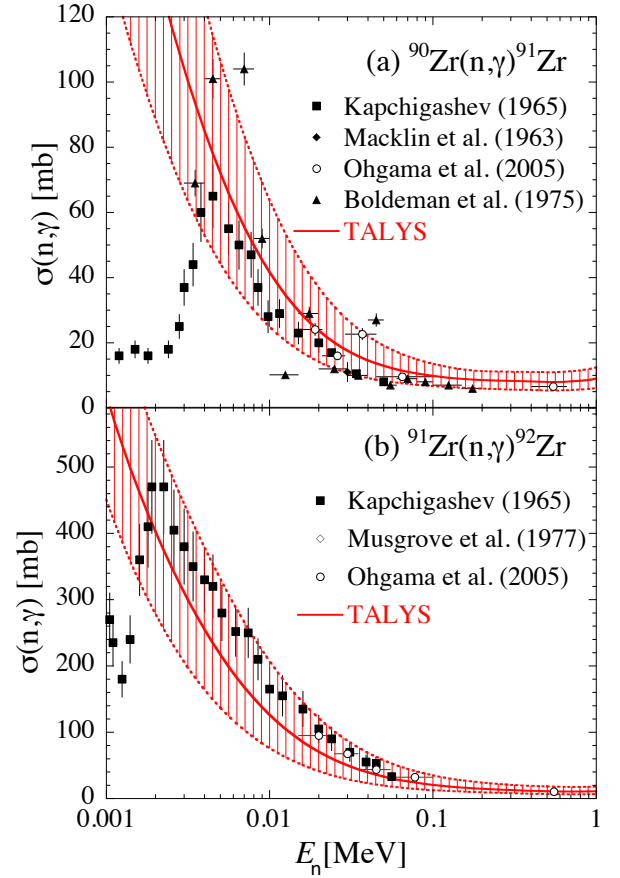
FIG. 9: (Color online) (a) Comparison between the experimental ^{90}\text{Zr}(n, \gamma)^{91}\text{Zr} cross section [51–53] and the one obtained with the TALYS code on the basis of the NLD and \gamma\text{SF} derived experimentally in the present work. The hashed area depicts all the experimental and model-dependent uncertainties taken into account in the present analysis. (b) Same for ^{91}\text{Zr}(n, \gamma)^{92}\text{Zr} cross section with experimental data taken from Refs. [51, 53, 54].
