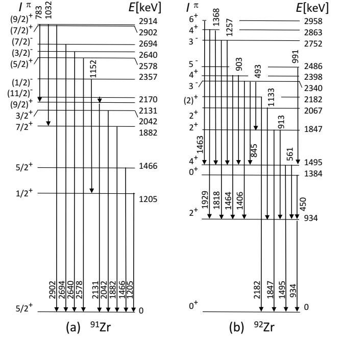
FIG. 3: Partial level schemes for (a) ^{91}\text{Zr} and (b) ^{92}\text{Zr} . Only the levels, which are most strongly populated in the (p,p') and (p,d) reactions, respectively, are shown. The most prominent \gamma -rays from these states are displayed with \gamma energies in keV. More complete level schemes are found in Ref. [17].
