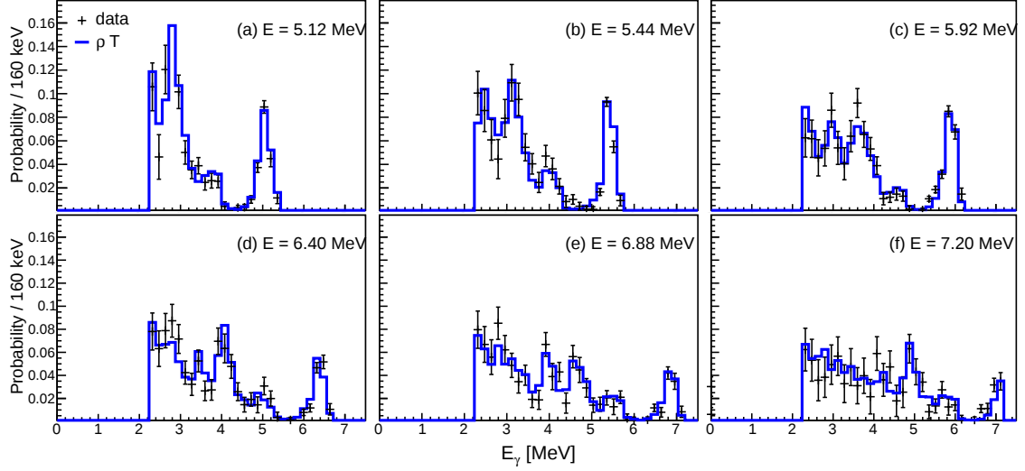
FIG. 4: (Color online) Primary \gamma -ray spectra from various initial excitation energies E (crosses) in ^{91}\text{Zr} . The spectra are compared to the product \rho(E - E_\gamma)\mathcal{T}(E_\gamma) (blue histogram). Both the \gamma and excitation energy dispersions are 160 keV/ch.
