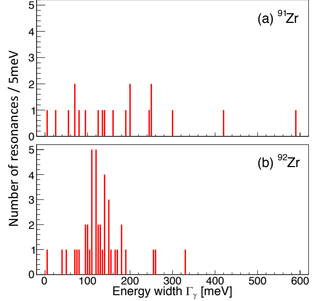
FIG. 7: (Color online) The number of \ell = 0 resonances as function of their specific \gamma width \Gamma_\gamma . For ^{91}\text{Zr} , 15 resonances are taken from Ref. [26] and additional 5 from Ref. [28]. For ^{92}\text{Zr} , the 42 resonances are taken from Ref. [27]. The data are used to re-evaluate the average \gamma width, called \langle \Gamma_{\gamma 0} \rangle_B in column 6 of Table I.
