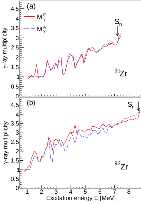
FIG. 2: (Color online) The \gamma -ray multiplicity measured as function of excitation energy for the (a) ^{92}\text{Zr}(p,d)^{91}\text{Zr} and (b) ^{92}\text{Zr}(p,p')^{92}\text{Zr} reactions. The energy bin is 120 keV.
