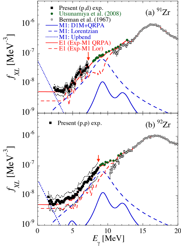
FIG. 8: (Color online) (a) Experimental 91 Zr \gamma SFs (solid squares) with its error band (dotted lines) due to the uncertainty in \sigma , D_0 and \langle\Gamma_{\gamma 0}\rangle (see Table III). Also shown are the photoneutron data [7, 37], the spin-flip M1 strength derived from either DIM+QRPA calculations (solid blue line) or a Lorentzian function (dashed blue line) and the M1 upbend (dotted blue line). The resulting recommended E1 strength is shown by a solid (dashed) red line and obtained from the total experimental dipole strength by subtracting the DIM+QRPA (Lorentzian) M1 component. The neutron separation energies are indicated by arrows. (b) Same for the 92 Zr \gamma SFs.
