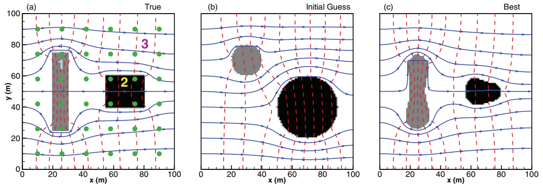
Figure 4: Comparison of (a) the true permeability field, (b) initial guess, and (c) the best results in terms of the minimum residual from 700 iterations, for Case 1, which has three materials.
