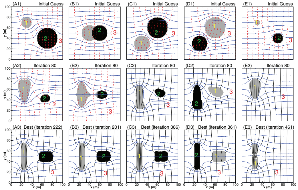
Figure 10: Sensitivity of inverse results on the initial guess field. The true zonation is the same as that in Case 1. Top row shows 5 initial guesses, the middle row for their corresponding snapshots at iteration 80, and the bottom row for the best results.
