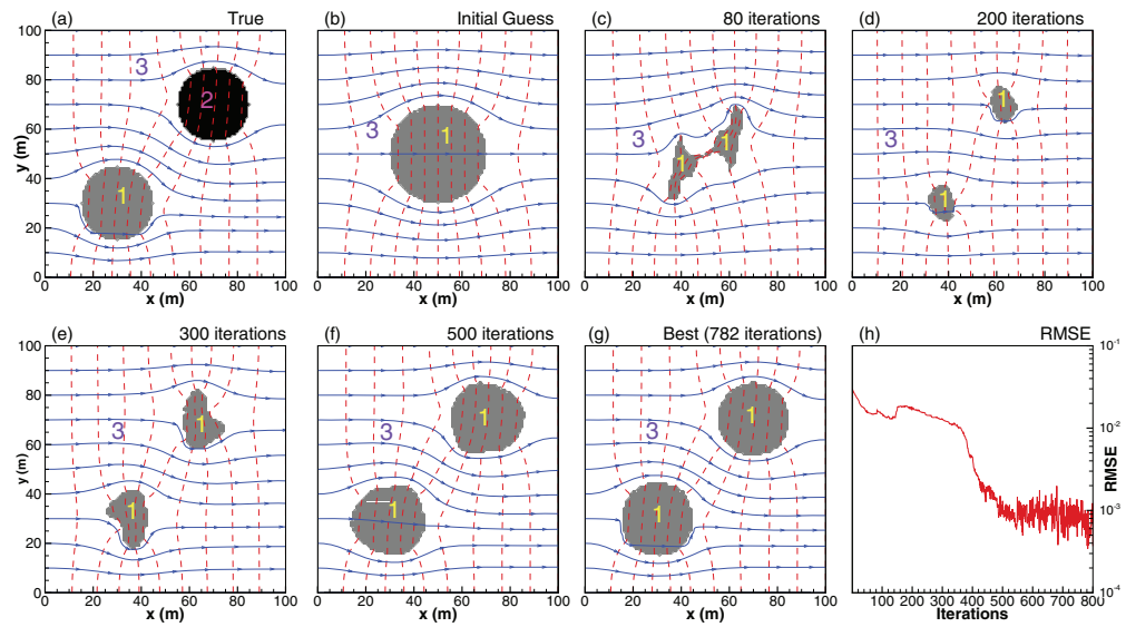
Figure 9: Evolution of lower permeable inclusions for Case 4, where the true field has two lower permeable materials (a), but the guess field has one lower permeable material because of lacking accurate information about the number of materials. Plots (b)-(f) illustrate some snapshots of the evolution, plot (g) is the best fit out of 800 iterations, and plot (h) shows the RMSE.
