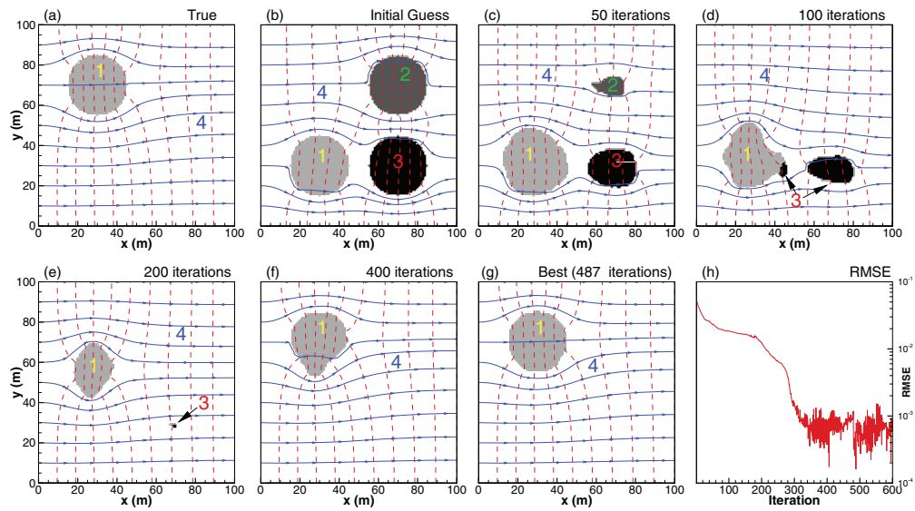
Figure 8: Evolution of lower permeable inclusions for Case 3, where the true field has one lower permeable material (a), but the guess field has three lower permeable materials because of lacking accurate information about the number of materials. Plots (b)-(f) illustrate some snapshots of the evolution, plot (g) is the best fit out of 600 iterations, and plot (h) shows the RMSE.
