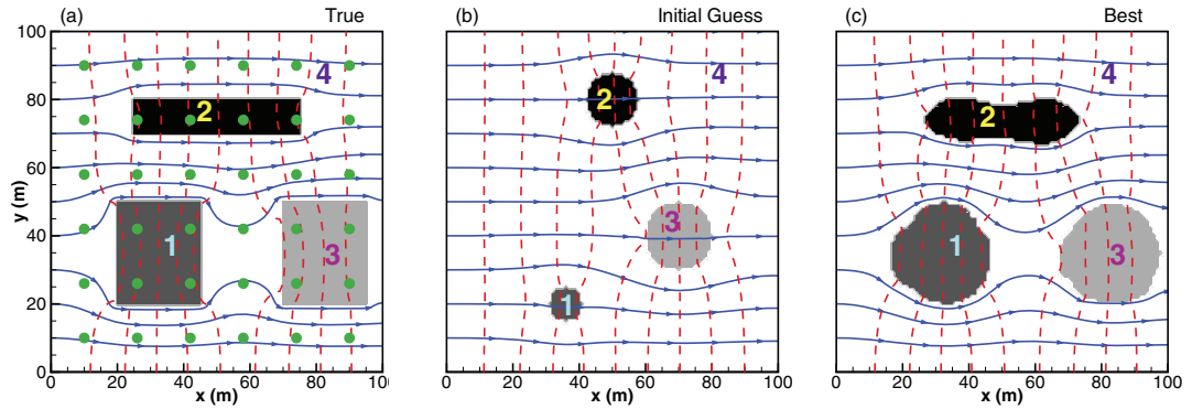
Figure 6: Comparison of (a) the true permeability field, (b) initial guess, and (c) the best inversion results in terms of the smallest RMSE in 700 iterations, for Case 2.
