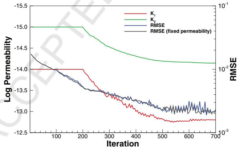
Figure 7: The permeability values and the root mean squared error (RMSE) as functions of the iteration number, Case 2.
