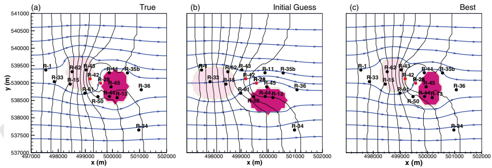
Figure 11: Comparison of (a) the true, (b) initial guess, and (c) the best results in terms of the minimum residual from 100 iterations, which has three materials. The contours and streamlines represent the flow field at 200 days.
