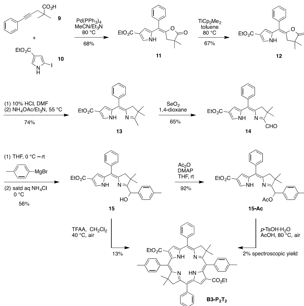
Scheme 6. Synthesis of a meso -tetraaryl bacteriochlorin ( B3-P 2 T 2 ).
