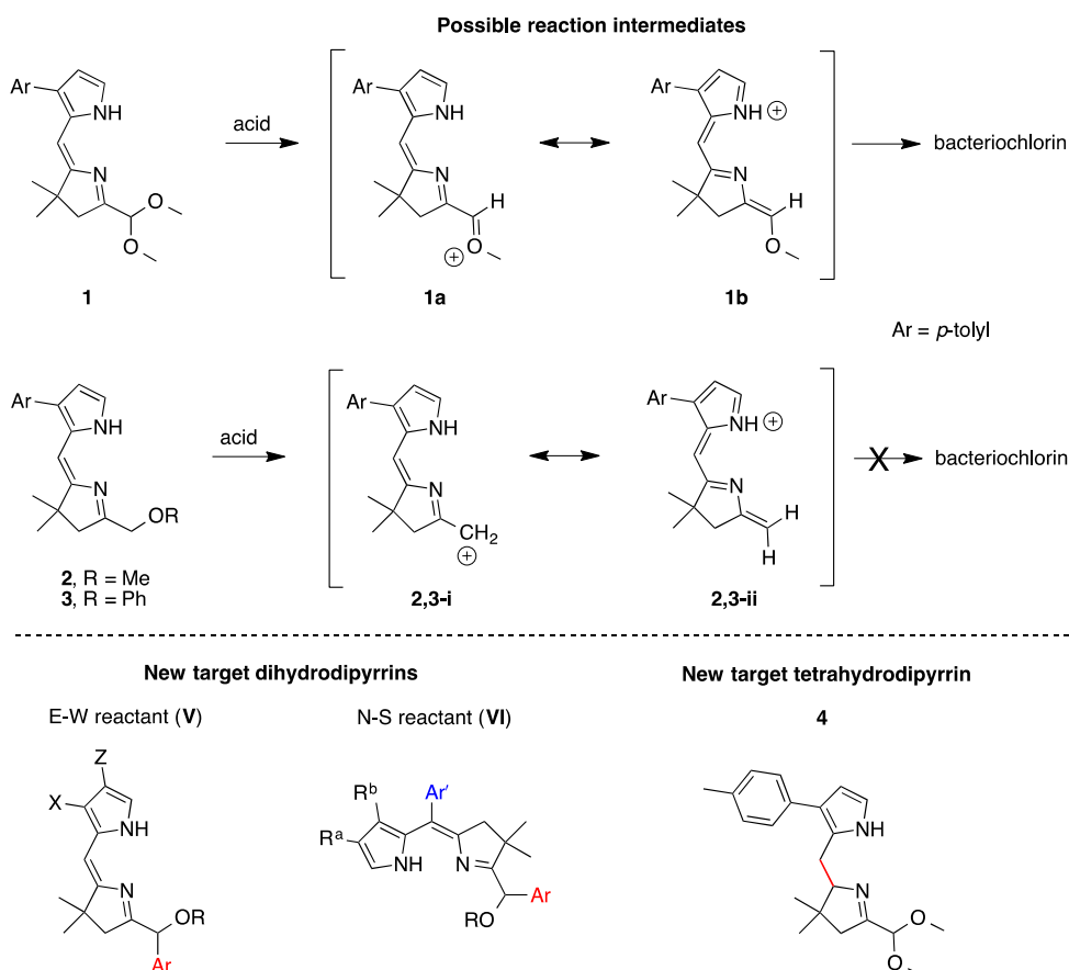
Scheme 2. Possible reaction intermediates for conversion of dihydrodipyrryn-acetal 1 or dihydrodipyrrens 2 or 3 to the bacteriochlorin ( top ) and new target hydrodipyrrens ( bottom ).
