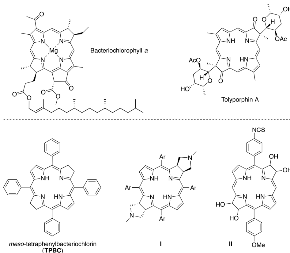
Figure 1. Bacteriochlorophyll a , tolyporphin A, and synthetic bacteriochlorins.
