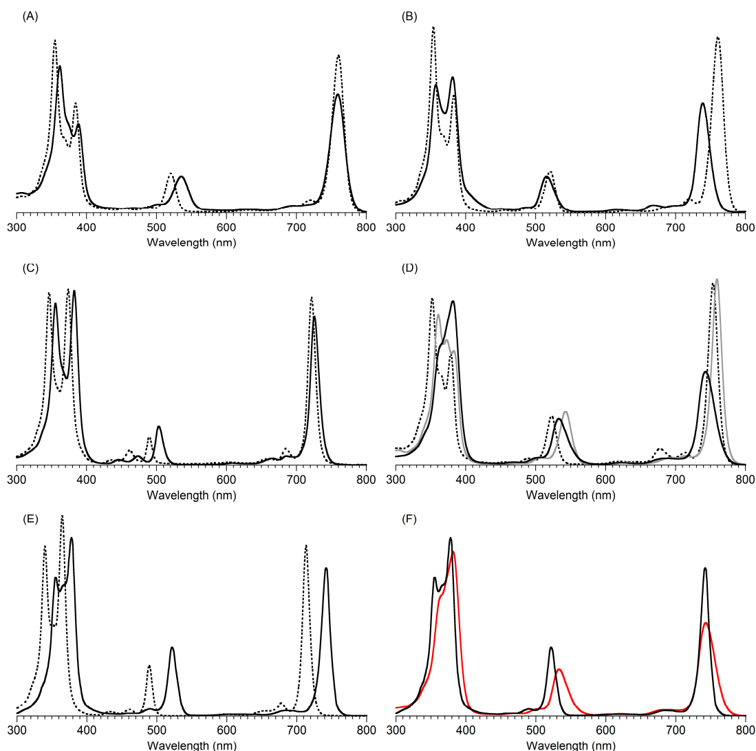
Figure 5. Absorption spectra of bacteriochlorins in toluene at room temperature. (A) iso -B2 (dotted) and iso -B2-T 2 (solid); (B) B2 (dotted) and B2-T 2 (solid); (C) B1 (dotted) and B1-T 2 (solid); (D) B3 (dotted), B3-T 2 (grey), and B3-P 2 T 2 (solid); (E) B6 (dotted) and TPBC (solid); (F) TPBC (black, reprised from panel E) and B3-P 2 T 2 (red, reprised from panel D).
