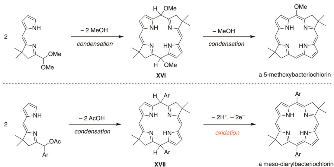
Scheme 11. Oxidation is required in the reaction of a dihydropyrrin-acetate ( lower panel) but not a dihydropyrrin-acetal ( upper panel). (Substituents have been omitted for clarity.)
