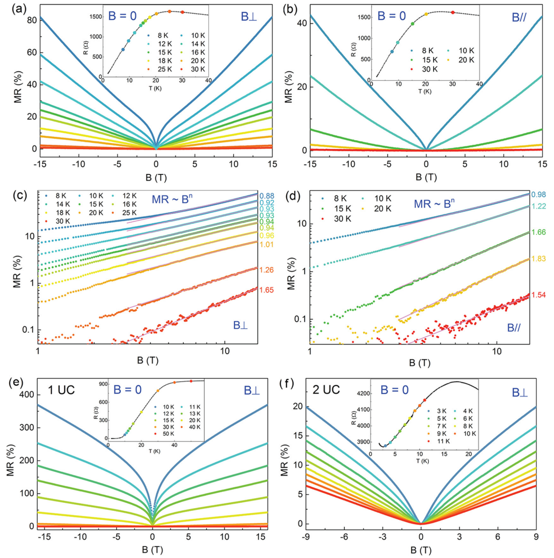
Figure 3. (a) and (b) MR as function of magnetic fields applied in perpendicular and parallel direction for another 3 UC FeSe film (S2). Insets: the temperature data points at which we measure the MR. (c) and (d) Demonstrate the MR as function of magnetic fields at different temperatures in double-logarithmic plot in perpendicular and parallel direction, respectively. (e) and (f) Demonstrate the magnetic field dependence of MR for 1 UC FeSe film and 2 UC FeSe film, respectively. Insets: the temperature data points at which we measure the MR.
