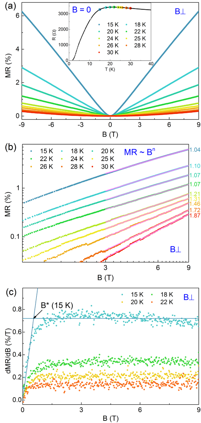
Figure 2. (a) Magnetic field dependence of MR for one 3 UC FeSe film (S1) at different temperatures. The inset labels the corresponding temperature data points at which we measure the MR by sweeping magnetic fields. (b) A double-logarithmic plot of MR versus magnetic fields at different temperatures. The lines show the power-law fitting ( MR \sim B^n ) of each curve in double-logarithmic coordinates above 3 T. The power exponent n is shown at the right column. (c) The field derivative of MR at different temperatures. The linear-fitting solid lines show the crossover from semiclassical regime to the linear response region.
