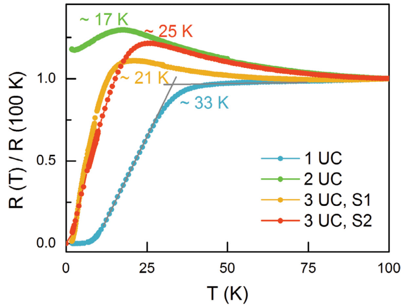
Figure 1. Temperature dependence of the resistance scaled by the values at 100 K under zero magnetic field for 1 UC, 2 UC and two 3 UC FeSe (S1 and S2) films grown on STO substrates. The values mark the T_c of the corresponding FeSe films.
