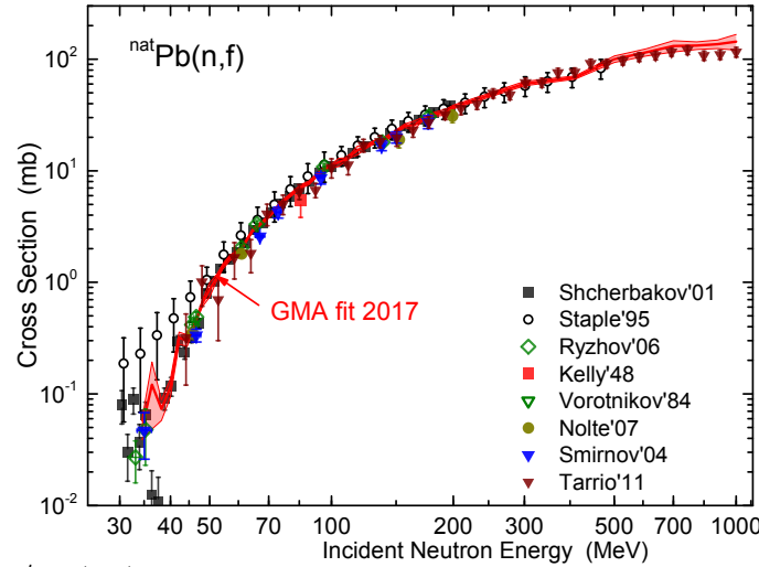
Figure 25: (Color online) ^{nat}\text{Pb}(n,f) cross section from threshold up to 1 GeV: known measurements selected for the GMA evaluation (symbols) and GMA fit 2017 with uncertainties (red curve).
