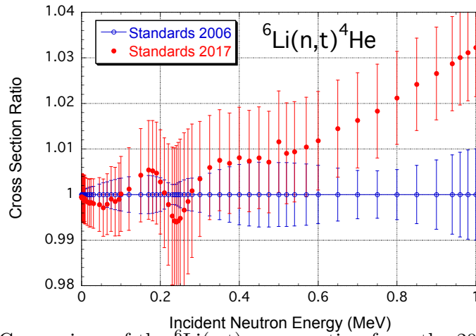
Figure 9: (Color online) Comparison of the {}^6\text{Li}(n,t) cross section from the 2017 evaluation with the 2006 standards evaluation. The baseline at 1.00 is the 2006 standards evaluation. At the highest energies the results are not within their uncertainties. The unrecognized systematic uncertainty of 0.5 % has been included in the 2017 data. It is possible that if the Parameter Confidence Interval and analysis of normalization for absolute measurements techniques had been available for the 2006 evaluation, those increased uncertainties would have provided agreement within uncertainties.
