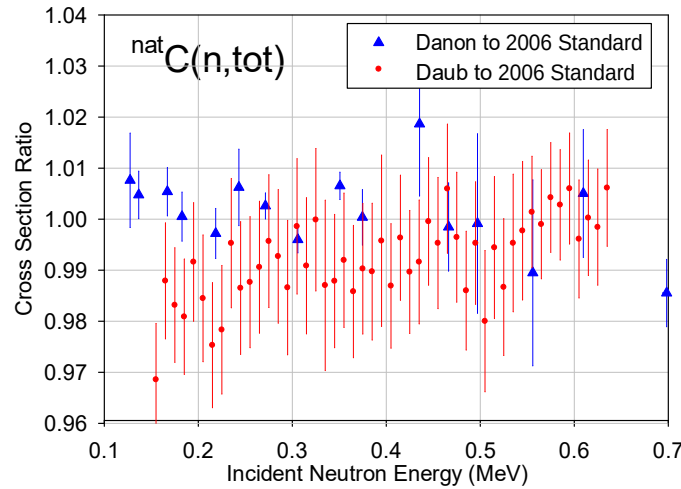
Figure 4: (Color online) Carbon total cross section of Danon et al. and Daub et al. compared with the 2006 standards evaluation.
