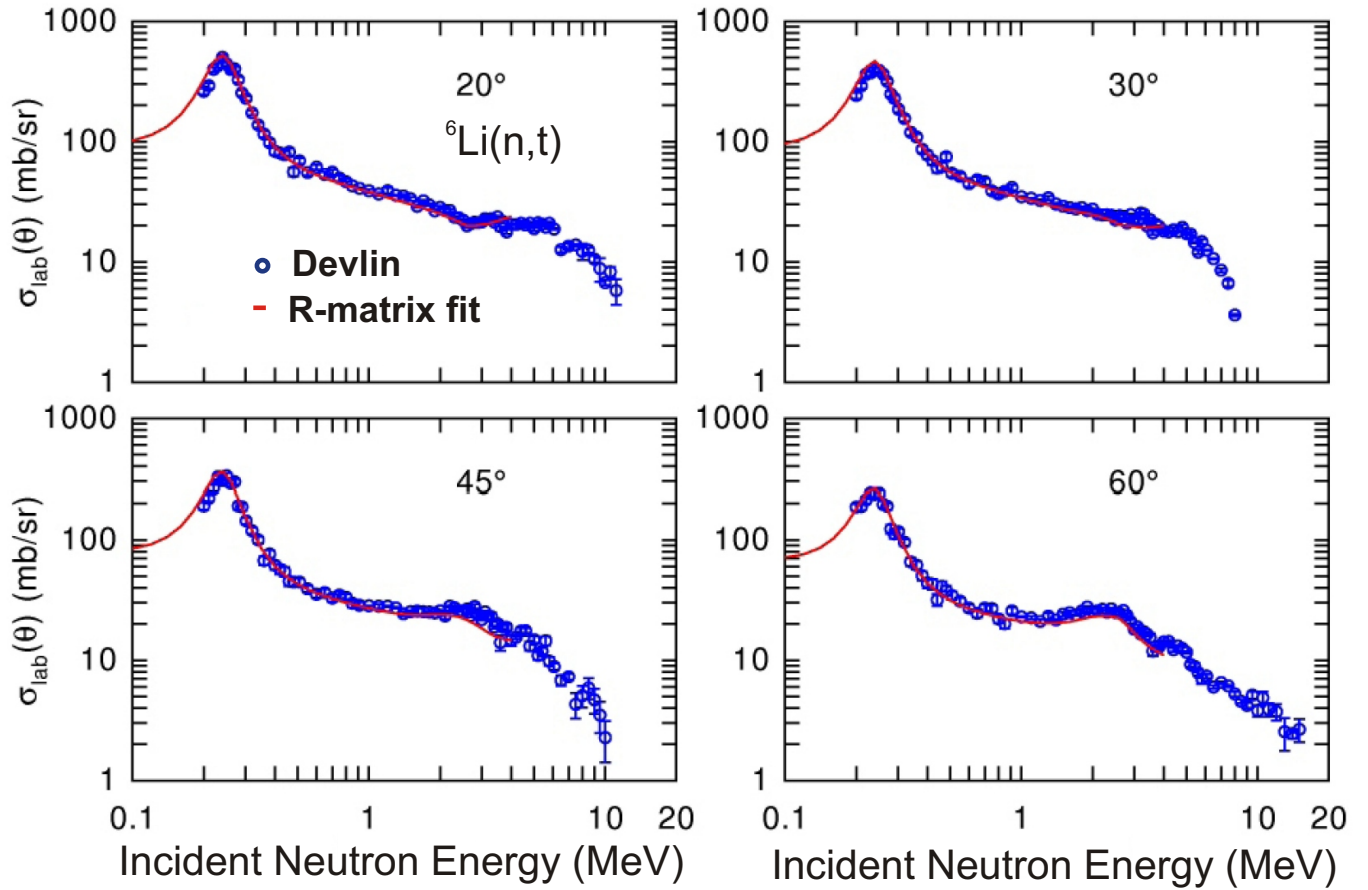
Figure 2: (Color online) Excitation functions measured by Devlin et al. for tritons from the {}^6\text{Li}(n,t) reaction for four angles compared with an R-matrix fit.
