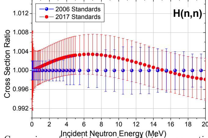
Figure 17: (Color online) Comparison of the total neutron elastic cross section of hydrogen for the 2017 evaluation with the 2006 standards evaluation. The unrecognized systematic uncertainty of 0.34 % has been included in the 2017 data.
