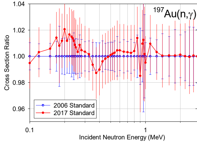
Figure 12: (Color online) Comparison of the \text{Au}(n, \gamma) cross section from the 2017 evaluation with the 2006 standards evaluation. The unrecognized systematic uncertainty of 1.7 % has been included in the 2017 data. The baseline at 1.00 is the 2006 standards evaluation.
