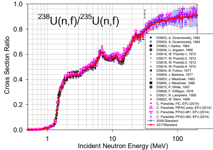
(f) ^{238}\text{U}(n,f) to ^{235}\text{U}(n,f) cross section ratio from 0.5–200 MeV.
