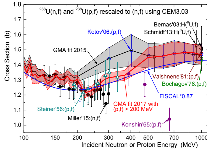
Figure 24: (Color online) ^{238}\text{U}(n,f) cross section from 100 MeV to 1 GeV. Symbols: recent measurement of Miller [50] and selected known (p,f) experiments above 200 MeV after rescaling to (n,f) using CEM3.03 model. Curves: GMA fit made in 2015 [90] (black) and current fit (red) with uncertainties; FISCAL parameterization scaled by factor 0.87 (blue). Note that we quote the results of the FISCAL parameterization by Fukahori et al. [94] as the JENDL-HE values from 300 to 1000 MeV.
