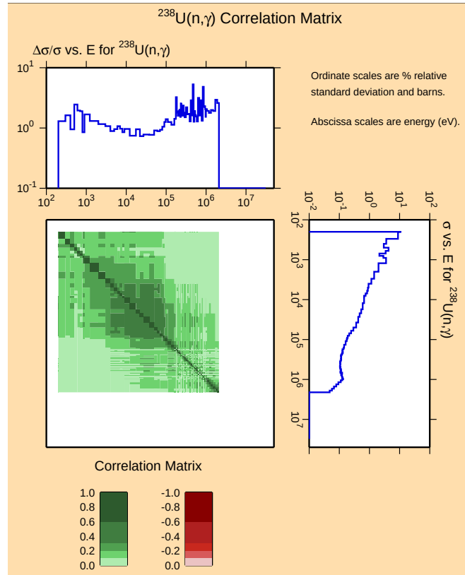
Figure 40: (Color online) Correlation matrix and relative uncertainties for the ^{238}\text{U}(n,\gamma) cross section.
