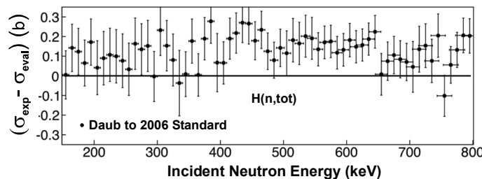
Figure 1: Comparison of the hydrogen total cross section measurements of Daub et al. with the 2006 standards evaluation.
