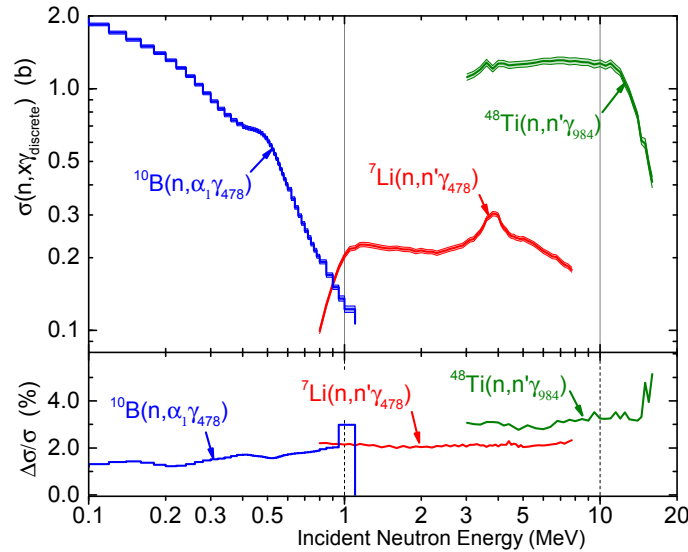
Figure 28: (Color online) Evaluated discrete \gamma -ray production cross sections for the ^{10}\text{B}(n, \alpha_1 \gamma) , ^7\text{Li}(n, n' \gamma) and ^{48}\text{Ti}(n, n' \gamma) reactions in the neutron energy ranges where they are recommended to use as references (top) and their uncertainties (bottom).
