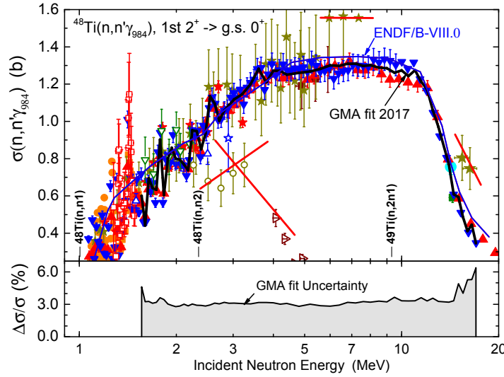
Figure 27: (Color online) ^{48}\text{Ti}(n,n'\gamma) reaction cross section in the neutron energy range 1–20 MeV. Top: existing and selected (except crossed) experimental (n,x\gamma) and (n,n_1) data (symbols); GMA fit 2017 (black curve) and ENDF/B-VIII.0 evaluation (blue). Bottom: uncertainty of the GMA fit.
