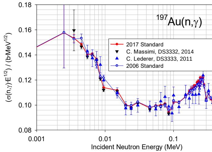
Figure 29: (Color online) Comparison of recent measurements and evaluations of the ^{197}\text{Au}(n,\gamma) cross section from 1 keV up to 400 keV.
