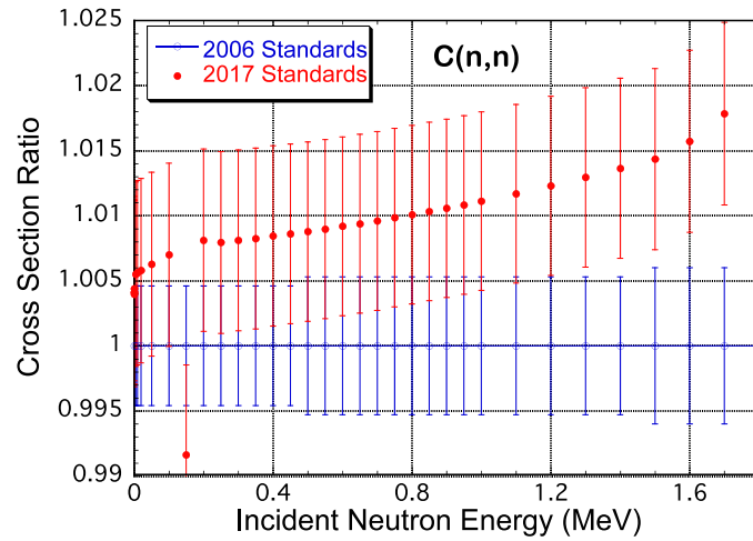
Figure 18: (Color online) Comparison of the carbon total elastic cross section for the 2017 evaluation with the 2006 standards evaluation. The unrecognized systematic uncertainty of 0.65 % has been included in the 2017 data. The baseline at 1.00 is the 2006 standards evaluation. The structures at about 0.15 MeV and 1.76 MeV are a result of changes in the evaluated ^{13}\text{C} total cross section.
