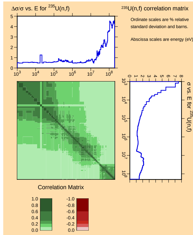
Figure 38: (Color online) Correlation matrix and relative uncertainties for the ^{235}\text{U}(n,f) cross section.
