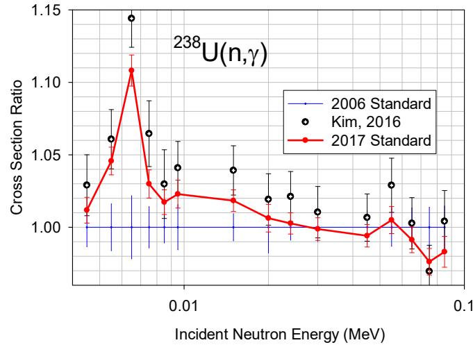
Figure 5: (Color online) Measurements of the ^{238}\text{U}(n,\gamma) cross section by Kim et al. compared with the results of the 2017 standards evaluation, relative to 2006 standards.
