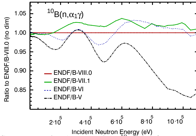
Figure 21: (Color online) Comparison of evaluations of the {}^{10}\text{B}(n,\alpha_1\gamma) cross section. In the standards energy region, the ENDF/B-VII.1 and ENDF/B-VIII.0 evaluations are the 2006 and 2017 {}^{10}\text{B}(n,\alpha_1\gamma) cross section standards, respectively.
