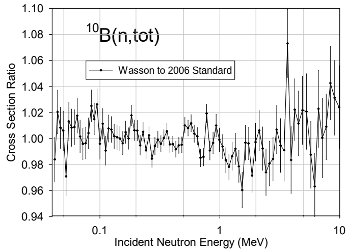
Figure 3: Measurements of the {}^{10}\text{B} total neutron cross section by Wasson et al. compared with the 2006 standard.
