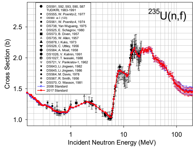
(b) Second group of ^{235}\text{U}(n,f) experimental data from 0.1–200 MeV.
