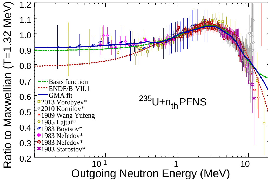
Figure 23: (Color online) Comparison of the measurements of ^{235}\text{U} PFNS measurements with the 2017 evaluation (GMA fit) and the ENDF/B-VII.1 evaluation. Above 10 MeV the 2017 evaluation follows the “basis function” which is a Maxwellian with temperature fitted to reproduce the evaluated ^{90}\text{Zr}(n,2n) SACS and Maxwellian normalization fixed by a continuity requirement at 10 MeV.
