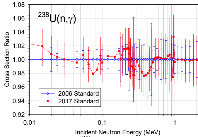
Figure 15: (Color online) Comparison of the ^{238}\text{U}(n,\gamma) cross section from the 2017 evaluation with the 2006 evaluation resulting from the standards evaluation. The unrecognized systematic uncertainty has been included in the 2017 data. That uncertainty is 1.7 % below 1 MeV and 2.4 % at 1 MeV and above. The baseline at 1.00 is the 2006 standards evaluation.
