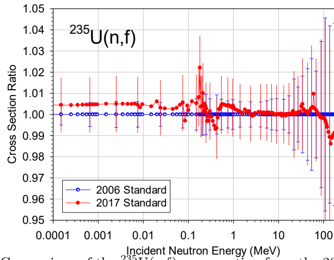
Figure 13: (Color online) Comparison of the ^{235}\text{U}(n,f) cross section from the 2017 evaluation with the 2006 standards evaluation. The results from 1 keV up to 150 keV correspond to the average of low resolution experiments. The unrecognized systematic uncertainty of 1.2 % has been included in the 2017 data. The baseline at 1.00 is the 2006 standards evaluation.
