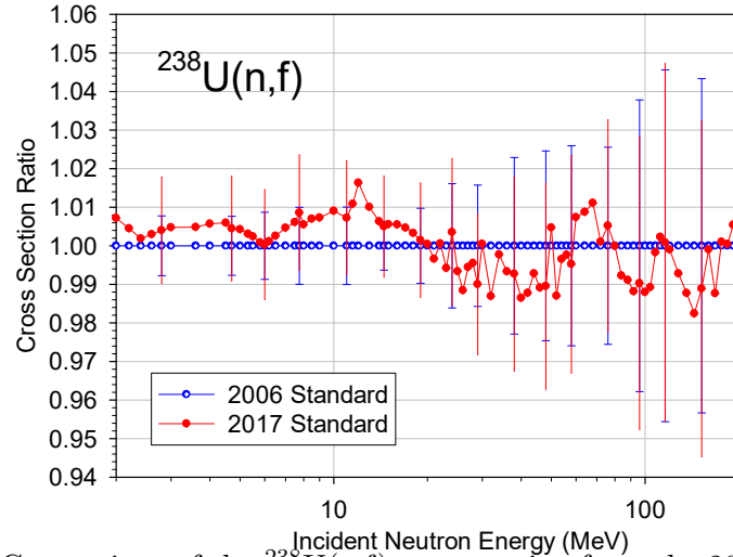
Figure 14: (Color online) Comparison of the ^{238}\text{U}(n,f) cross section from the 2017 evaluation with the 2006 standards evaluation. The unrecognized systematic uncertainty of 1.2 % has been included in the 2017 data. The baseline at 1.00 is the 2006 standards evaluation.
