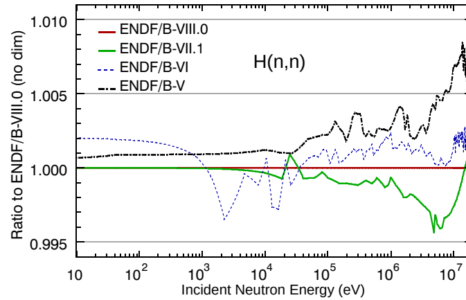
Figure 19: (Color online) Comparison of evaluations of the hydrogen total elastic cross section. In the standards energy region, the ENDF/B-VII.1 and ENDF/B-VIII.0 evaluations are the 2006 and 2017 \text{H}(n,n) cross section standards, respectively.
