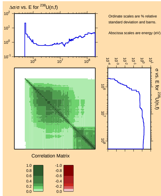
Figure 39: (Color online) Correlation matrix and relative uncertainties for the ^{238}\text{U}(n,f) cross section.
