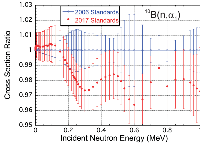
Figure 11: (Color online) Comparison of the ^{10}\text{B}(n, \alpha_1 \gamma) cross section from the 2017 evaluation with the 2006 standards evaluation. The unrecognized systematic uncertainty of 0.8 % has been included in the 2017 data. The baseline at 1.00 is the 2006 standards evaluation.
