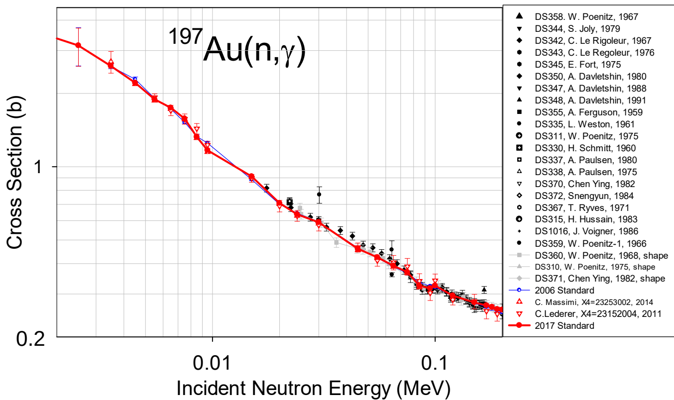
Figure 33: (Color online) Comparison of the 2017 and 2006 standards evaluations, together with experimental data for the \text{Au}(n,\gamma) cross section.
