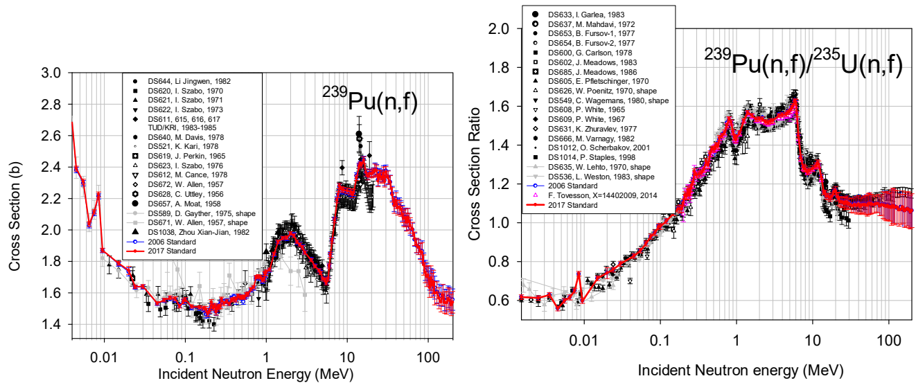
(a) ^{239}\text{Pu}(n,f) experimental data from 4 keV up to 200 MeV. (b) ^{239}\text{Pu}(n,f) to ^{235}\text{U}(n,f) cross section ratio from 1 keV up to 200 MeV.
