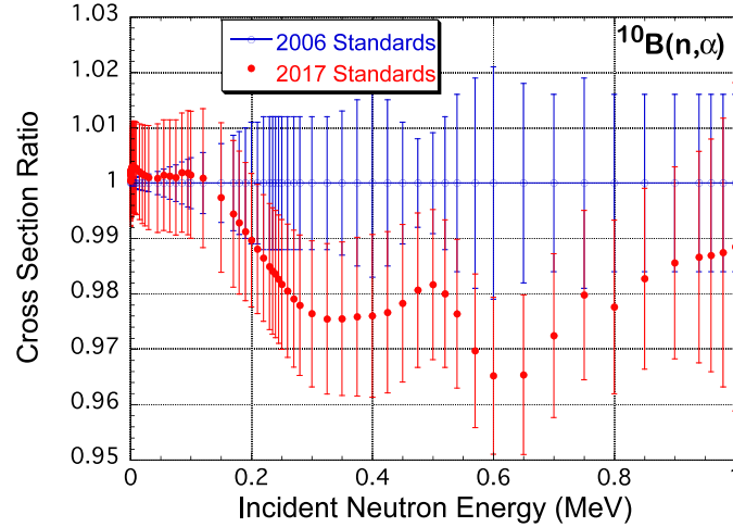
Figure 10: (Color online) Comparison of the {}^{10}\text{B}(n,\alpha) cross section from the 2017 evaluation with the 2006 standards evaluation. The unrecognized systematic uncertainty of 0.8 % has been included in the 2017 data. The baseline at 1.00 is the 2006 standards evaluation.
