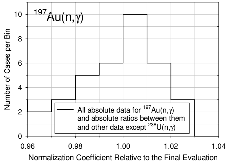
Figure 8: Histogram as a function of deviation from unity for normalization coefficients of \text{Au}(n,\gamma) absolute cross section and absolute cross section ratio measurements with \text{Au}(n,\gamma) except data with ^{238}\text{U}(n,\gamma) . The standard deviation is 1.7 % which is interpreted as unrecognized systematic uncertainty of neutron capture measurements on non-fissioning targets or actinides below the fission threshold.
