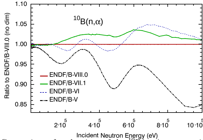
Figure 22: (Color online) Comparison of evaluations of the ^{10}\text{B}(n,\alpha) cross section. In the standards energy region, the ENDF/B-VII.1 and ENDF/B-VIII.0 evaluations are the 2006 and 2017 ^{10}\text{B}(n,\alpha) cross section standards, respectively.
