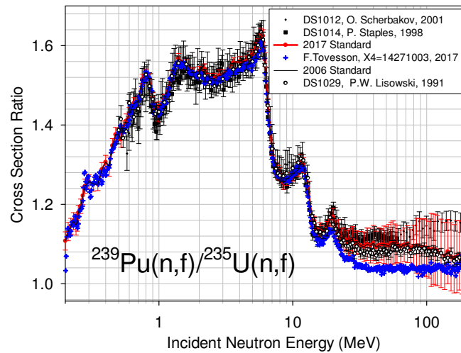
(c) ^{239}\text{Pu}(n,f) to ^{235}\text{U}(n,f) cross section ratio from 200 keV up to 200 MeV.
