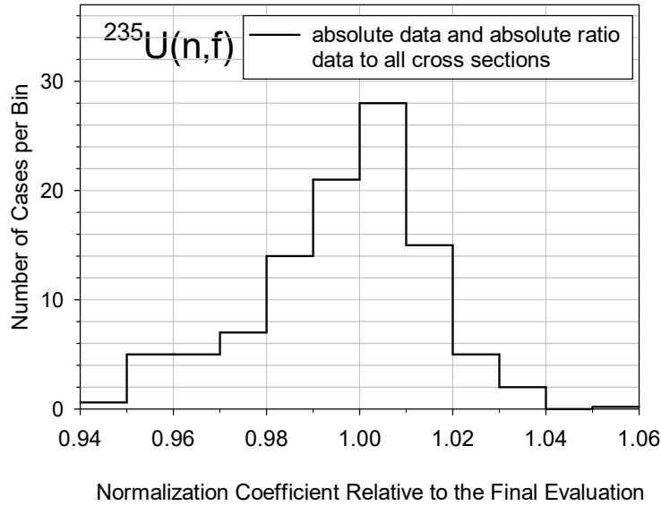
Figure 7: Histogram as a function of deviation from unity for normalization coefficients of ^{235}\text{U}(n,f) absolute fission cross section and fission cross section ratio measurements. The standard deviation is 1.2 % which is interpreted as unrecognized systematic uncertainty that corresponds to all fission measurements of actinides that use fission chambers.
