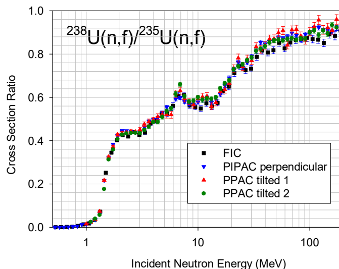
Figure 6: (Color online) Measurements of the ^{238}\text{U}(n,f)/^{235}\text{U}(n,f) cross section ratio by Paradela et al.
