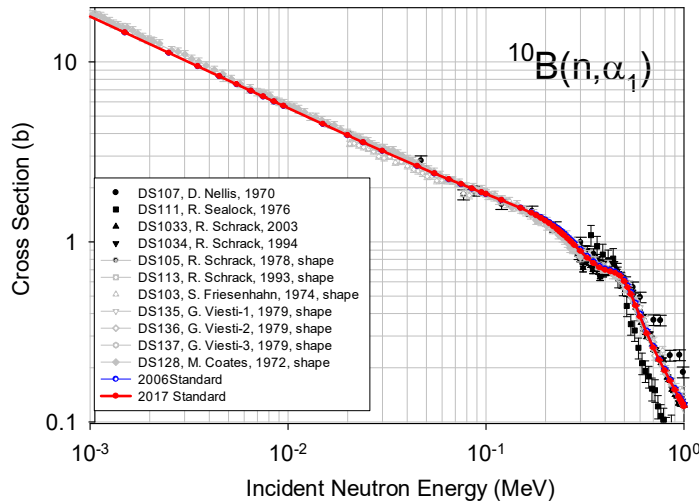
Figure 30: (Color online) Comparison of the 2017 and 2006 standards evaluations, together with experimental data for the ^{10}\text{B}(n,\alpha_1\gamma) cross section for energies from 1 keV to 1 MeV.
