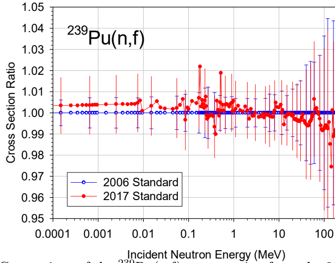
Figure 16: (Color online) Comparison of the ^{239}\text{Pu}(n,f) cross section from the 2017 evaluation with the 2006 evaluation resulting from the standards evaluation. The unrecognized systematic uncertainty of 1.2 % has been included in the 2017 data. The baseline at 1.00 is the 2006 standards evaluation.
