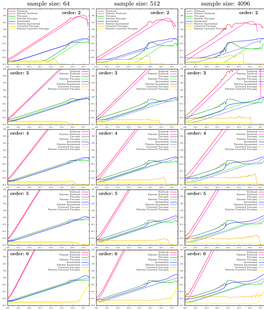
Fig. 4.2 The relative error (ordinate) in moments of orders 2 through 6 averaged over 2^{16} samples of size 64 (left), 512 (center), and 4096 (right) drawn from a noncentral exponential distribution with mean 1 and varying standard deviation (abscissa).
