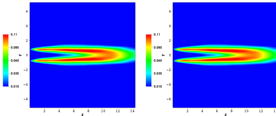
Fig. 4.3 Comparison of the compound second moment of \phi_f extracted from turbulent combustion DNS data. Left: moment extracted using the single-pass algorithm. Right: moment extracted using the naive two-pass algorithm.
