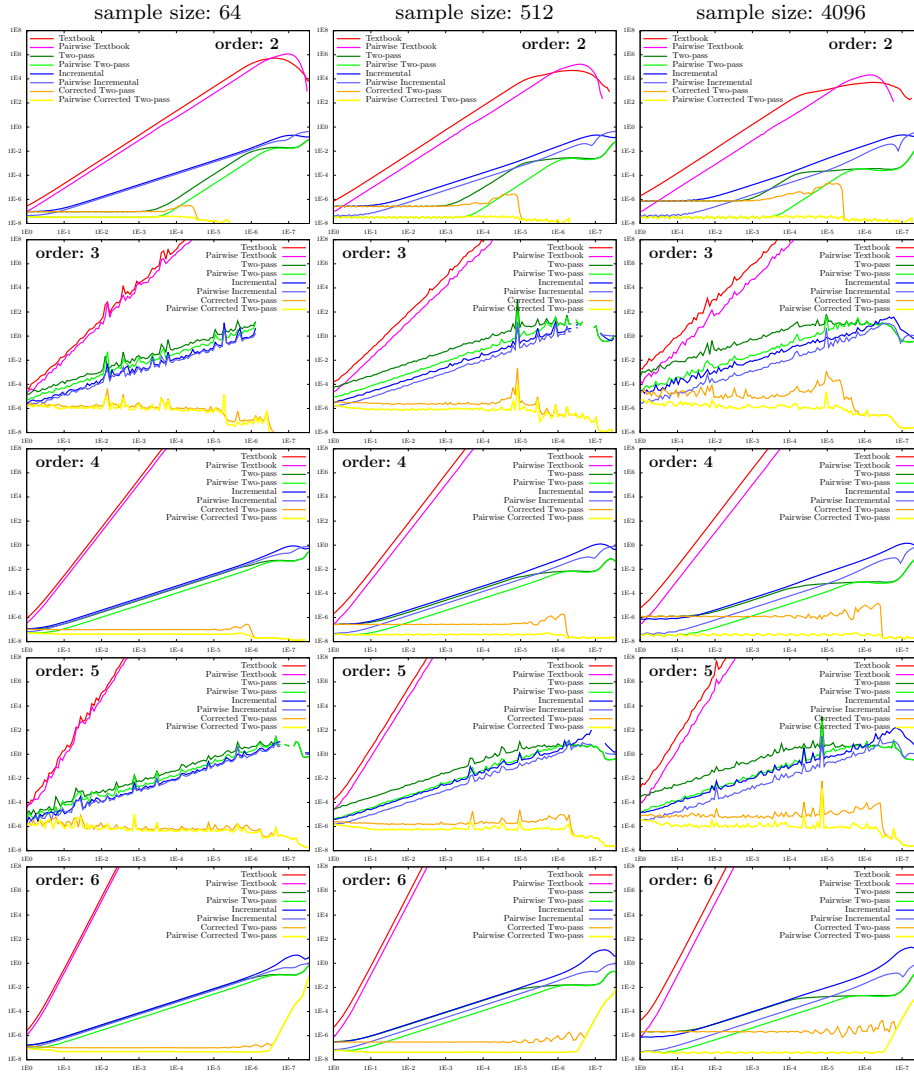
Fig. 4.1 The relative error (ordinate) in moments of orders 2 through 6 averaged over 2^{16} samples of size 64 (left), 512 (center), and 4096 (right) drawn from a Gaussian distribution with mean 1 and varying standard deviation (abscissa).
