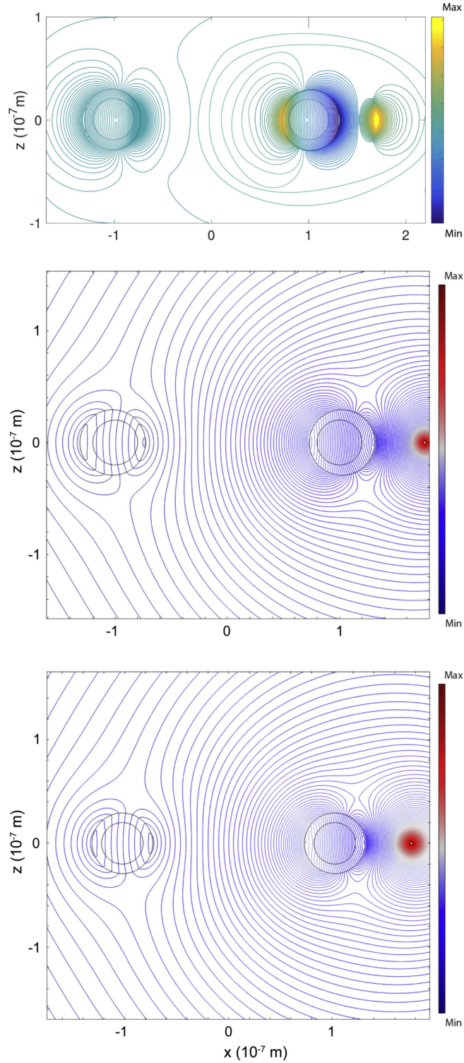
Figure 2. Potential distribution representing the response of a composite nanoring with a = 0.0980 \mu\text{m} , \cosh \mu_1 = 5 , \cosh \mu_2 = 3.5 , \epsilon_1 = -1.5 , \epsilon_2 = -3 , and \epsilon_3 = 1 to a non-uniform field of an electric monopole. (Top) The result is obtained via equation (74) with s = 1 by summation of poloidal and toroidal modes for a coated ring. Computationally determined distribution using FEM for confocal (Middle) versus concentric (Bottom) rings. Max (Min) signifies the highest (lowest) potential.
