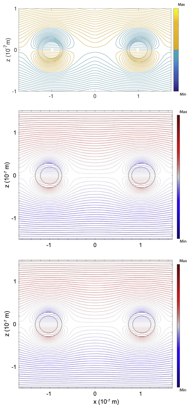
Figure 5. Potential distribution representing the response of a composite metal nanoring with similar parameters as in figure 2 to a uniform field polarized parallel to the ring symmetry axis. (Top) The result is obtained via equation (41) with m = 0 . Computationally determined distribution using FEM for confocal (Middle) versus concentric (Bottom) rings. Max (Min) signifies the highest (lowest) potential.
