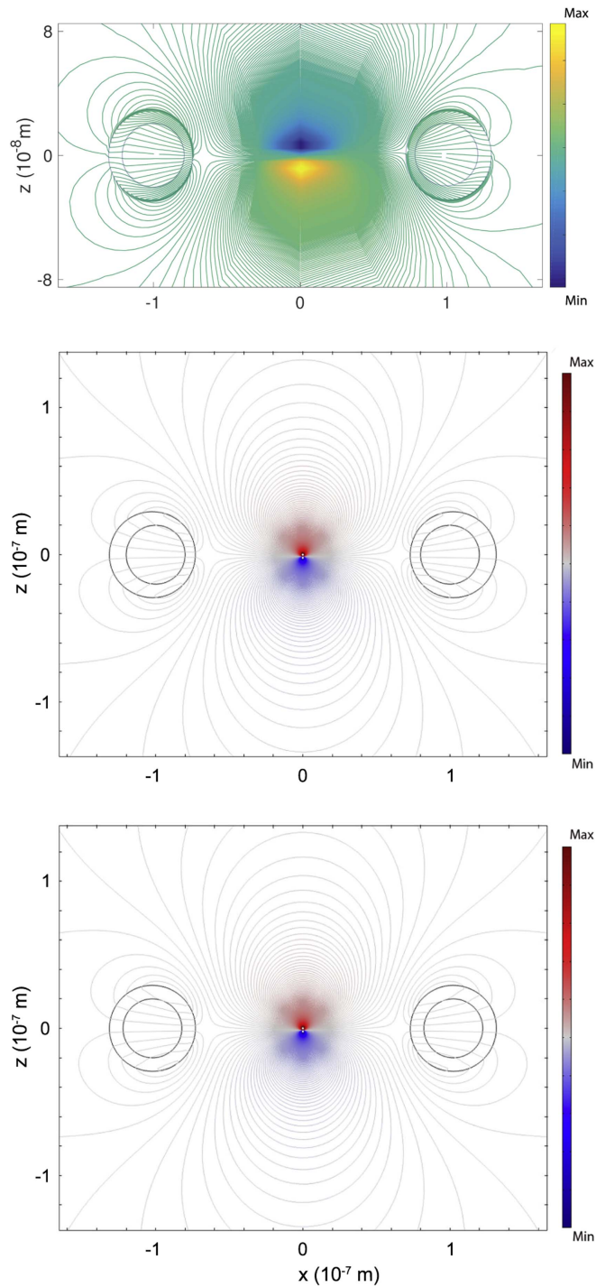
Figure 4. Potential distribution representing the response of a composite nanoring with similar parameters as in figure 2 to a non-uniform field of a dipole emitter located near the origin. ( Top ) The result is obtained via equation (74) with s = 1, 2 by summation of poloidal and toroidal modes for a composite ring. Computationally determined distribution using FEM for confocal ( Middle ) versus concentric ( Bottom ) rings. Max (Min) signifies the highest (lowest) potential.
