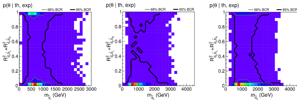
Figure 11. Resulting correlations between the sbottom flavour content and the masses of the three lightest down-type squarks after imposing all experimental constraints mentioned in table 3. Red colour indicates the highest and dark purple the lowest likelihood.
