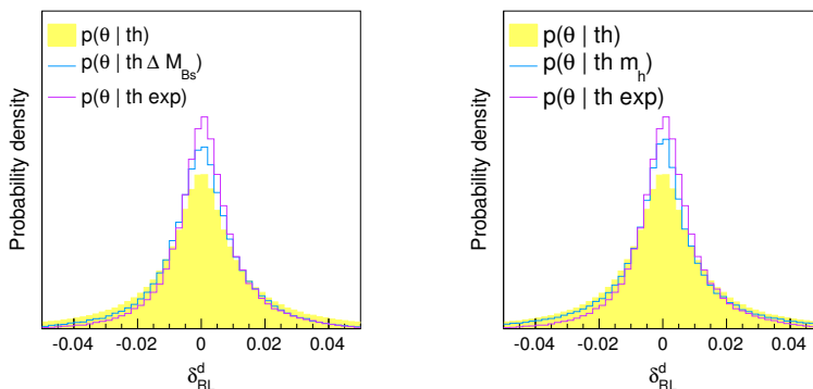
Figure 5. Most relevant observables constraining the \delta_{RL}^d parameter.
