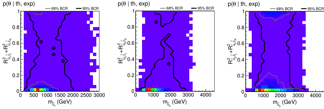
Figure 9. Resulting correlations between the stop flavour content and the masses of the three lightest up-type squarks after imposing all experimental constraints mentioned in table 3. Red colour indicates the highest and dark purple the lowest likelihood.
