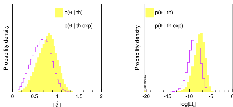
Figure 6. The one-dimensional prior (yellow histogram) and posterior (violet curve) distributions of the quantities |\vec{\delta}| and \log|\Pi_\delta| defined in eq. (4.4).
