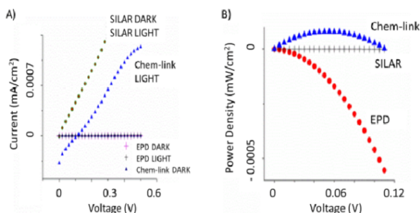
Figure 16. Typical current density (A) and power density (B) responses from nine replicates of photovoltaic devices containing TiO _2 nanotubes, indium-tin oxide deposited via electrochemical assistance and PbS quantum dots deposited using successive ion layer adsorption and reaction (SILAR), electrophoretic deposition (EPD) or chemical linking (Chem link)
