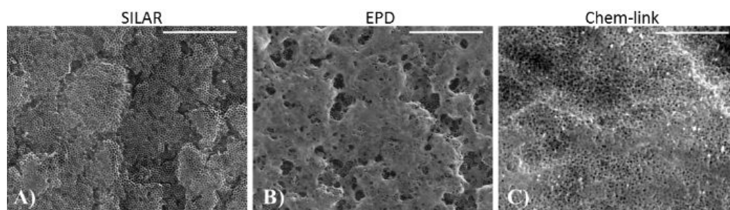
Figure 20. (Scale bar: 3 µm) Plan-view scanning electron microscopy micrographs of nanotube arrays sensitized with PbS quantum dots using either successive ion layer adsorption and reaction (A), electrophoretic deposition (B) or chemical linking (C)
