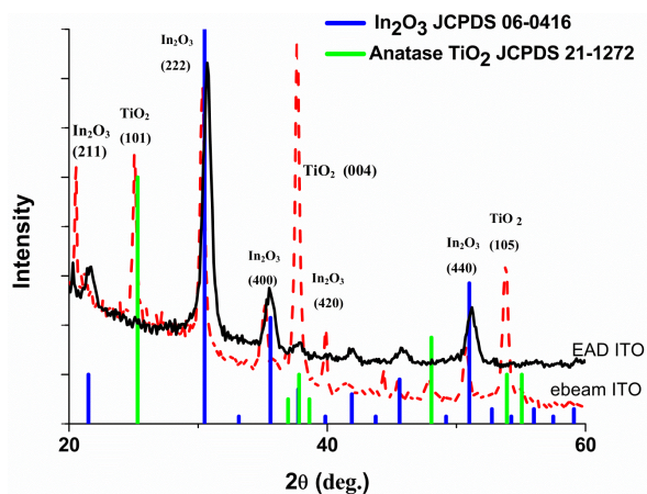
Figure 15. Glancing angle x-ray diffraction patterns of photovoltaic devices containing annealed TiO _2 nanotubes, PbS quantum dots, and indium-tin oxide deposited using either electrochemically assisted deposition (EAD) or electron beam evaporation (ebeam)
