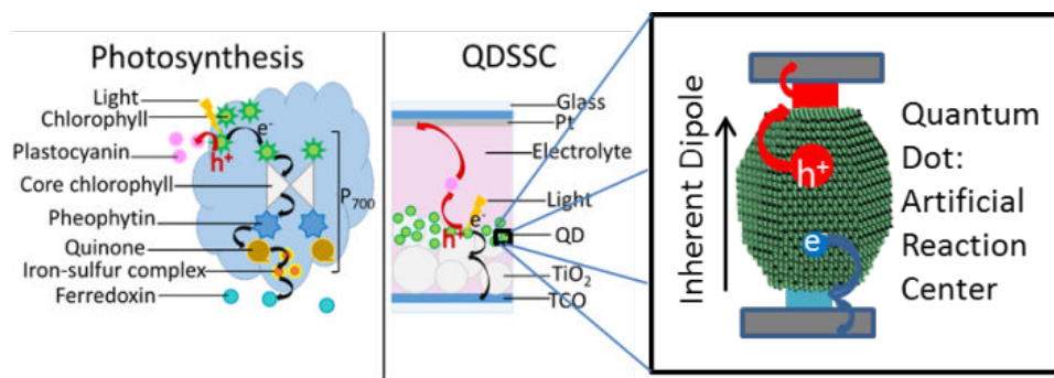
Figure 1. Comparison of charge generation and migration during photosynthesis in the P 700 reaction centre of photosystem I and during photoexcitation in a quantum dot, which acts as an artificial reaction centre in a quantum dot-sensitized solar cell (QDSSC)
