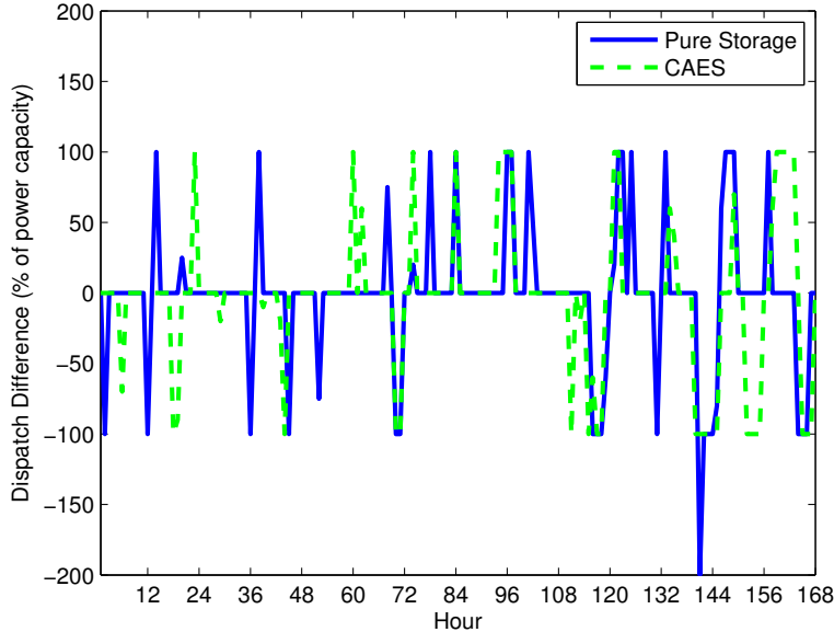
Figure 9: Difference in hourly net energy sales of pure storage and CAES between two consecutive weeks, as a percentage of power capacity.
