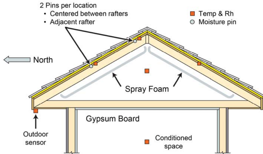
Figure 2: Cross-Section of sealed attic showing placement of thermistors, relative humidity sensors and moisture pins in demonstration homes.
