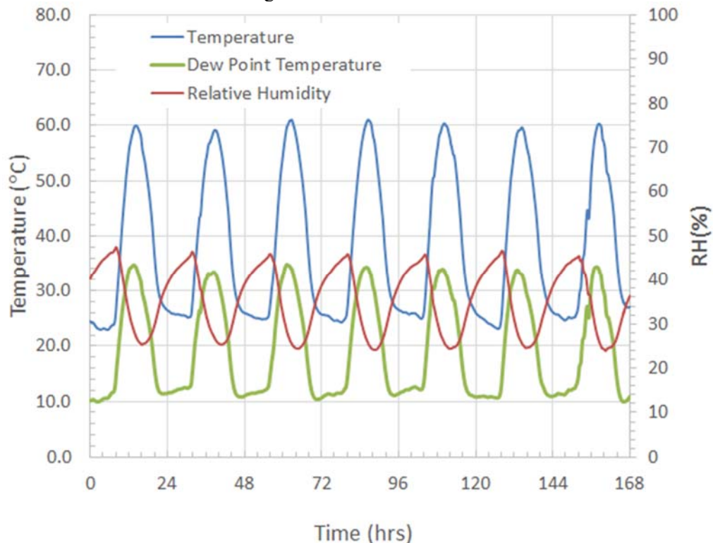
Figure 6: Sheathing temperature and relative humidity measured between the spray foam and the underside of the sheathing for the north-facing roof deck in West Palm Beach, FL
