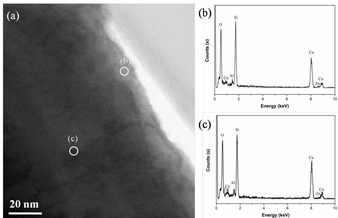
Figure 12. TEM image of the fresh Zn/ZSM-5 catalyst (a) and the corresponding EDX spectra at spot (b) and (c) selected in (a)
