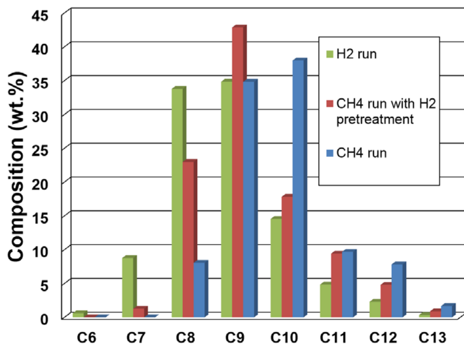
Figure 3. The carbon number distribution in the aromatics portion of the liquid product collected over 1%Ag/ZSM-5 with and without H 2 pretreatment at 400 °C under CH 4 and H 2 environments
