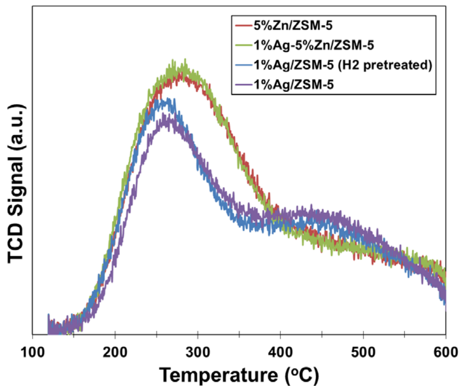
Figure 14. The NH 3 -TPD profiles collected over different catalysts
