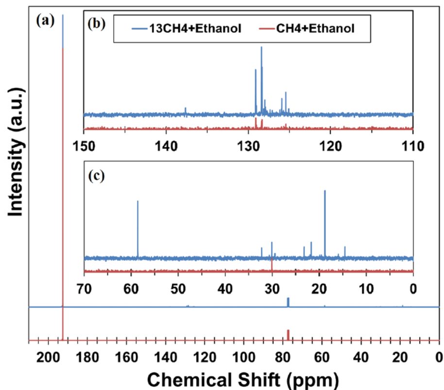
Figure 5. (a) The ^{13}\text{C} NMR spectra and its zoom-in views at chemical shift region of (b) 110~150 ppm and (c) 0~70 ppm of the liquid products collected from ethanol conversion under ^{13}\text{CH}_4 and \text{CH}_4 environments, respectively, at 400 °C and 1 atm
