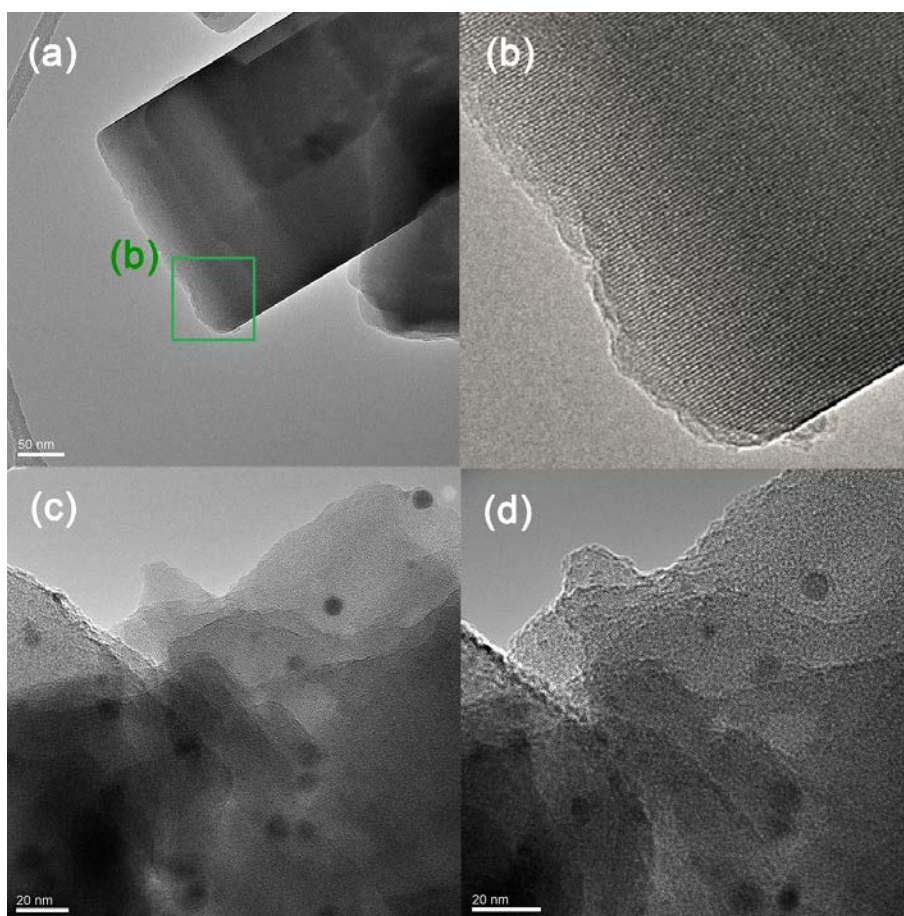
Figure 9. TEM Images of spent Ag/ZSM-5 catalyst (a) with ZSM-5 support focused, (b) zoom-in view of the squared area in (a), (c) and (d) with active metal focused at different resolutions
