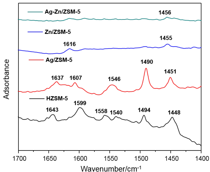
Figure 13. DRIFT spectra collected over HZSM-5, Ag/ZSM-5, Ag-Zn/ZSM-5, and Zn/ZSM-5 catalysts upon pyridine adsorption
