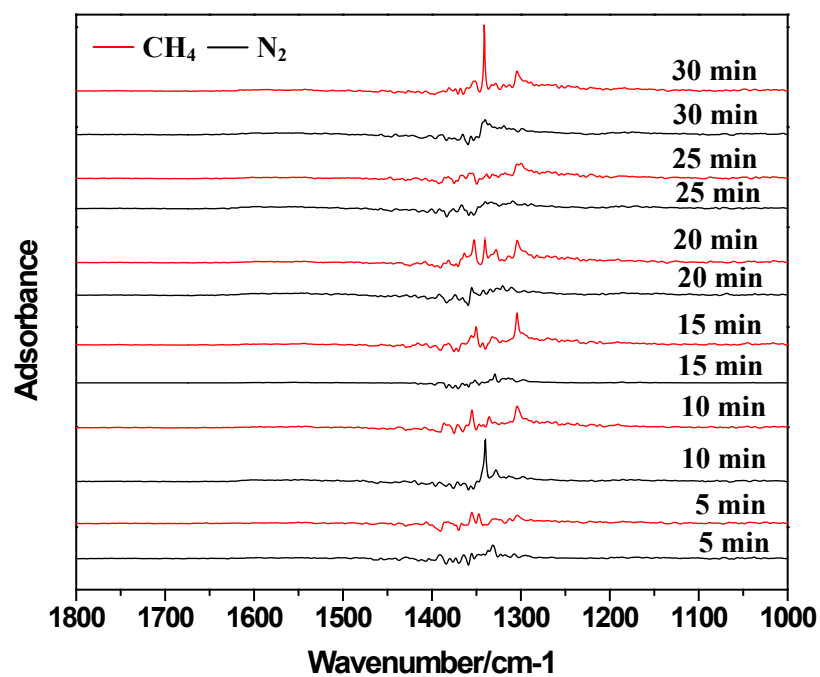
Figure 6. The DRIFT spectra collected at different time over 1%Ag/ZSM-5 during ethanol conversion under various environments at 400 °C and 1 atm
