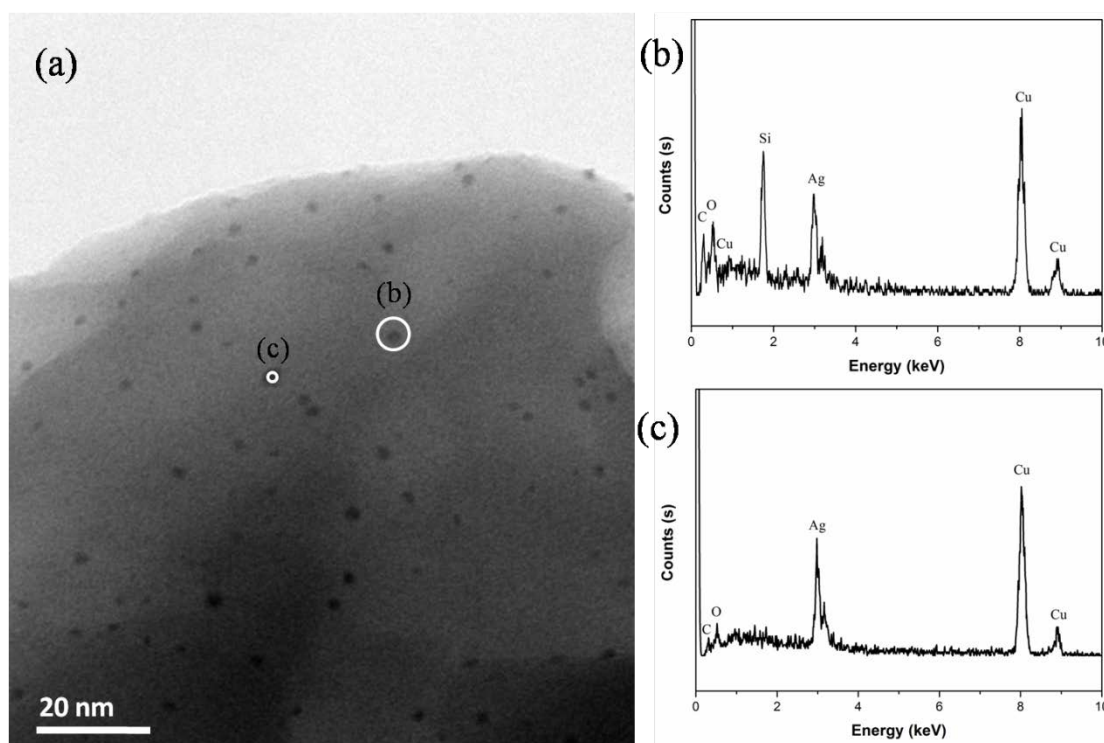
Figure 8. TEM image of the Ag/ZSM-5 catalyst (a) and the corresponding EDX spectra at spot (b) and (c) selected in (a)
