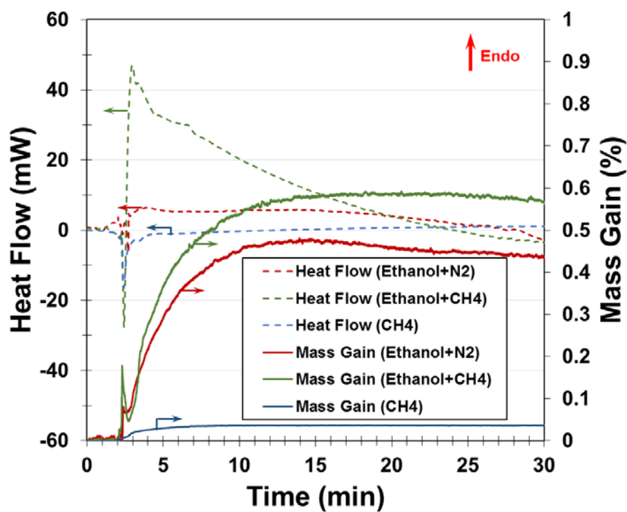
Figure 4. The TGA-DSC profiles collected over 1%Ag/ZSM-5 during ethanol aromatization under various environments and methane-alone run at 400 °C and 1 atm
