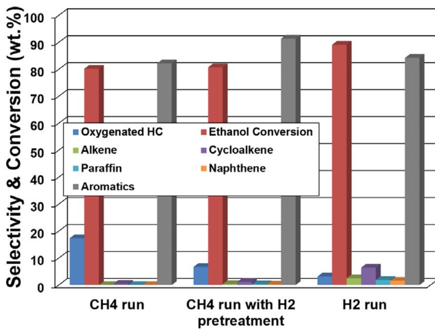
Figure 2. The ethanol conversion and liquid product selectivity from the runs over 1%Ag/ZSM-5 with and without H 2 pretreatment at 400 °C under CH 4 and H 2 environments
