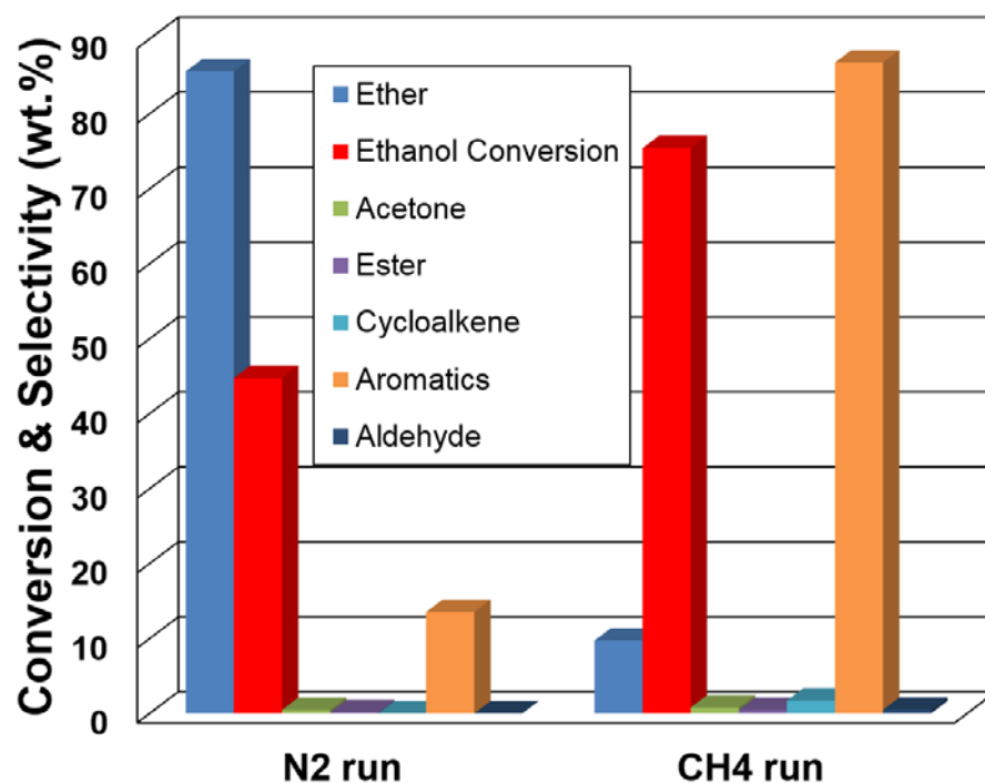
Figure 1. The ethanol conversion and liquid product selectivity from the runs over 1%Ag/ZSM-5 at 400 °C under N 2 and CH 4 environments
