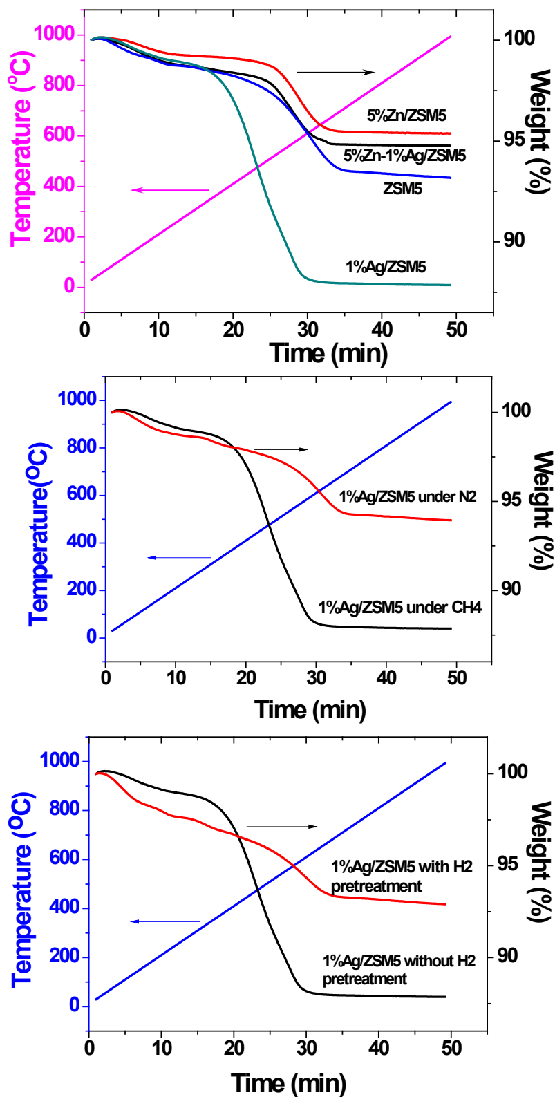
Figure 15. TGA profiles collected over (a) various spent catalysts and spent Ag/ZSM-5 (b) under different environments, and (c) with or without H 2 pretreatment under heating in air
