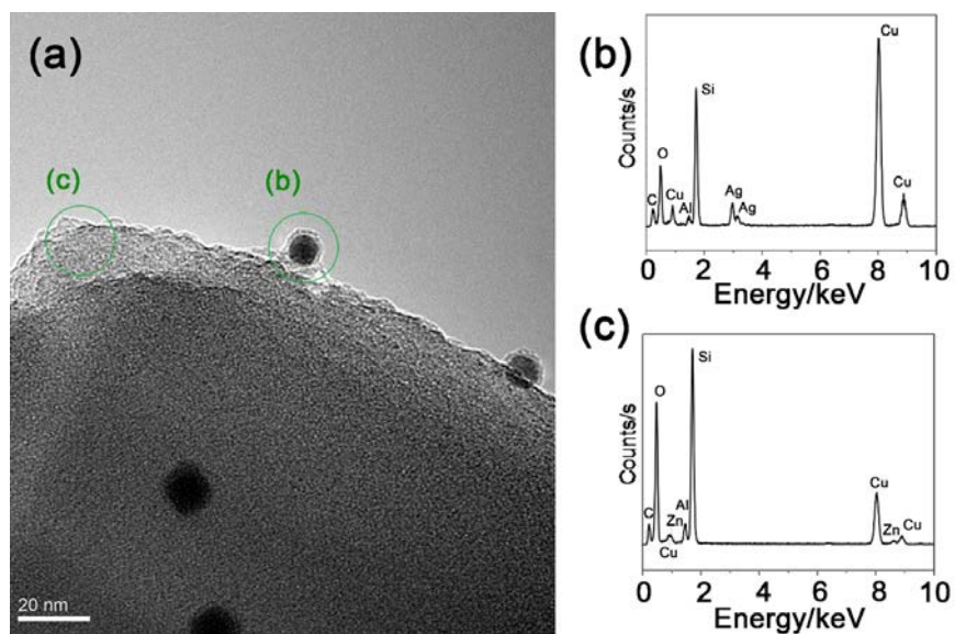
Figure 11. TEM Image of spent Ag-Zn/ZSM-5 catalyst (a) with active metal particles focused, and the corresponding EDX spectra at spots (b) and (c) selected in (a)
