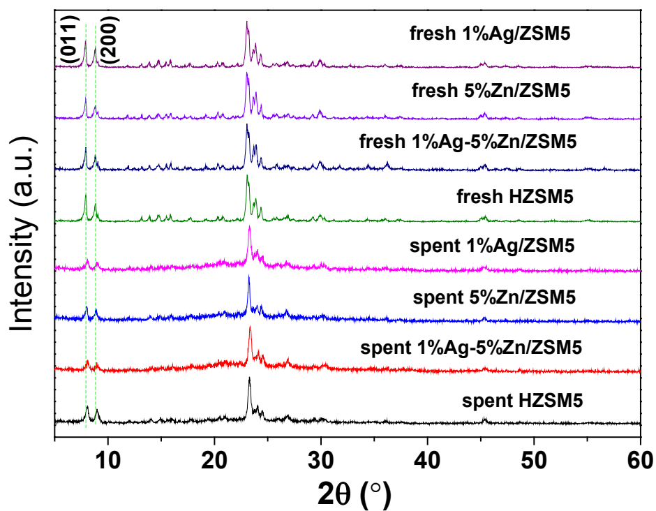
Figure 7. XRD patterns of fresh and spent HZSM-5, Zn/ZSM-5, Ag-Zn/ZSM-5, and Ag/ZSM-5 catalysts
