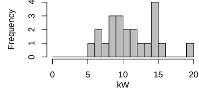
Fig. 5: Histogram of maximum power consumed, as recorded for 22 households in the U.K.
