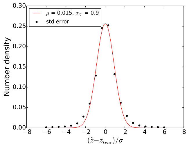
Figure A2. Photometric standardized error for the mode: The photometric standardized error computed from the mode of each individual galaxy’s photo- z PDF compared to the best fit Gaussian. As modes are defined by the peak of each PDF, the distribution tends to be more concentrated than the distribution of mean PDF values.
