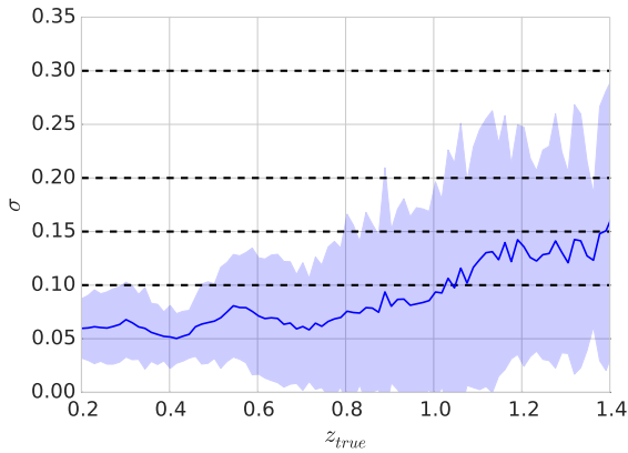
Figure 2. Dependence of the square root of the mean photo-z variance, given by \sigma^2 in Equation (1) for galaxies in small true redshift bins, on the true redshift. Standard deviations are given by the square root of the variance of the photo-z errors in each bin. Dashed lines correspond to the width of the different bin configurations treated in this paper, in order to compare the bin widths with the photo-z dispersion for the sample considered.
