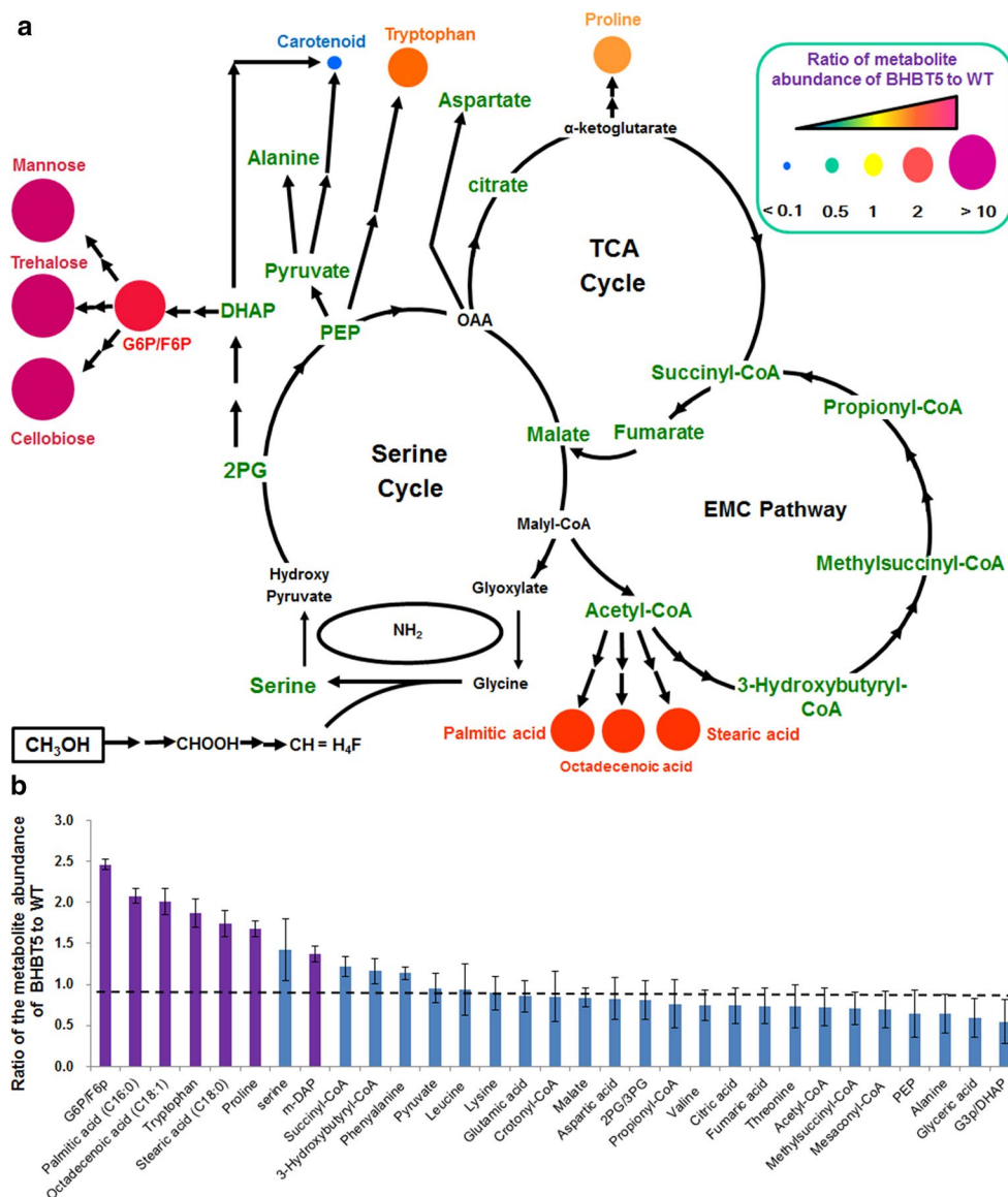
Fig. 5 Targeted metabolomic analysis of wild-type and BHBT5 strains. a Methylotrophic major metabolism in M. extorquens AM1 and metabolite change between BHBT5 and wild-type. The colored circle indicates significant difference ( p < 0.05 ). The metabolites without significant change are shown in green. Double arrows indicate multiple reactions. b The ratio of metabolite abundance of the BHBT5 strain to the wild-type strain. Note: myristic acid (C14:0) was not presented as it was only detected in the wild-type strain. Ratios outside the 1.0 \pm 0.2 range indicated significant difference of concentration ( p < 0.05 ) for each metabolite (purple). The data were presented as the mean plus STDEV calculated from triplicate biological replicates
