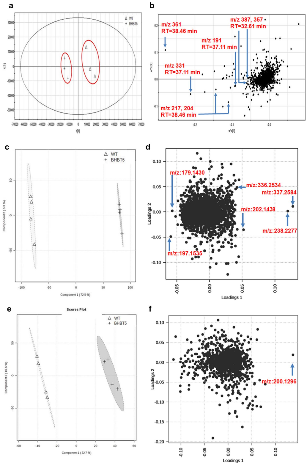
Fig. 6 Untargeted metabolomic analysis of wild-type and BHBTS strains. The metabolome data were processed by PLS-DA. a, b The score plot and loading plot of metabolome analyzed by GC-MS. c, d The score plot and loading plot of metabolome analyzed by LC-MS in the positive mode. e, f The score plot and loading plot of metabolome analyzed by LC-MS in the negative mode. The arrows point out the differential metabolites between the wild-type and BHBTS strains
