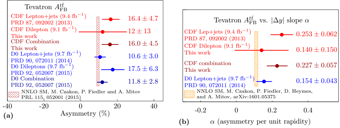
FIG. 14. Comparison of the combined inclusive A_{FB}^{t\bar{t}} and the slope \alpha of A_{FB}^{t\bar{t}} vs. |\Delta y| with all other Tevatron measurements and the NNLO SM calculations.
