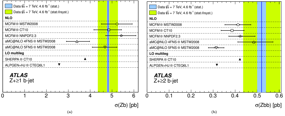
Figure 6. Cross-sections for (a) Z + \geq 1 b-jet, and (b) Z + \geq 2 b-jets. The measurement is shown as a vertical blue line with the inner blue shaded band showing the corresponding statistical uncertainty and the outer green shaded band showing the sum in quadrature of statistical and systematic uncertainties. Comparison is made to NLO predictions from MCFM interfaced to different PDF sets and aMC@NLO interfaced to the same PDF set in both the 4FNS and 5FNS. The statistical (inner bar) and total (outer bar) uncertainties are shown for these predictions, which are dominated by the theoretical scale uncertainty calculated as described in the text. Comparisons are also made to LO multi-legged predictions from ALPGEN+HERWIG+JIMMY and SHERPA; in this case the uncertainty bars are statistical only, and smaller than the marker.
