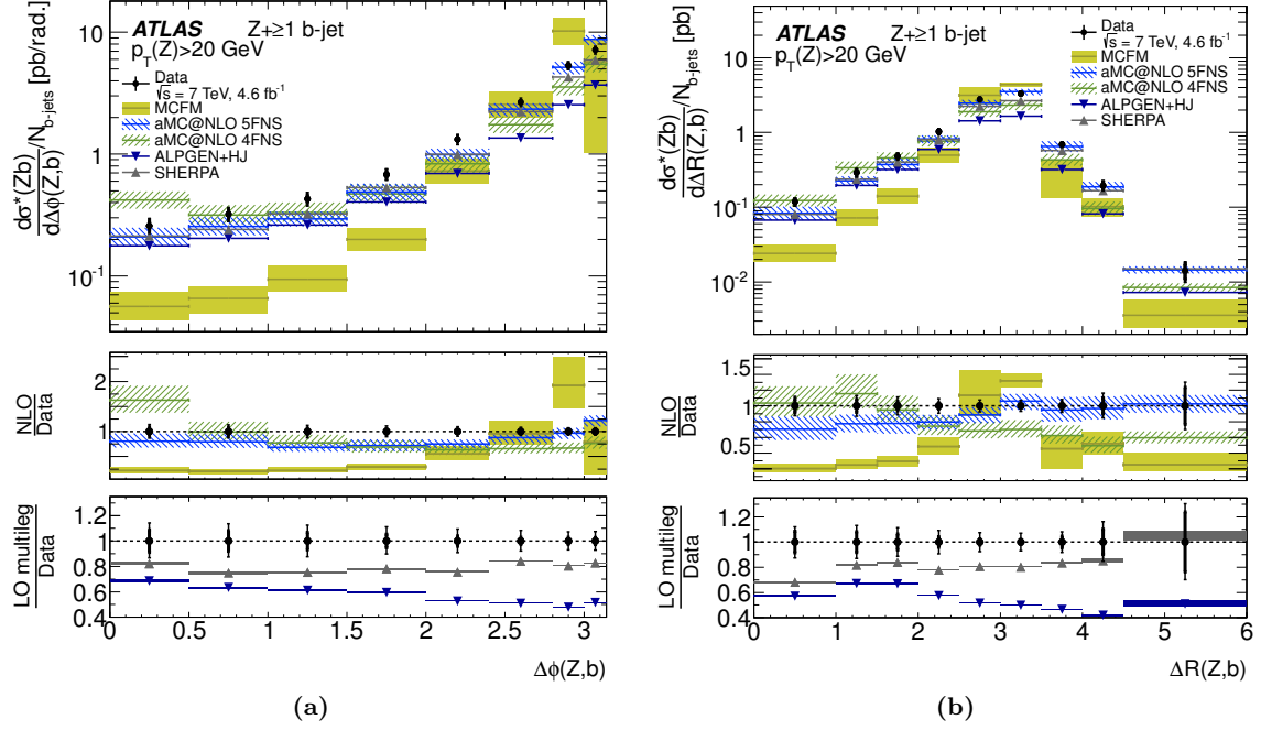
Figure 10. The inclusive b -jet cross-section \sigma^*(Zb) \times N_{b\text{-jet}} as a function of \Delta\phi(Z, b) (a) and \Delta R(Z, b) (b). The inclusive cross-section requires that the Z boson p_T be at least 20 GeV. The top panels show measured differential cross-sections as filled circles with statistical (inner) and total (outer bar) uncertainties. Overlaid for comparison are the NLO predictions from MCFM and aMC@NLO both using the MSTW2008 PDF set. The shaded bands represents the total theoretical uncertainty for MCFM and the uncertainty bands on aMC@NLO points represent the dominant theoretical scale uncertainty only. Also overlaid are LO multi-legged predictions for ALPGEN+HERWIG+JIMMY and SHERPA. The middle panels show the ratio of NLO predictions to data, and the lower panels show the ratio of LO predictions to data.
