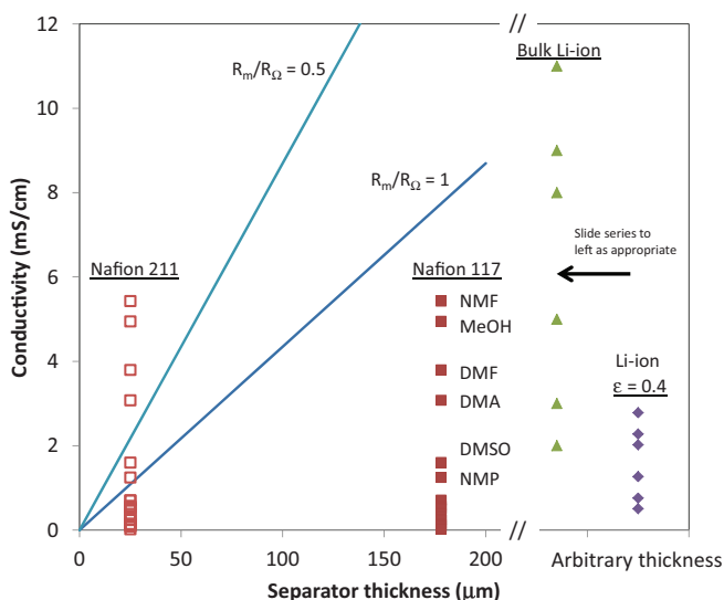
Figure 2. Relationship between conductivity and separator thickness for R_\Omega = 2.3 \Omega\cdot\text{cm}^2 . The lines follow the equation \kappa = l/R_m . The vertical series labeled Nafion were measured by Doyle et al. for lithium exchanged N117 imbibed with various solvents. 17 Filled squares are data for N117 and open squares are corrected to the thickness of Nafion 211, 25 \mu\text{m} . The vertical series labeled Li-ion are data taken from various literature sources for carbonate electrolytes for lithium-ion batteries. Triangles are bulk values and diamonds are corrected to a porosity of 40%, typical of lithium-ion battery separators. The lithium-ion data is plotted at an arbitrary thickness for the sake of presentation and can be moved to the left as appropriate.
