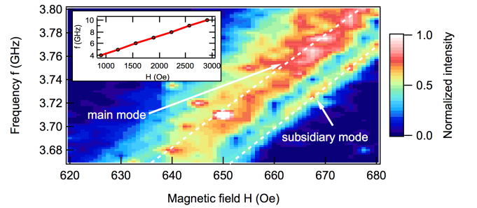
FIG. 3. Resonance frequency as a function of bias magnetic field measured by BLS illustrated in a color-coded image. The laser spot was focused onto the center of the sample while the rf frequency and magnetic field were varied. As for the electrical measurements two modes are detected by BLS. The inset shows corresponding field dependence of the resonance measured by electrical means.
