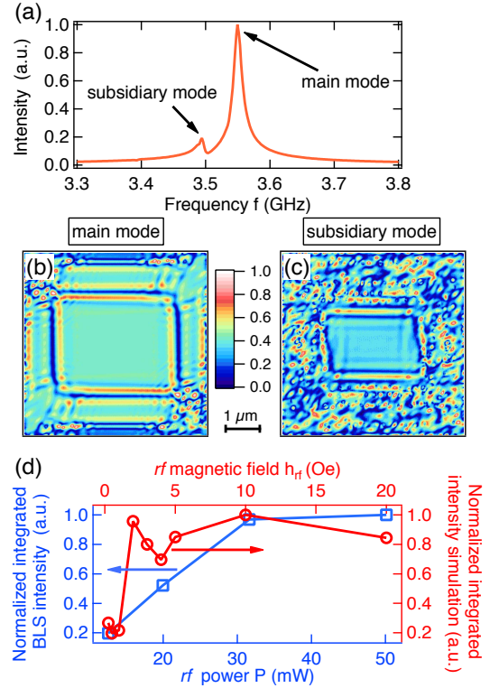
FIG. 5. Micromagnetic simulations: (a) The spectrum reveals two modes. Spatially-resolved magnetization distribution of the main mode, (b), and the less intense, subsidiary mode, (c). (d) The normalized integrated BLS intensity saturates at high excitation powers P , which is validated by micromagnetic simulations at large driving rf magnetic fields h_{rf} .
