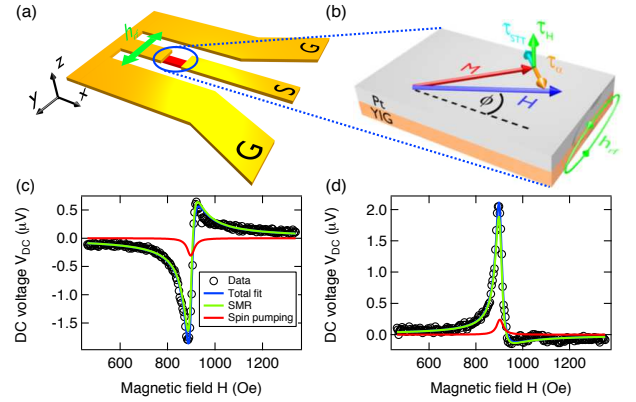
FIG. 1. (a) Schematic of the ST-FMR experimental setup (b) ST-FMR mechanism in the YIG/Pt bilayer. The alternating rf current drives an Oersted field h_{rf} exerting a field-like torque \tau_H on the magnetization M . At the same time a oscillatory transverse spin accumulation at the YIG/Pt interface is generated by the SHE which results in a damping-like torque \tau_{STT} . (c) and (d) Typical dc voltage spectra recorded at in-plane angles of \phi = 30^\circ and \phi = 240^\circ and P = +10 dBm.
