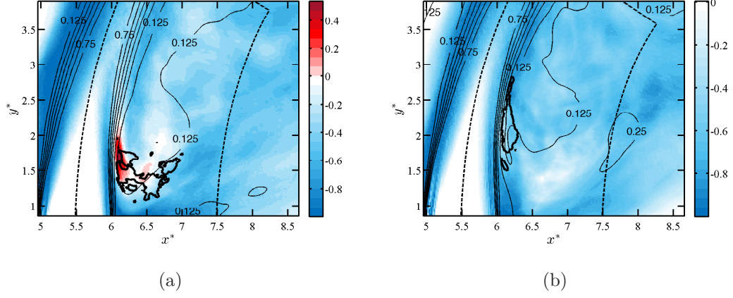
Figure 8: Iso-lines of mean velocity magnitude \|\tilde{\mathbf{u}}\|^* = 0.125, 0.25, \dots, 0.75 (thin solid line) and probable explosive zones p_{EZ}^o = 0.5 (bold solid line) overlaid on color iso-contours of the mean flame index \overline{\text{FI}} for the CO-lean (a) and the CO-rich (b) cases.
