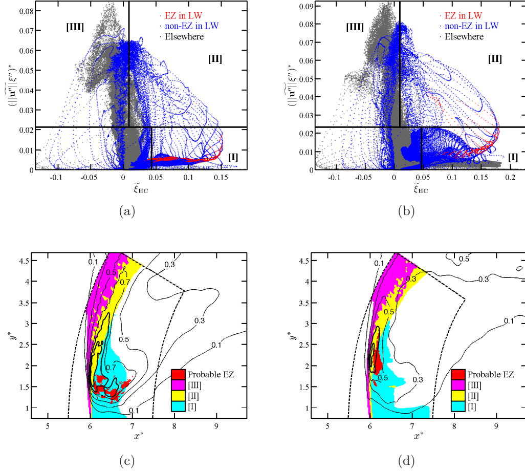
Figure 7: Variation of \widetilde{\|\mathbf{u}''\|\xi''}^* with \tilde{\xi}_{\text{HC}} with the classification of zones [1]–[3] (a, b), and a map showing these zones in the LW region in physical space (c, d) for the CO-lean (a, c) and the CO-rich (b, d) cases. In (a, b), red: samples taken from the probable EZ ( p_{EZ}^\circ > 0.5 ) in the LW sampling region, blue: non-EZ samples in the LW sampling region, and gray: other samples in entire domain. In (c, d), iso-lines of \overline{Q}^\circ = 0.1, 0.3, 0.5, 0.7 (thin lines), 0.8, 0.9 (bold line) for the CO-lean and \overline{Q}^\circ = 0.1, 0.3, 0.5 (thin lines), 0.7, 0.8 (bold line) for the CO-rich cases. Zone [I]: Large \tilde{\xi}_{\text{HC}}^\circ \geq 0.25 and negligible \widetilde{\|\mathbf{u}''\|\xi''}^\circ \leq 0.25 , zone [II]: \tilde{\xi}_{\text{HC}}^\circ \geq 0.05 and large \widetilde{\|\mathbf{u}''\|\xi''}^\circ > 0.25 , and zone [III]: negative or negligible \tilde{\xi}_{\text{HC}}^\circ < 0.05 and large \widetilde{\|\mathbf{u}''\|\xi''}^\circ \geq 0.25 .
