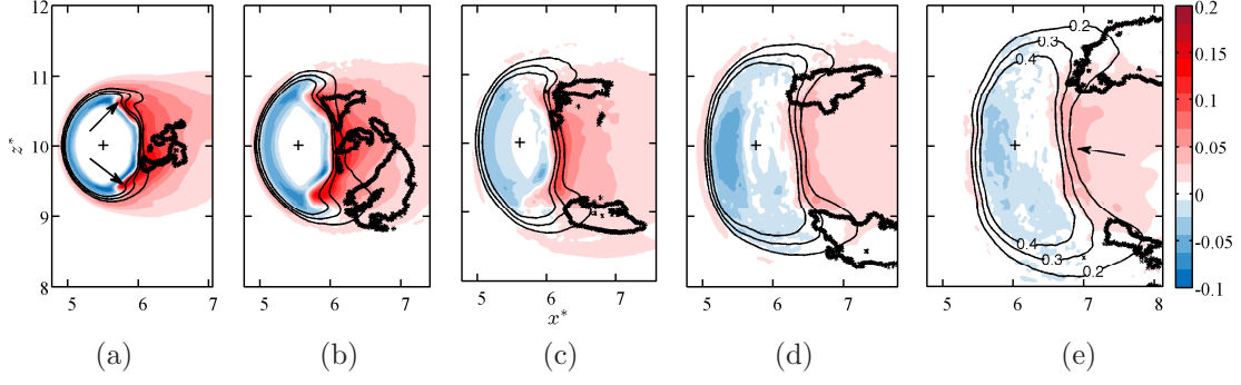
Figure 5: Mean mixture fraction iso-lines ( \tilde{\xi} = 0.2, 0.3, 0.4 ) overlaid on the differential diffusion elemental mixture fraction \tilde{\xi}_{HC} in the x - z slices at different y positions, (a) y^* = 1.20 , (b) y^* = 1.69 , (c) y^* = 2.20 , (d) y^* = 2.88 , (e) y^* = 3.75 , for the CO-lean case. Bold line shows explosive zones. The mean jet trajectory is also denoted by the + symbol.
