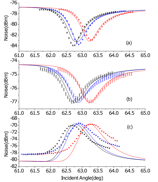
FIG. 2. (Color online) (a) Noise power of the single-channel coherent light source, (b) the noise power of the double-channel coherent light source and (c) the noise power of the squeezed light source. The simulated noise power is shown in solid lines calculated from the complex reflection coefficient shown in Eq. (1) and the relative intensity noise shown in Eq. (4). The black, blue and red lines correspond to the refractive index of 1.3, 1.301 and 1.305. In all cases, the uncertainty in the experimental data was \pm 0.1 dB statistical and systematic combined error.
