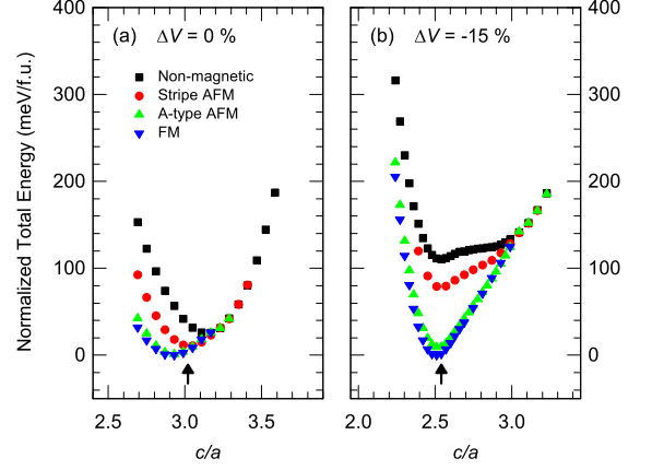
FIG. 5. (color online) The energy difference between magnetic states from total energy calculations for (a) the T phase ( \Delta V = 0\% ) and (b) the cT phase ( \Delta V = -15\% ). The measured values of \frac{c}{a} at ambient pressure and above 20 GPa are indicated by the black arrows.
