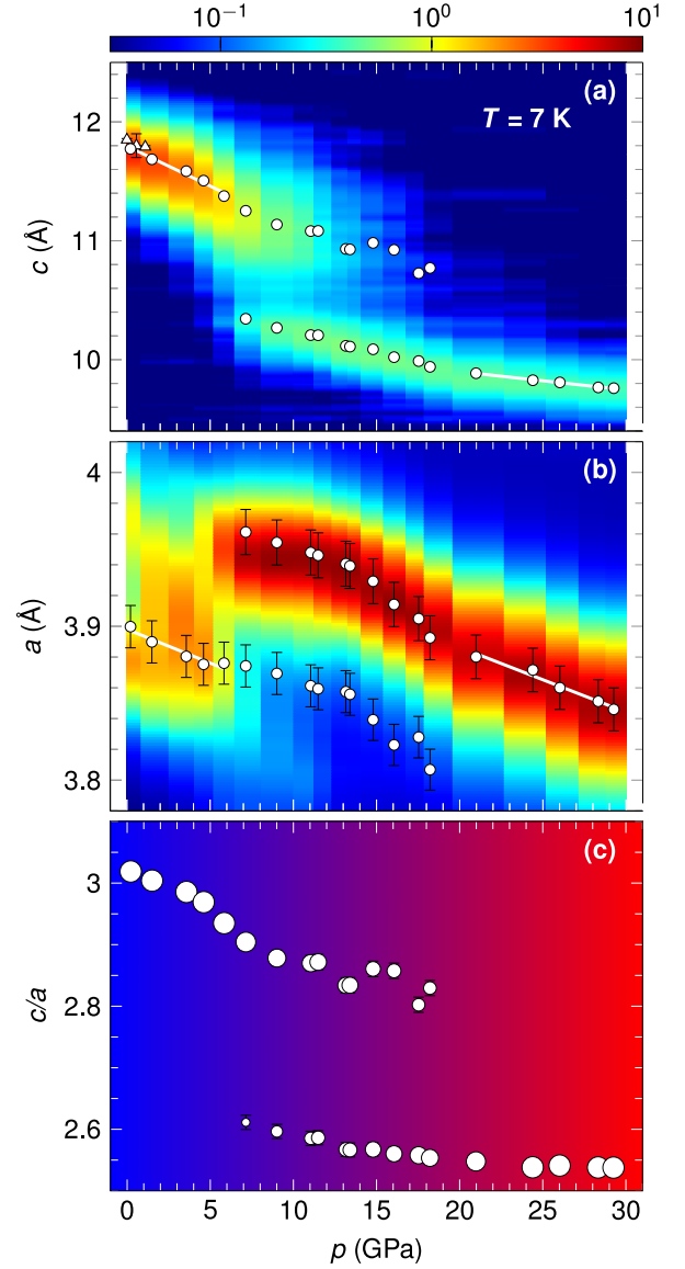
FIG. 2. (color online) Evolution of the unit cell dimensions with pressure. The detector counts are color-coded on a log scale in units of 10^{-5} counts/monitor. (a) The c -lattice parameter determined from the (0 0 2) HE-XRD powder Bragg peak (solid white circles) and the (0 0 8) neutron single crystal Bragg peak (solid white triangles). (b) The a -lattice parameter determined from the (1 1 2) HE-XRD powder Bragg peak and the c -lattice parameter from panel (a). The solid white lines in (a) and (b) are linear fits to the pressure dependence of the lattice parameter. (c) The \frac{c}{a} ratio determined from the data in panels (a) and (b). The area of the circles represent the volume fractions of the T and cT phases and the background color provides a guide to the eye.
