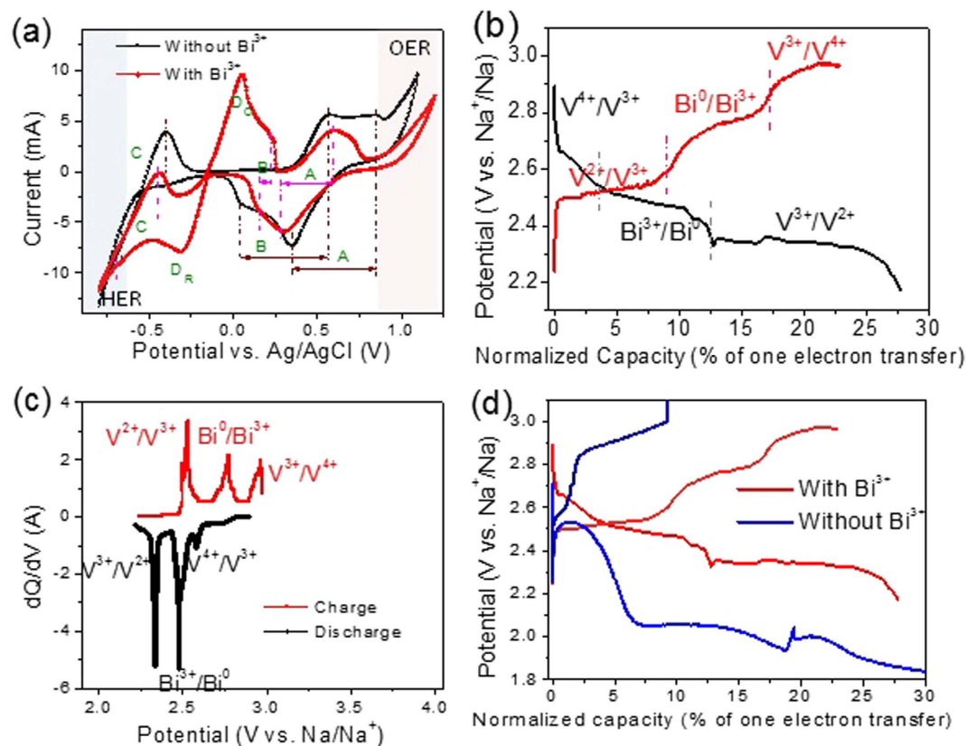
Figure 5. (a) CV curves of aqueous electrolytes with and without BiCl 3 in half cells at a scan rate of 10 mV/s in which a graphite felt, Ag/AgCl, and Pt wire were used as the working, reference, and counter electrodes, respectively; (b) the charge/discharge profile (1 st cycle) of a full cell at 0.02 mA with the 0.01 M VOSO 4 – 0.05 M Na 2 SO 4 – 1.5 M HCl – 0.002 M BiCl 3 aqueous solution as the catholyte and the Na chip anode with the 0.5 M NaTFSI / pyrrTFSi electrolyte in which the three charge/discharge plateaus are identified; (c) the differential capacity vs. voltage of the charge/discharge profile in (b); and (d) the comparison of the charge/discharge profiles between the full cells with and without BiCl 3 in catholytes.
