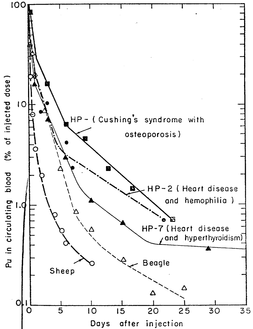
Fig. 2. Disappearance of Pu from the blood of man, dog, and sheep. Dog data are from Stover et al. 28 , all dose levels combined; sheep data are from McClellan et al. 38, 39
