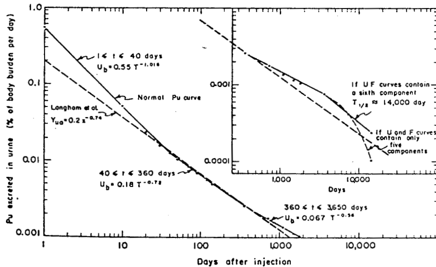
Fig. 9. Comparison of the percent of the Pu body content excreted daily in the urine from 1 day to 40 years predicted by the normal Pu urine and fecal curves in this paper and the equations of Langham et al. 19 Points shown were calculated from the parameters given in Table VI.
