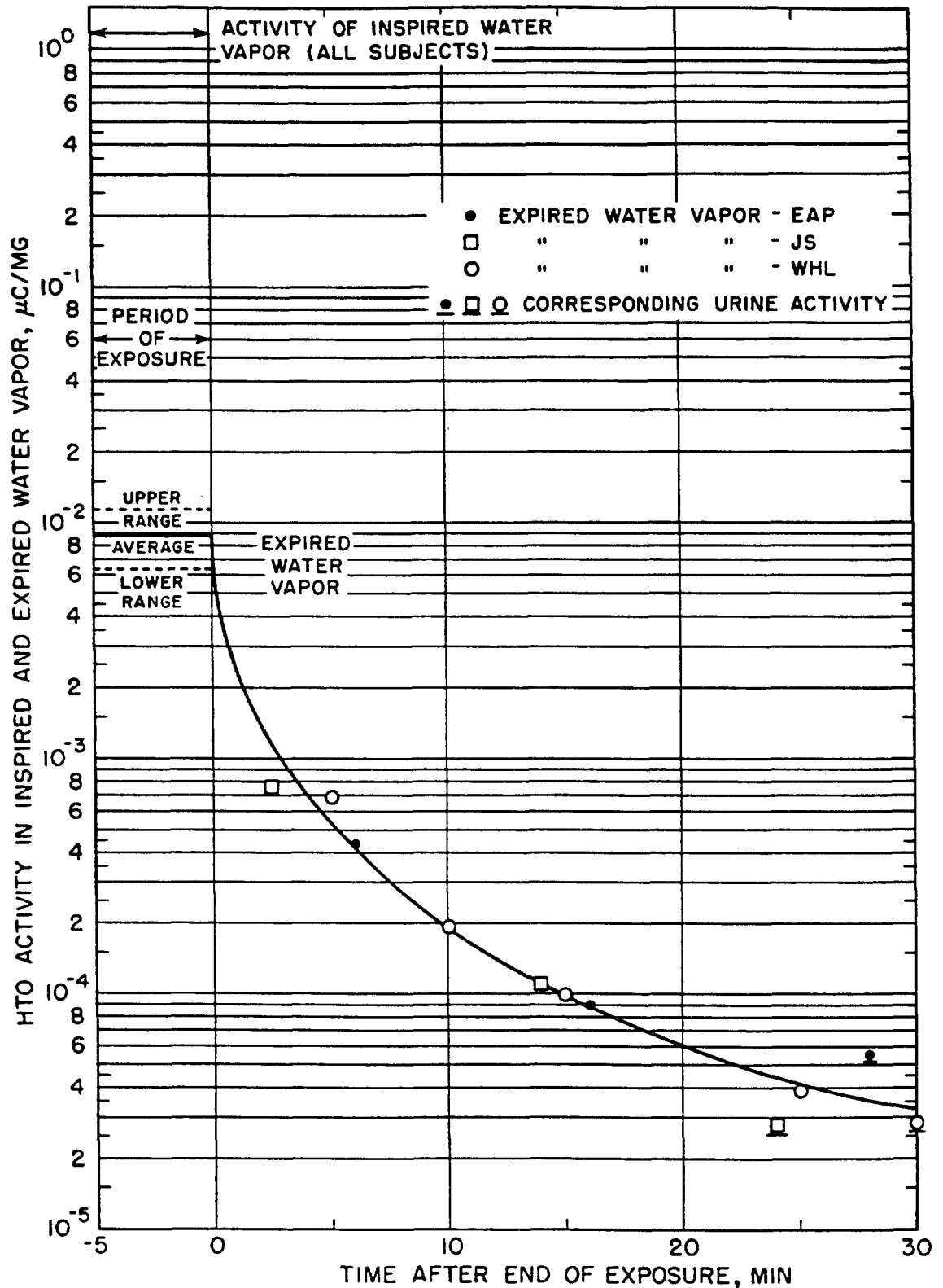
Fig. 2. HTO activity in expired water during and following exposure to HTO vapor in inspired air.
