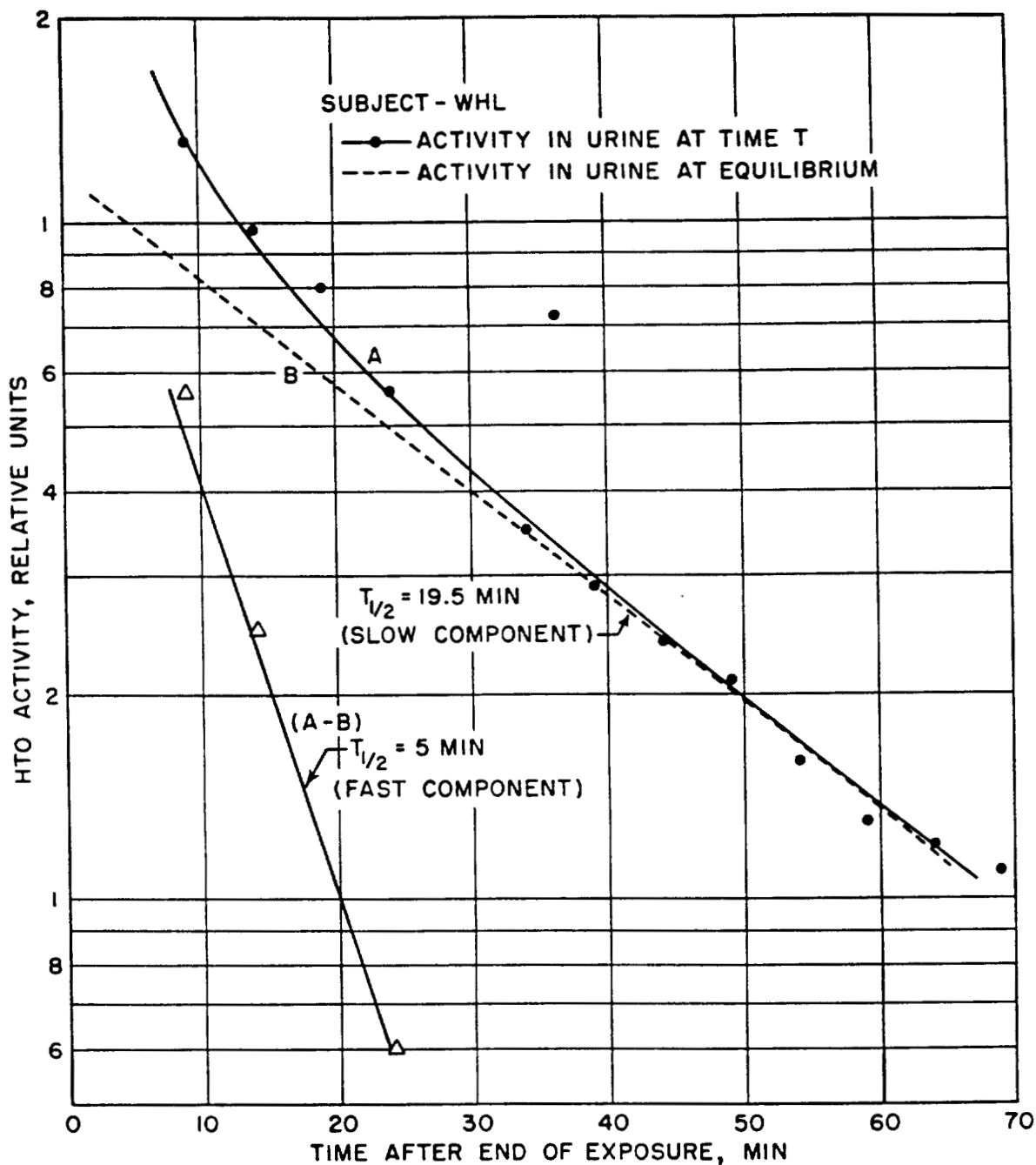
Fig. 6. Exponential decline of HTO activity in urine with time after exposure to HTO in inspired gas.
