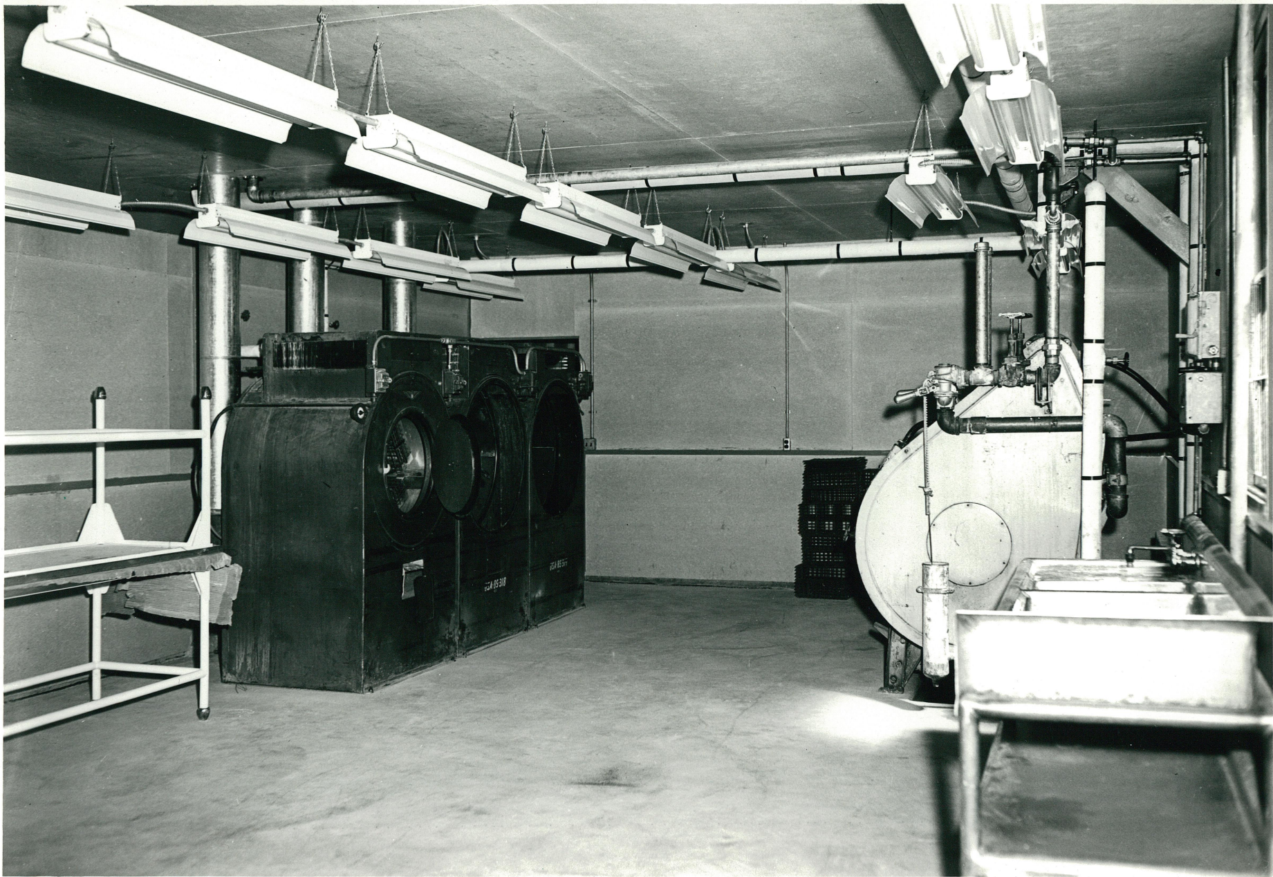
OFFICIAL USE ONLY HOO, Richland, Washington Mask Washing Station, 200-W, CA-596 Taken: 8-23-55 Showing interior of completed laundry room. 100% complete L. A. Hopkins Co., AT(45-1)-871
