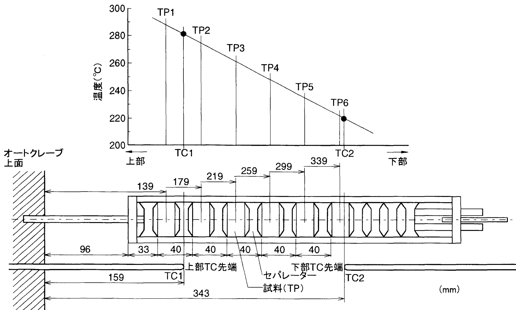
Fig. 15 Alignment of corrosion test pieces and estimated temperature
