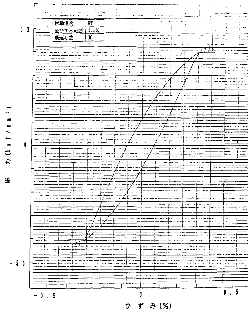
Fig. B-10 Stress-Strain hysteresis diagram of fatigue test at room temperature (Specimen ID:7, Total strain range: 0.6%, Cycle number: 30)
