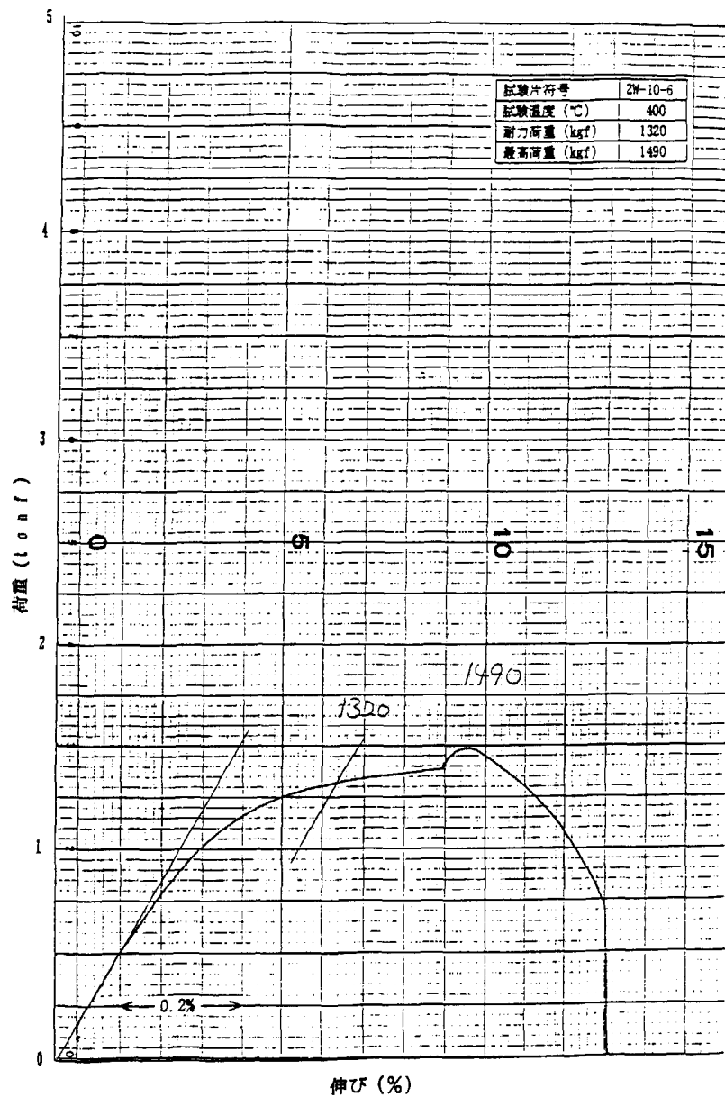
Fig. A-5 Load-Displacement diagram of tensile test at 400°C (2W-10-6)
