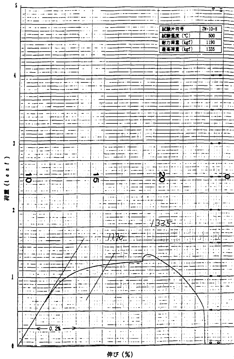
Fig. A-7 Load-Displacement diagram of tensile test at 500°C (2W-10-8)
