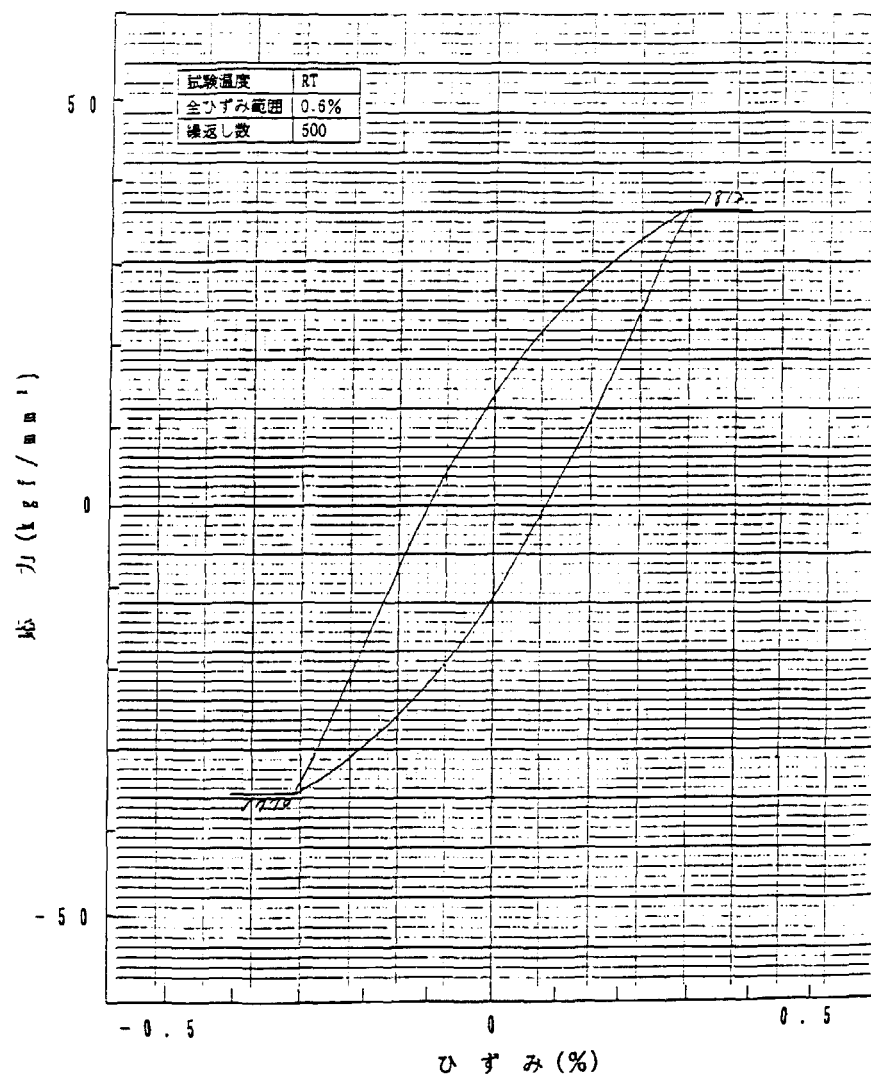
Fig. B-13 Stress-Strain hysteresis diagram of fatigue test at room temperature (Specimen ID:7, Total strain range: 0.6%, Cycle number: 500)
