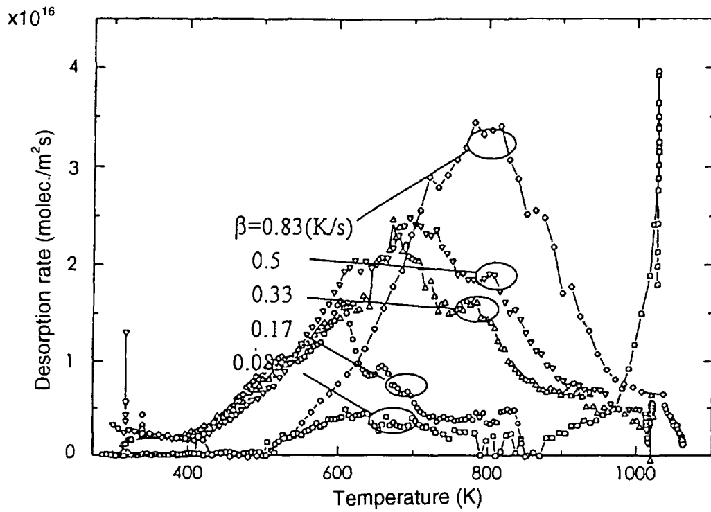
Fig. 52 TDS spectrum of CH 4 gas from F82H IEA heat with heating rate variation ( \beta = 0.17 \sim 0.83 K/s)
