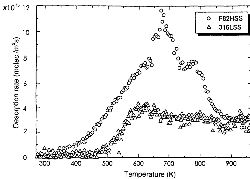
Fig. 47 TDS spectrum of \text{CH}_4 gas from F82H IEA heat ( \beta = 0.17 \text{ K/s} )
