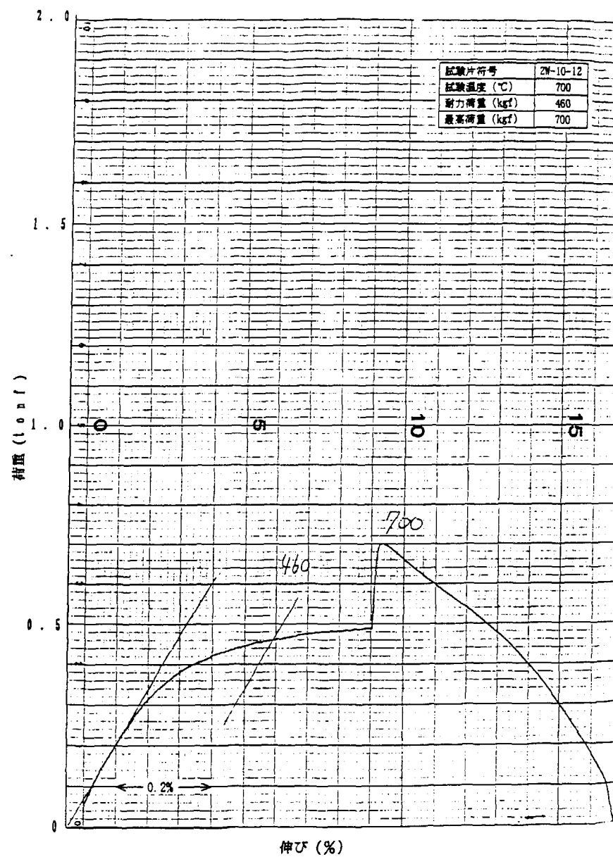
Fig. A-11 Load-Displacement diagram of tensile test at 700°C (2W-10-12)
