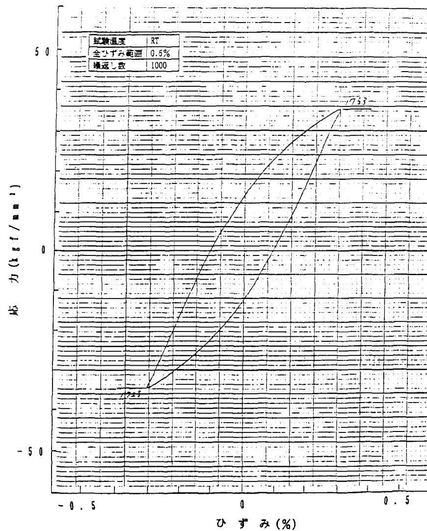
Fig. B-14 Stress-Strain hysteresis diagram of fatigue test at room temperature (Specimen ID:7, Total strain range: 0.6%, Cycle number: 1000)
