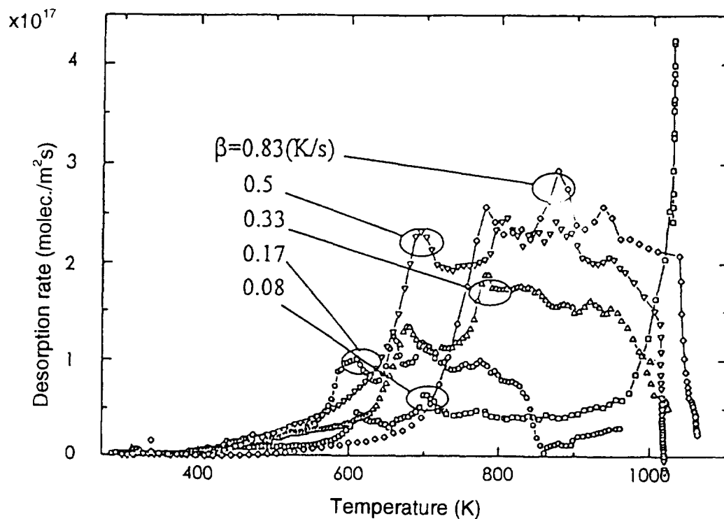
Fig. 48 TDS spectrum of \text{H}_2 gas from F82H IEA heat with heating rate variation ( \beta = 0.17 \sim 0.83 K/s)
