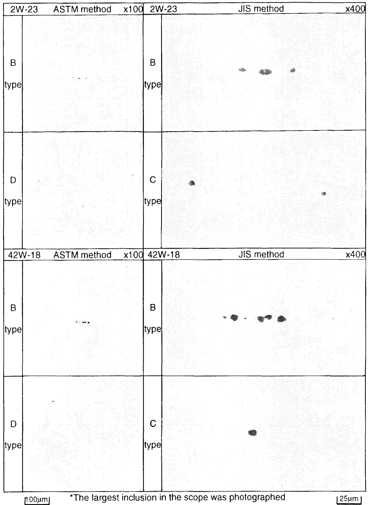
Photo 4 Non-metallic inclusion in F82H IEA heat (2W-23, 42W-18)
