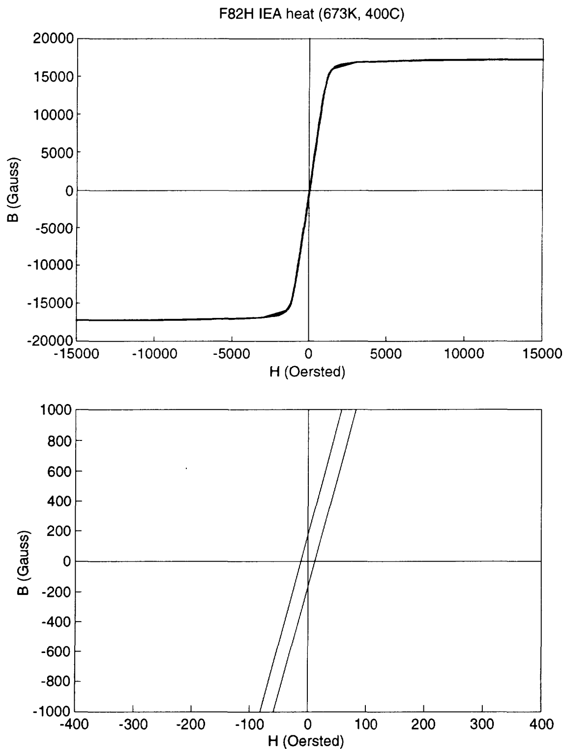
Fig. 28 Hysteresis curve of F82H IEA heat (673K, 400C)
