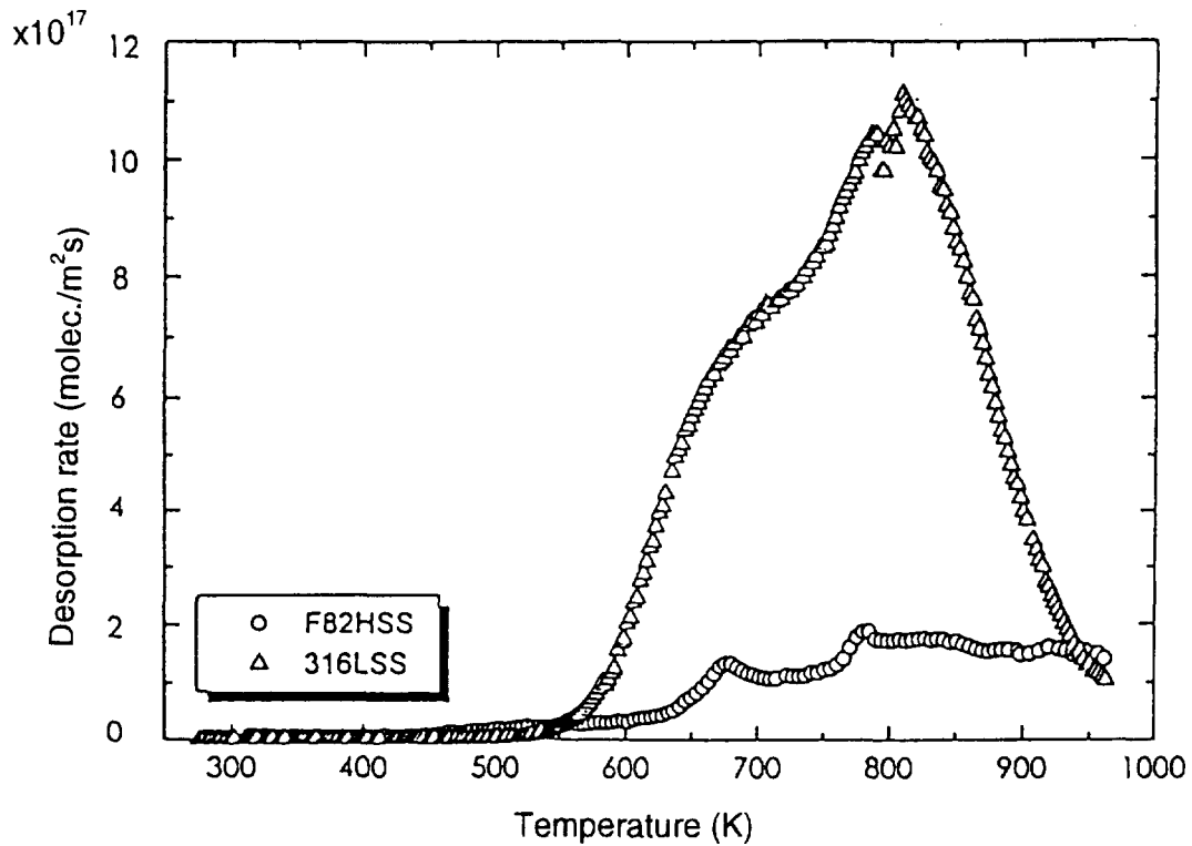
Fig. 43 TDS spectrum of \text{H}_2 gas from F82H IEA heat ( \beta = 0.17 \text{ K/s} )
