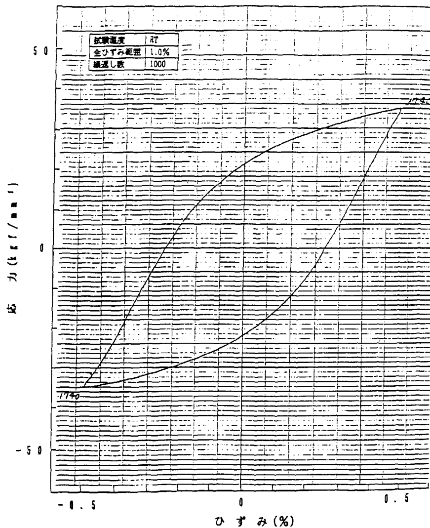
Fig. B-7 Stress-Strain hysteresis diagram of fatigue test at room temperature (Specimen ID:6, Total strain range: 1.0%, Cycle number: 1000)
