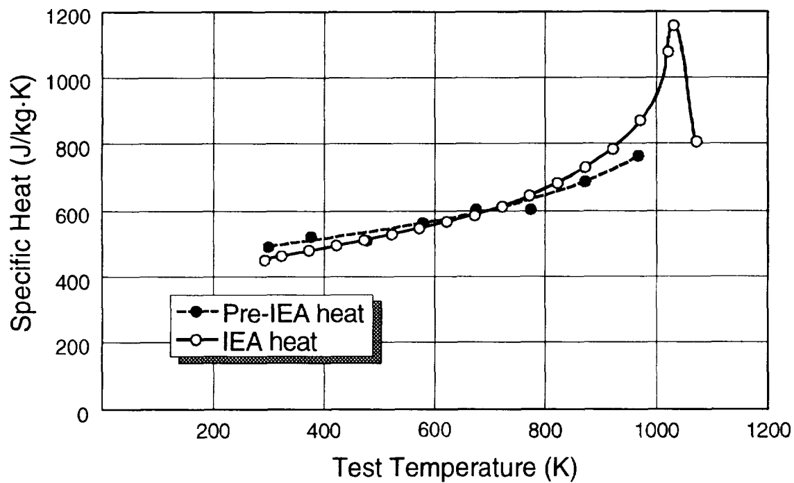
Fig. 16 Specific heat of F82H IEA heat
