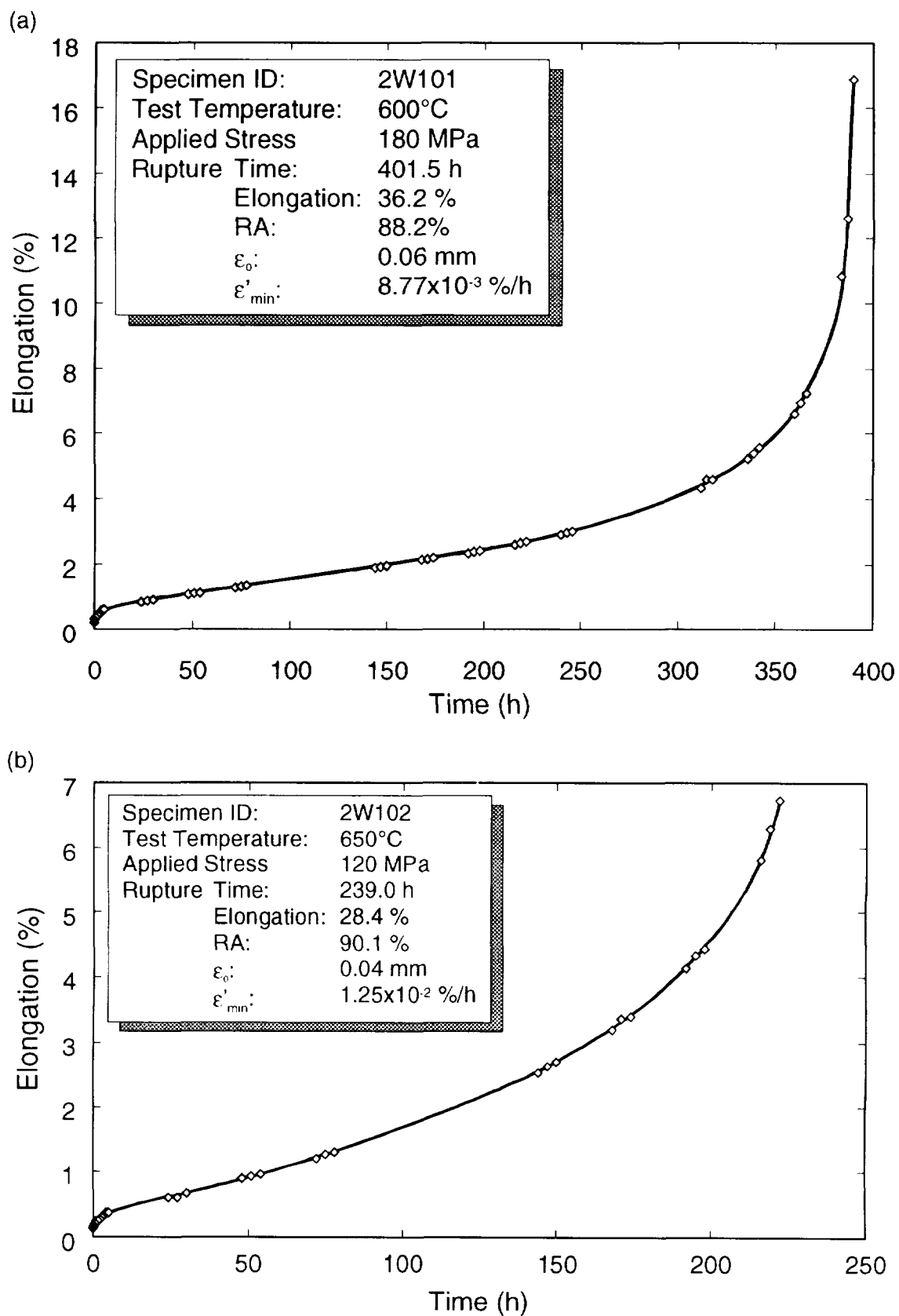
Fig. 33 Creep rupture test result of F82H IEA heat
