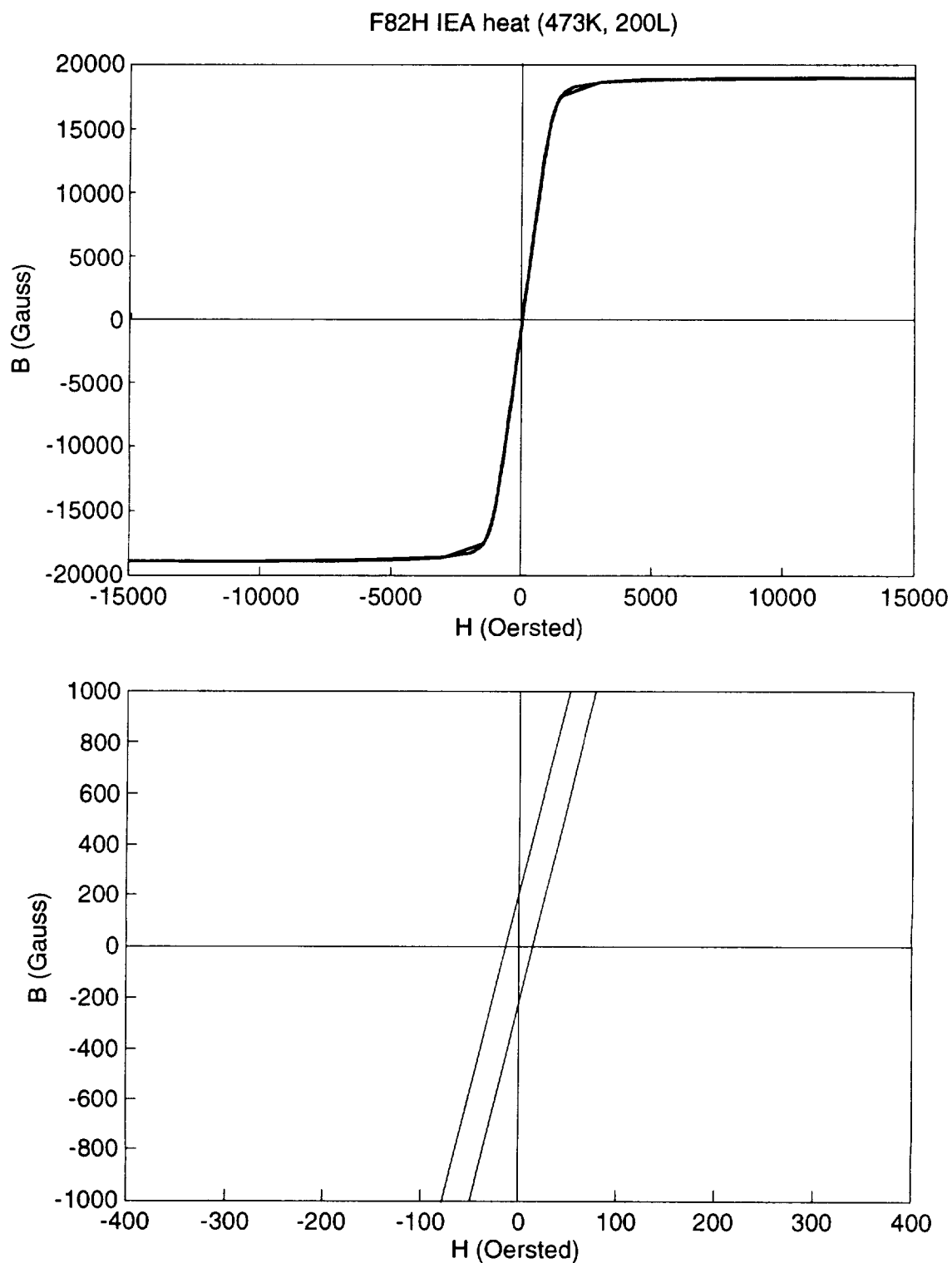
Fig. 23 Hysteresis curve of F82H IEA heat (473K, 200L)
