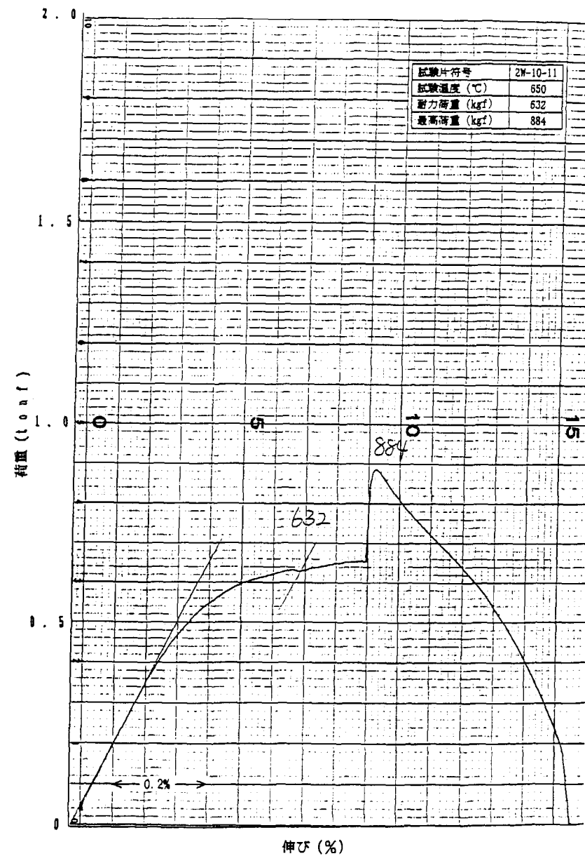
Fig. A-10 Load-Displacement diagram of tensile test at 650°C (2W-10-11)
