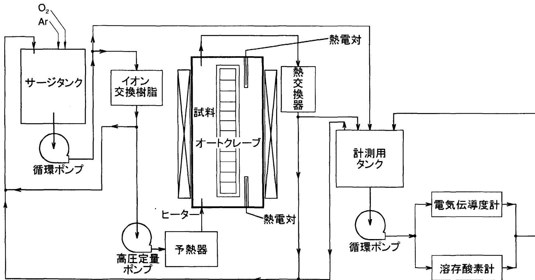
Fig. 14 High-temperature water circulation system for corrosion teset
