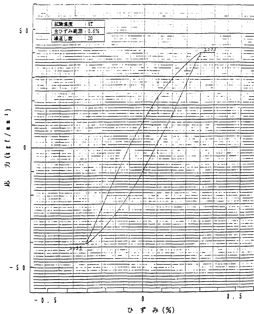
Fig. B-9 Stress-Strain hysteresis diagram of fatigue test at room temperature (Specimen ID:7, Total strain range: 0.6%, Cycle number: 20)
