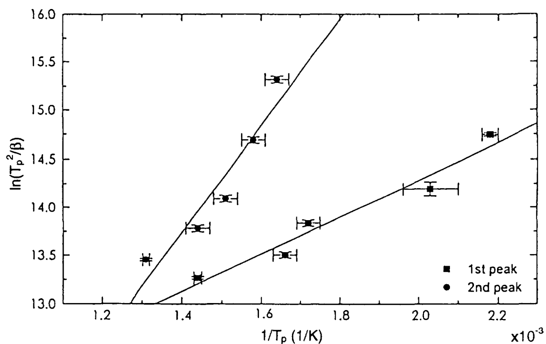
Fig. 54 The relationship between desorption peak temperature of H_2O and heating rate \beta .
