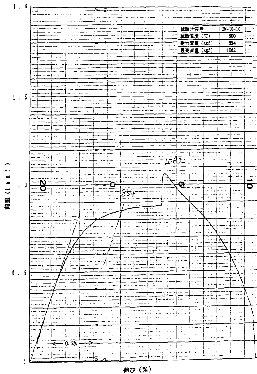
Fig. A-9 Load-Displacement diagram of tensile test at 600°C (2W-10-10)
