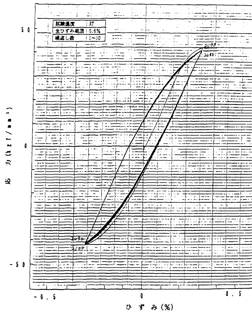
Fig. B-8 Stress-Strain hysteresis diagram of fatigue test at room temperature (Specimen ID:7, Total strain range: 0.6%, Cycle number: 1-10)
