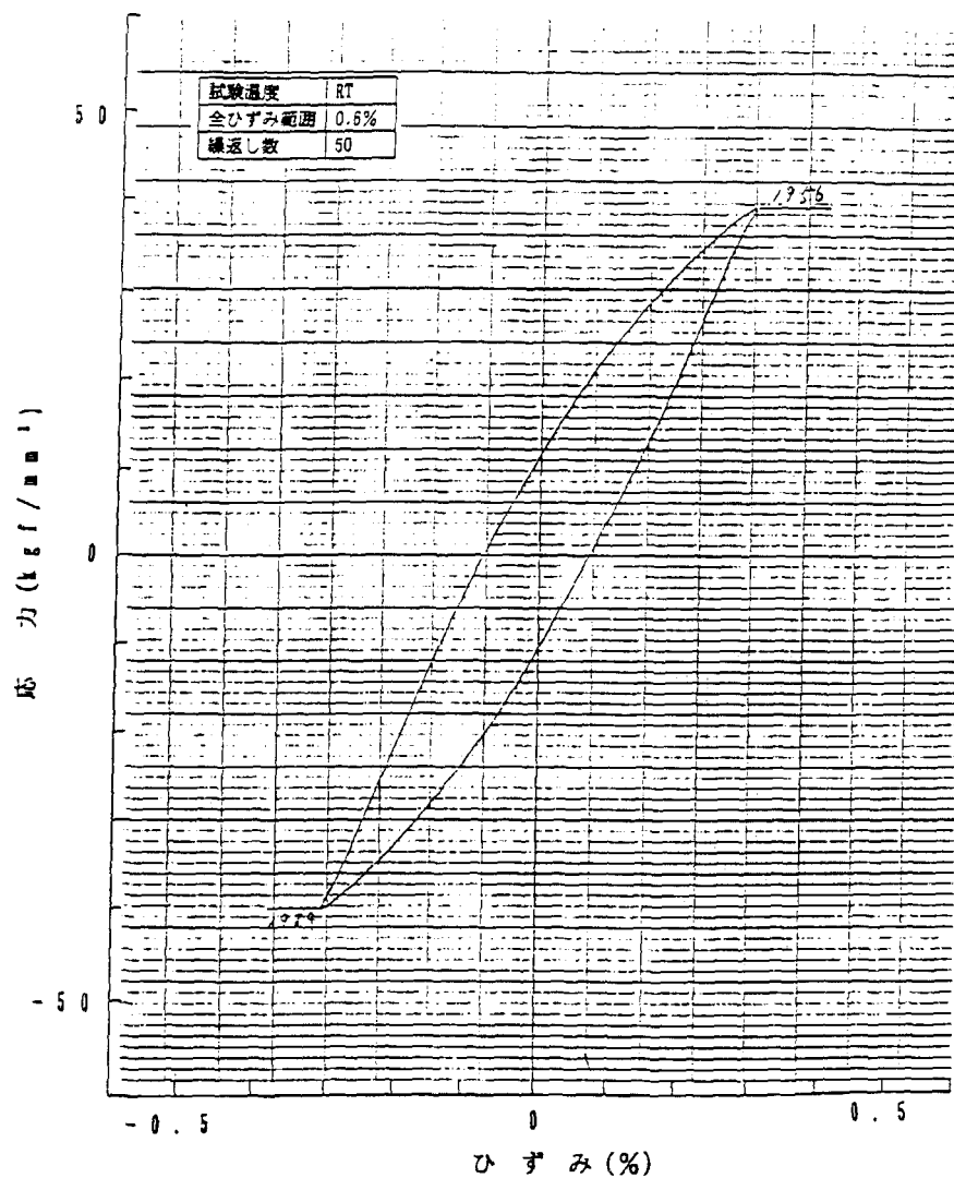
Fig. B-11 Stress-Strain hysteresis diagram of fatigue test at room temperature (Specimen ID:7, Total strain range: 0.6%, Cycle number: 50)
