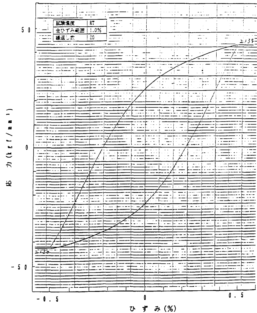
Fig. B-2 Stress-Strain hysteresis diagram of fatigue test at room temperature (Specimen ID:6, Total strain range: 1.0%, Cycle number: 20)
