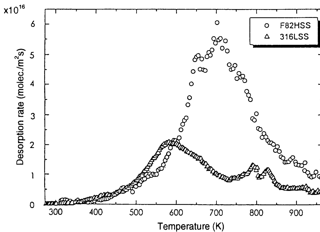
Fig. 46 TDS spectrum of CO 2 gas from F82H IEA heat ( \beta = 0.17 K/s)
