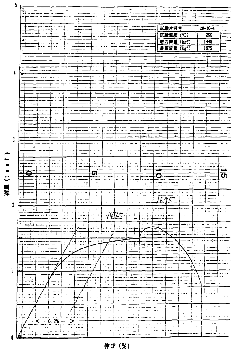
Fig. A-3 Load-Displacement diagram of tensile test at 200°C (2W-10-4)
