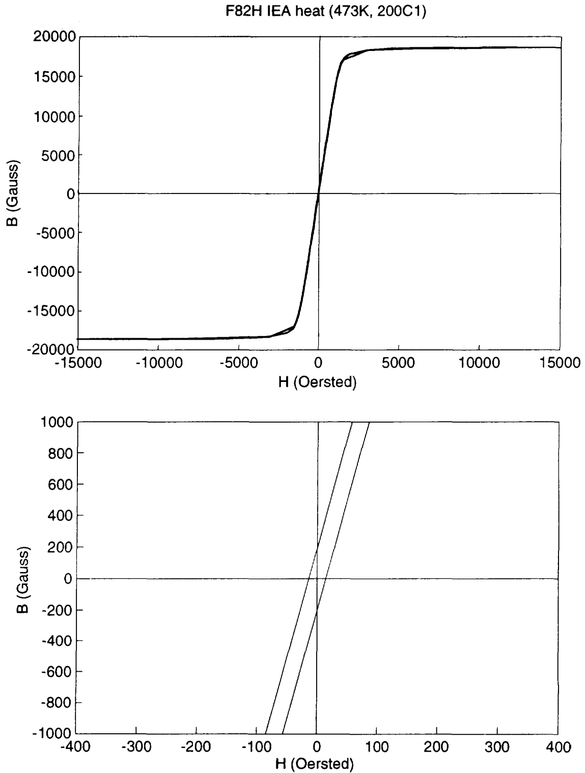
Fig. 24 Hysteresis curve of F82H IEA heat (473K, 200C1)
