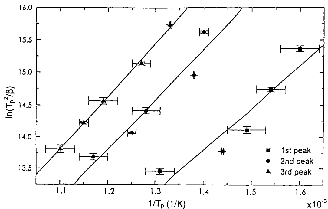
Fig. 53 The relationship between desorption peak temperature of H_2 and heating rate \beta .
