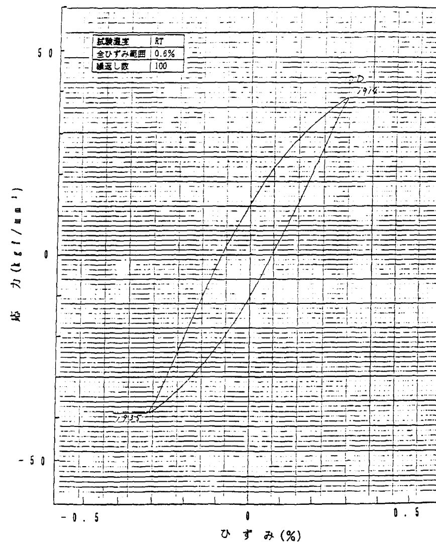
Fig. B-12 Stress-Strain hysteresis diagram of fatigue test at room temperature (Specimen ID:7, Total strain range: 0.6%, Cycle number: 100)
