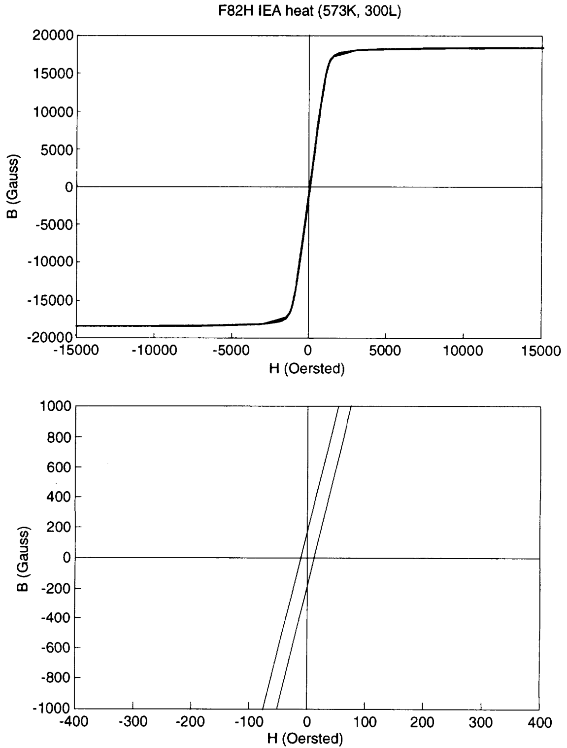
Fig. 25 Hysteresis curve of F82H IEA heat (573K, 300L)
