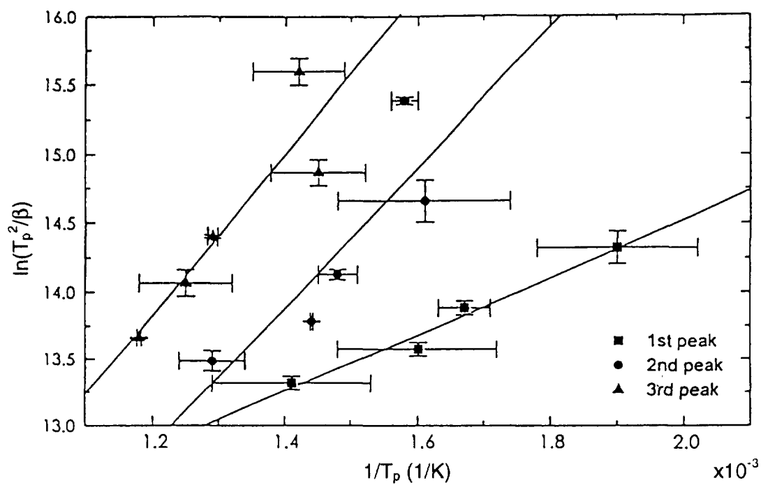
Fig. 57 The relationship between desorption peak temperature of \text{CH}_4 and heating rate \beta .
