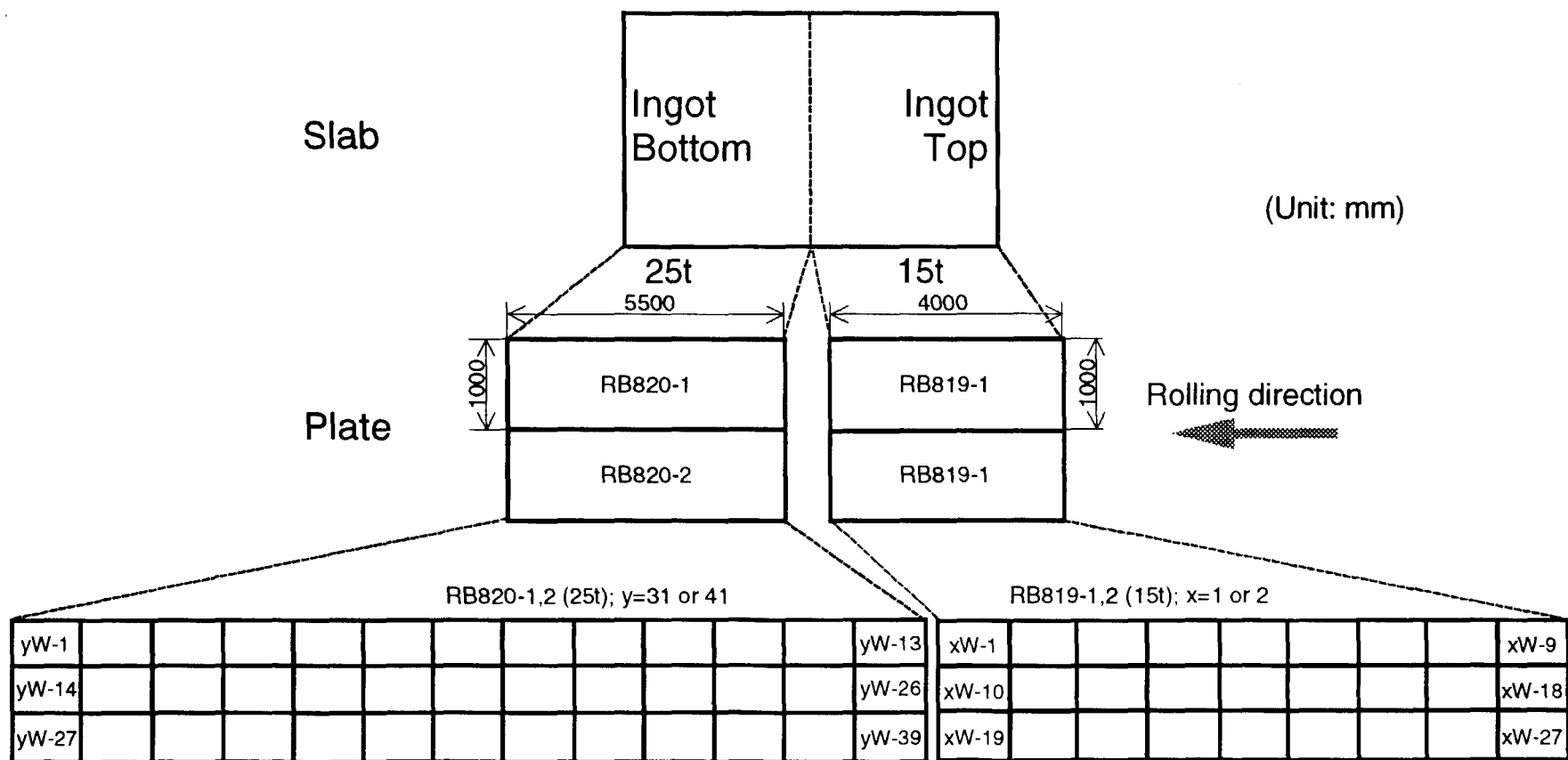
Fig. 5 F82H IEA heat (Heat No. 9753)
