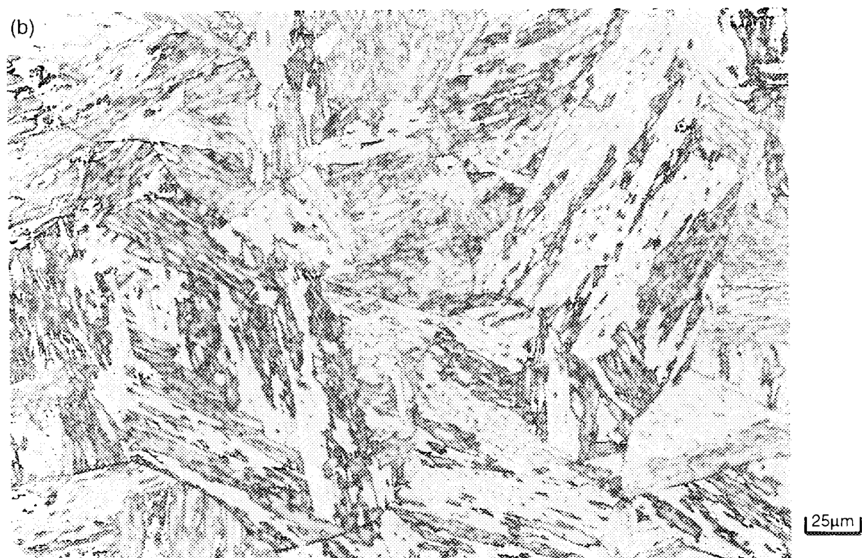
Photo 6 Microstructure of F82H IEA heat (2W-23); (a) x100, (b) x400
