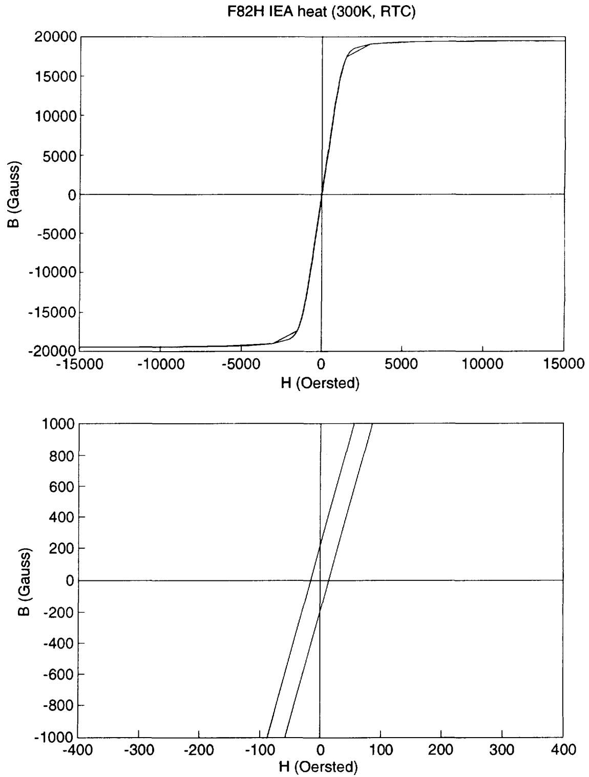
Fig. 22 Hysteresis curve of F82H IEA heat (300K, RTC)
