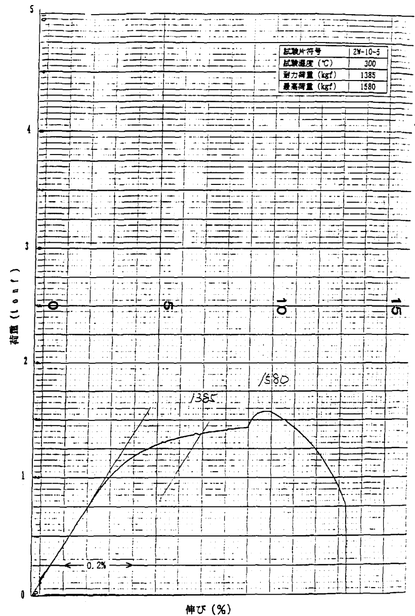
Fig. A-4 Load-Displacement diagram of tensile test at 300°C (2W-10-5)
