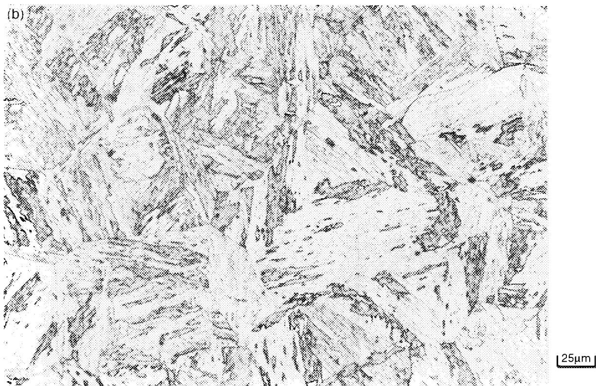
Photo 7 Microstructure of F82H IEA heat (42W-18); (a) x100, (b) x400
