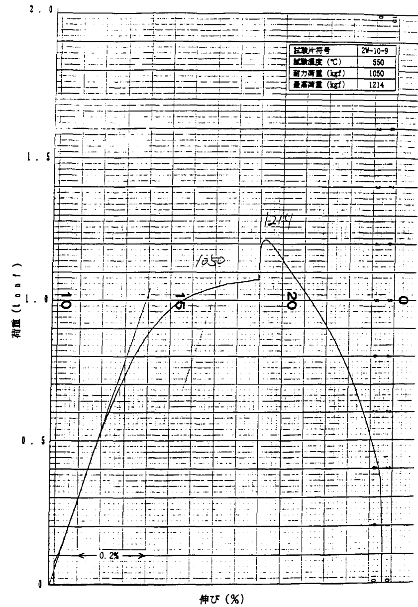
Fig. A-8 Load-Displacement diagram of tensile test at 550°C (2W-10-9)
