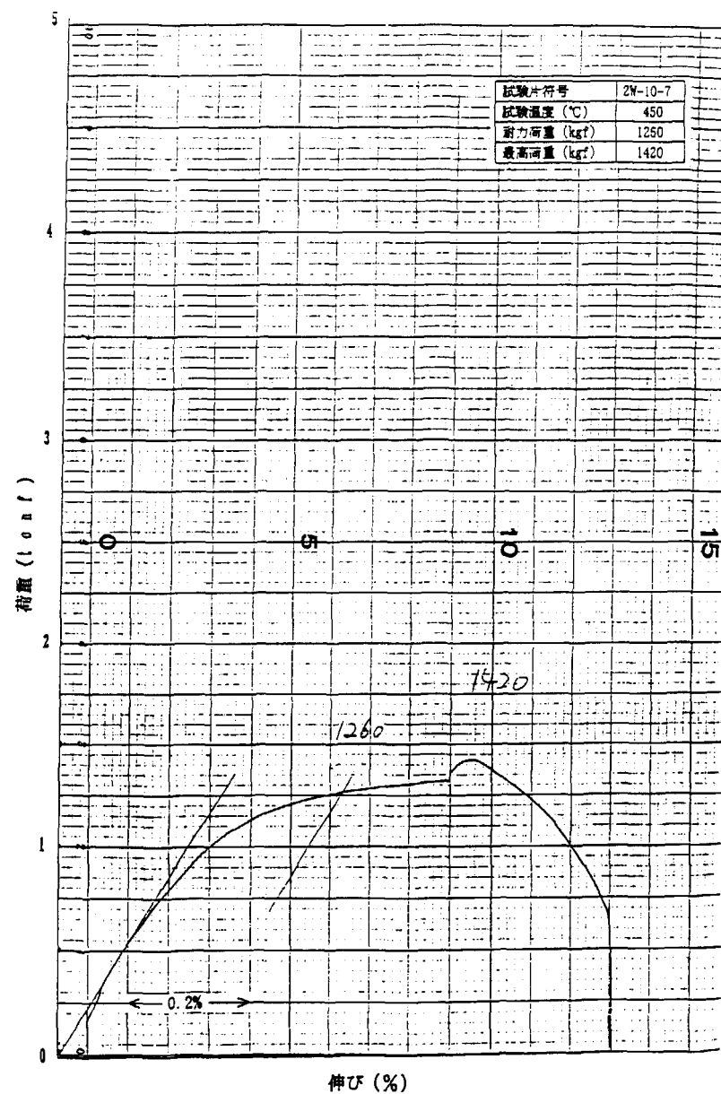
Fig. A-6 Load-Displacement diagram of tensile test at 450°C (2W-10-7)
