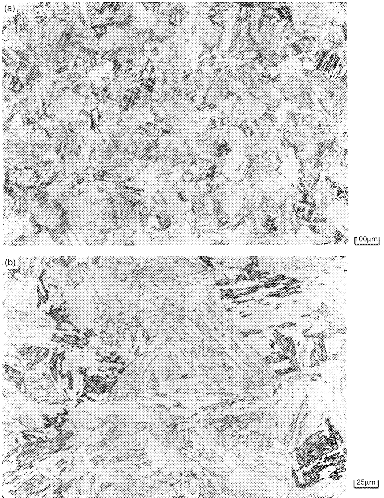
Photo 5 Microstructure of F82H IEA heat (5-16); (a) x100, (b) x400
