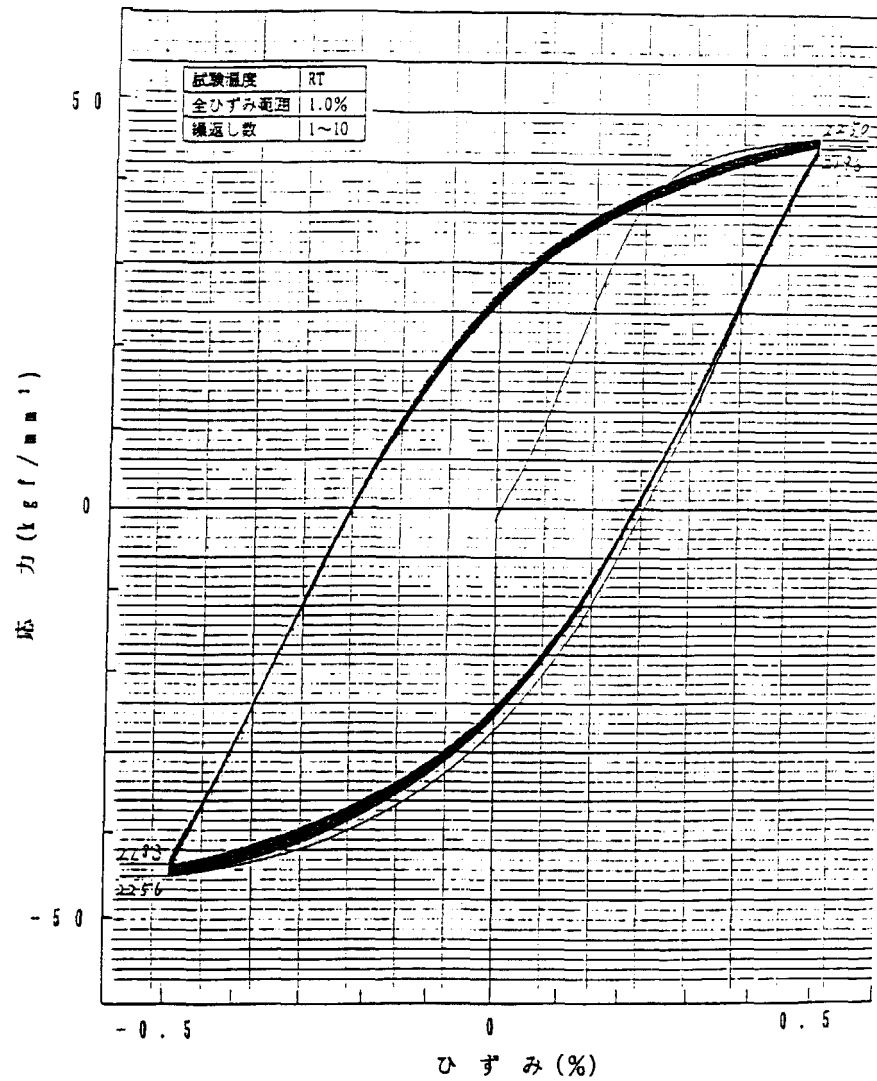
Fig. B-1 Stress-Strain hysteresis diagram of fatigue test at room temperature (Specimen ID:6, Total strain range: 1.0%, Cycle number: 1-10)
