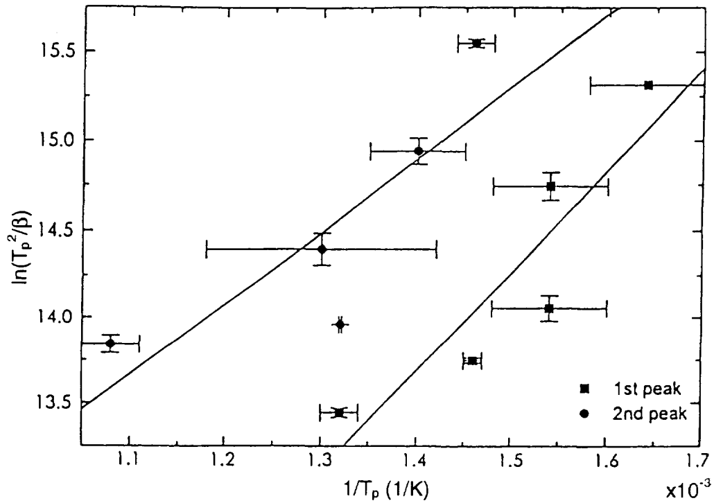
Fig. 55 The relationship between desorption peak temperature of CO and heating rate \beta .
