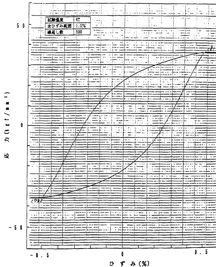
Fig. B-6 Stress-Strain hysteresis diagram of fatigue test at room temperature (Specimen ID:6, Total strain range: 1.0%, Cycle number: 500)
