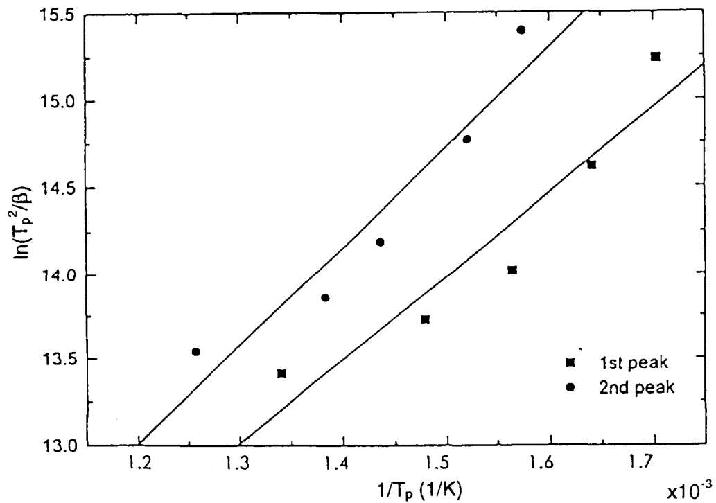
Fig. 56 The relationship between desorption peak temperature of CO 2 and heating rate \beta .
