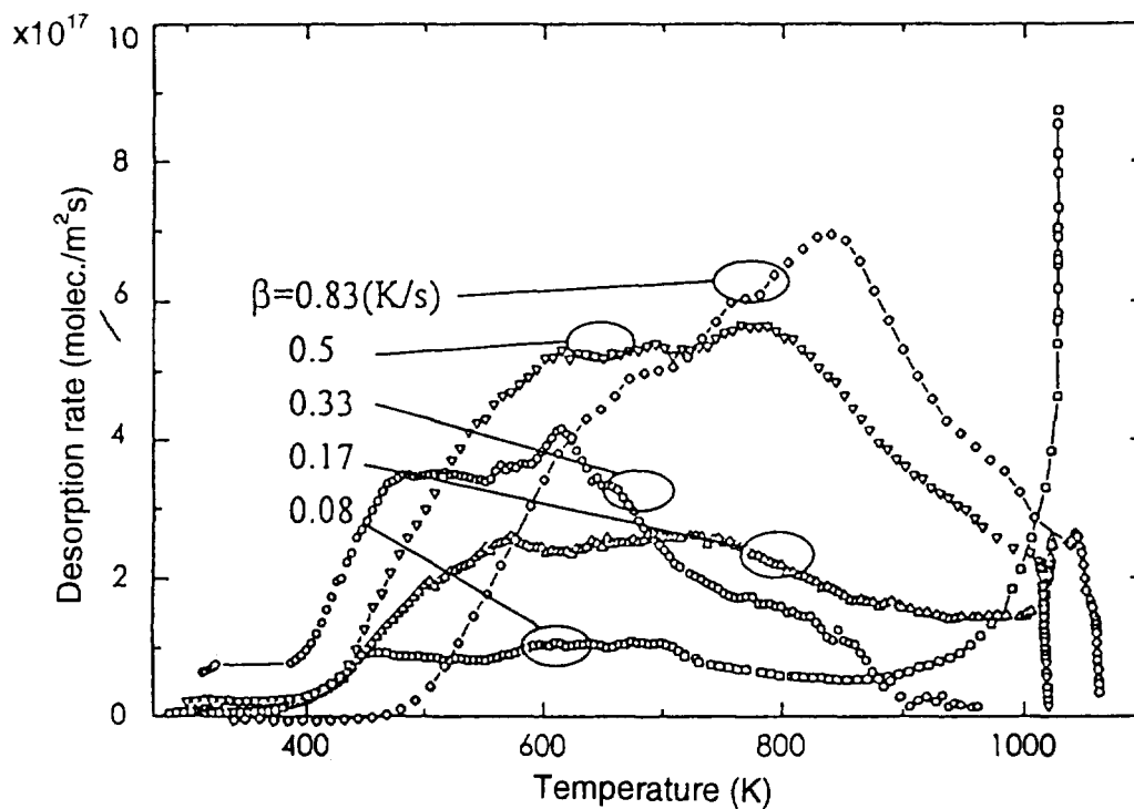
Fig. 49 TDS spectrum of \text{H}_2\text{O} gas from F82H IEA heat with heating rate variation ( \beta = 0.17 \sim 0.83 K/s)
