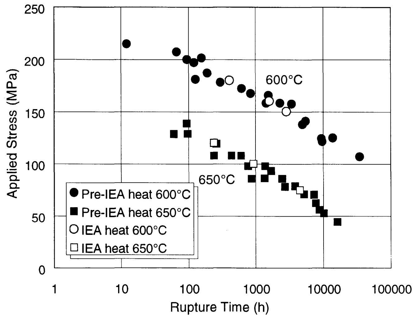
Fig. 36 Creep rupture test result of F82H
