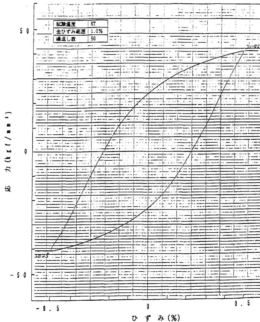
Fig. B-4 Stress-Strain hysteresis diagram of fatigue test at room temperature (Specimen ID:6, Total strain range: 1.0%, Cycle number: 50)
