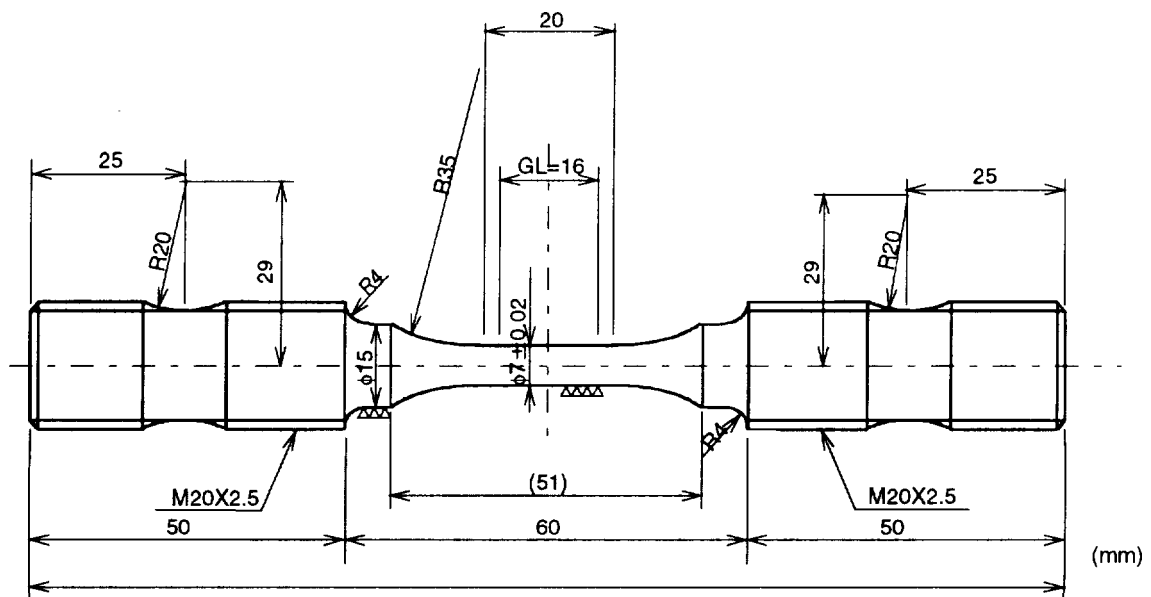
Fig. 12 Dimension of the fatigue test specimen
