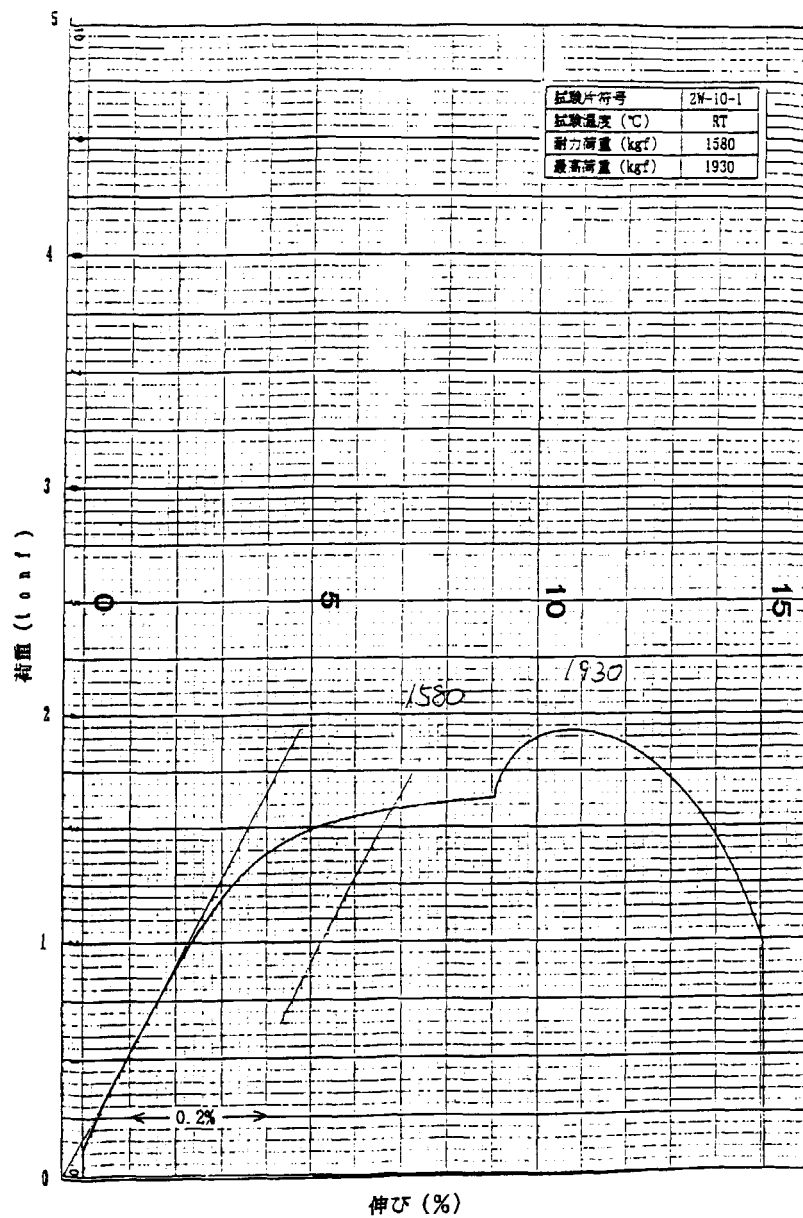
Fig. A-1 Load-Displacement diagram of tensile test at room temperature (2W-10-1)
