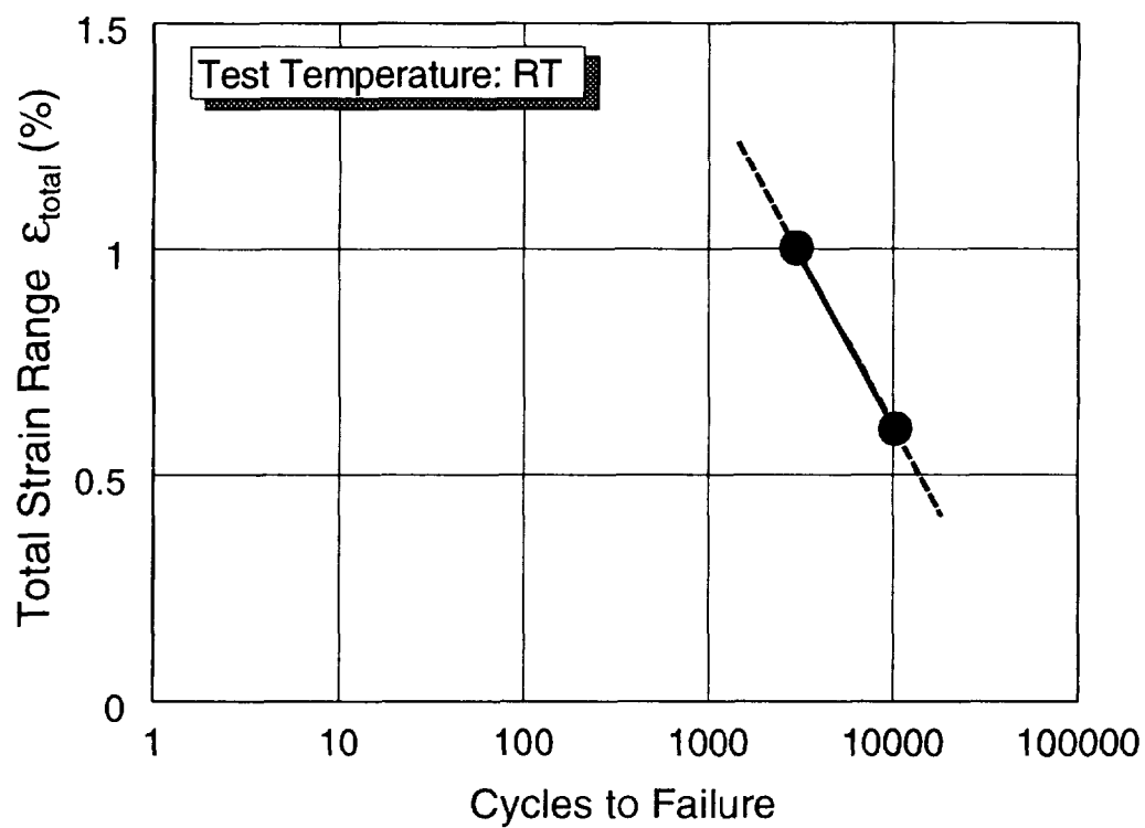
Fig. 38 Low cycle fatigue test results of F82H IEA heat
