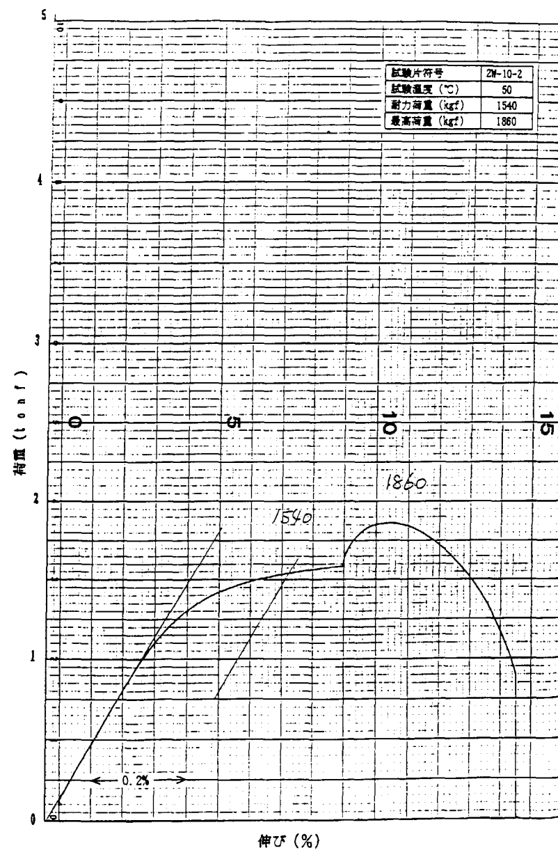
Fig. A-2 Load-Displacement diagram of tensile test at 50°C (2W-10-2)
