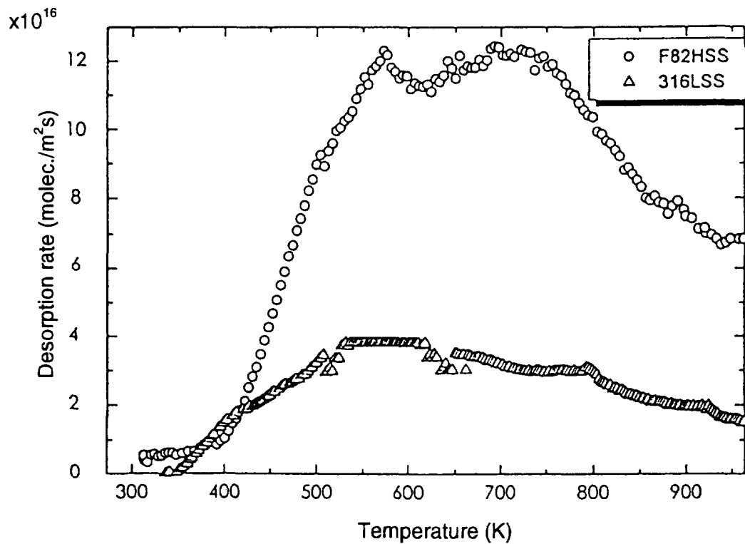
Fig. 44 TDS spectrum of \text{H}_2\text{O} gas from F82H IEA heat ( \beta = 0.17 \text{ K/s} )
