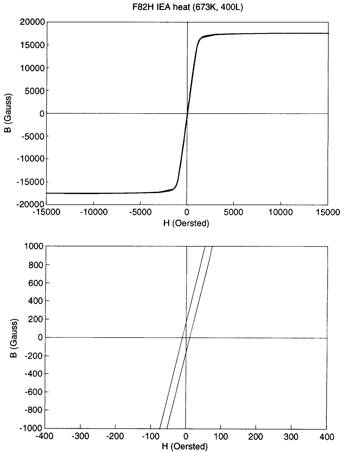
Fig. 27 Hysteresis curve of F82H IEA heat (673K, 400L)
