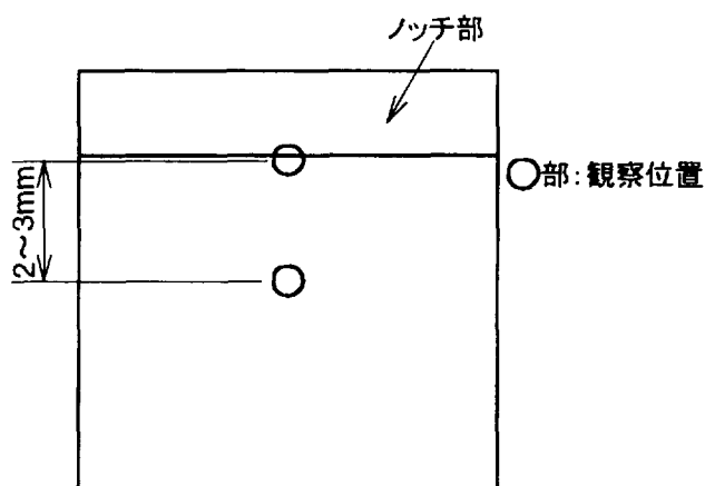
Fig. 11 Positions of the SEM observation of fracture surface after Charpy test
