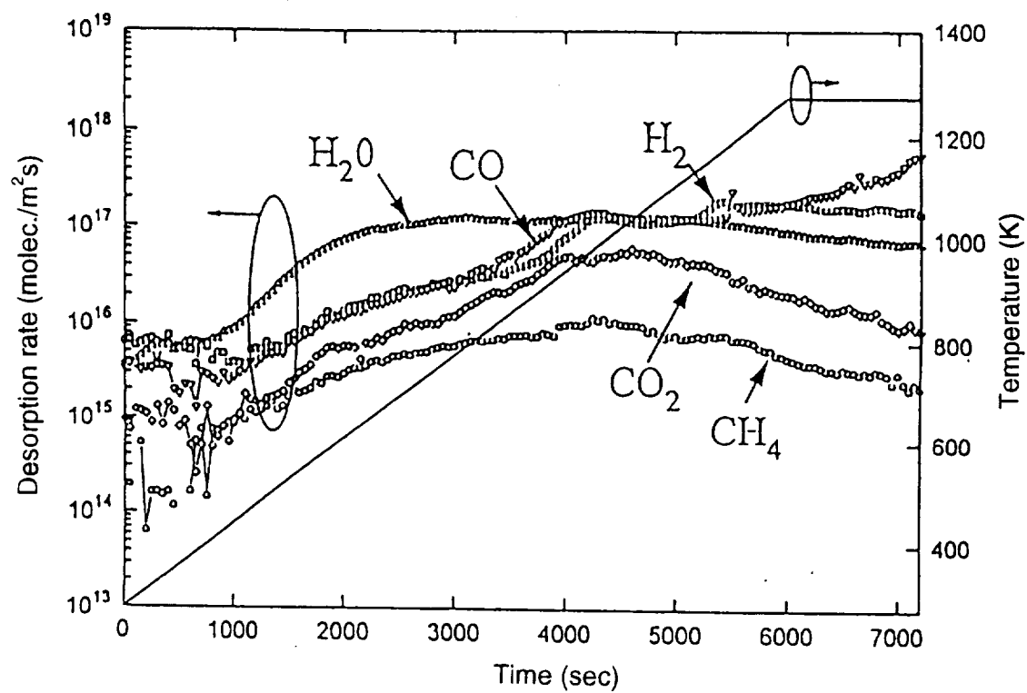
Fig. 42 TDS spectrum of F82H IEA heat ( \beta = 0.17 \text{ K/s} )
