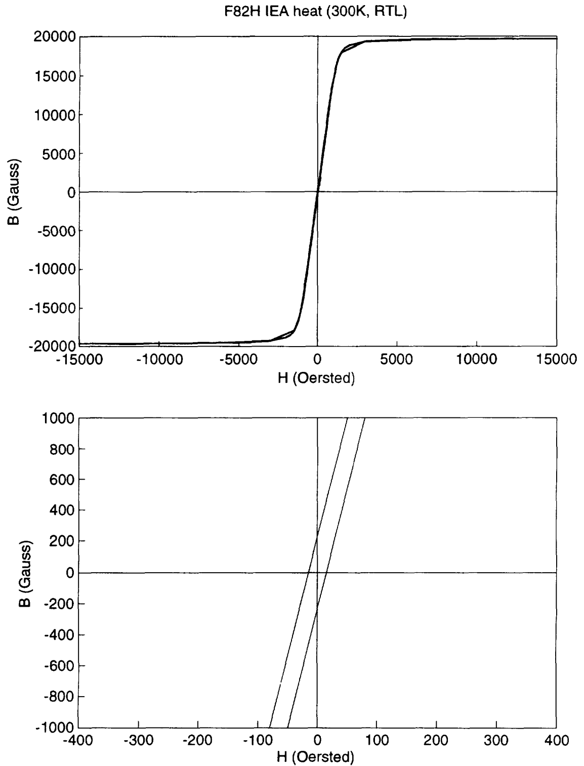
Fig. 21 Hysteresis curve of F82H IEA heat (300K, RTL)
