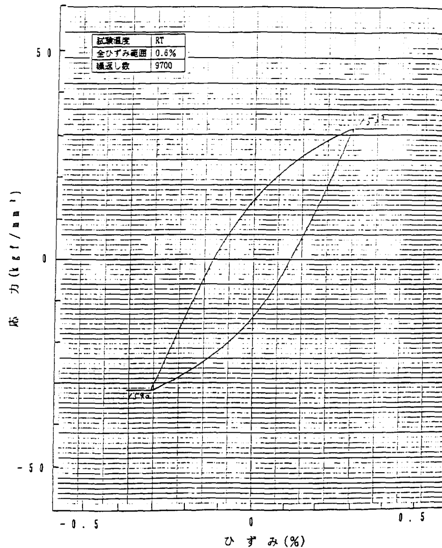
Fig. B-16 Stress-Strain hysteresis diagram of fatigue test at room temperature (Specimen ID:7, Total strain range: 0.6%, Cycle number: 9700)
