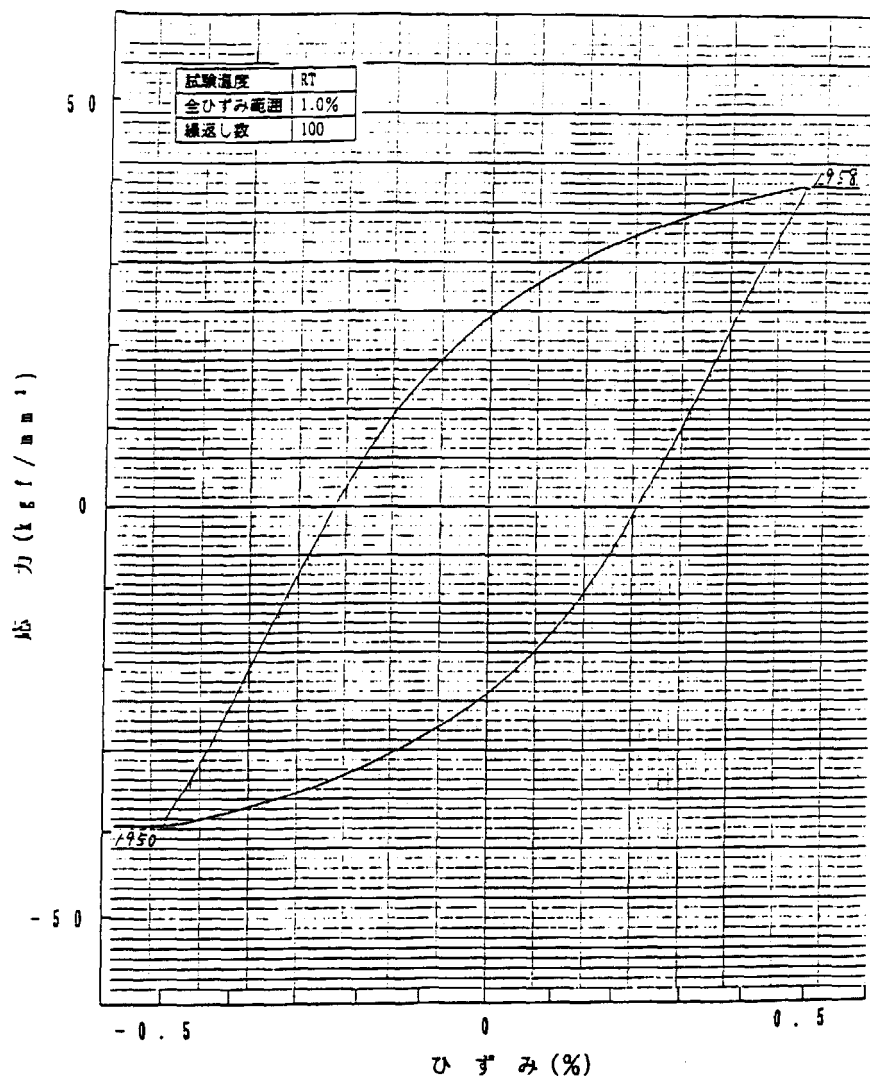
Fig. B-5 Stress-Strain hysteresis diagram of fatigue test at room temperature (Specimen ID:6, Total strain range: 1.0%, Cycle number: 100)
