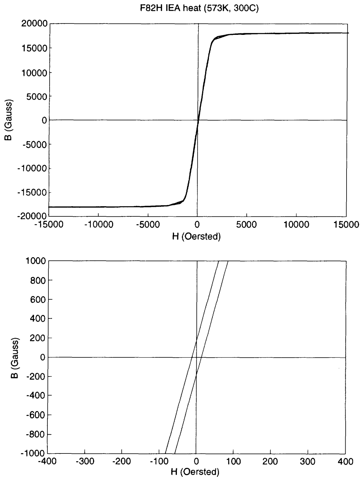
Fig. 26 Hysteresis curve of F82H IEA heat (573K, 300C)
