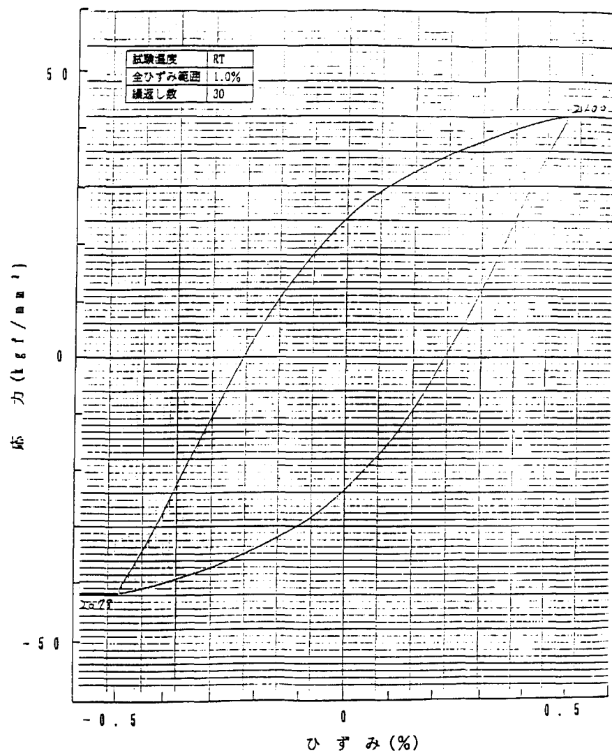
Fig. B-3 Stress-Strain hysteresis diagram of fatigue test at room temperature (Specimen ID:6, Total strain range: 1.0%, Cycle number: 30)
