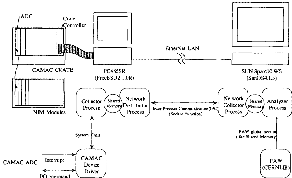
Fig. 4 : The hardware and software configuration of the DAQ system
