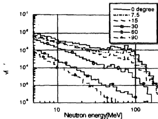
Fig. 10 : Neutron spectra from 100MeV/u carbon ions in a aluminum target.
