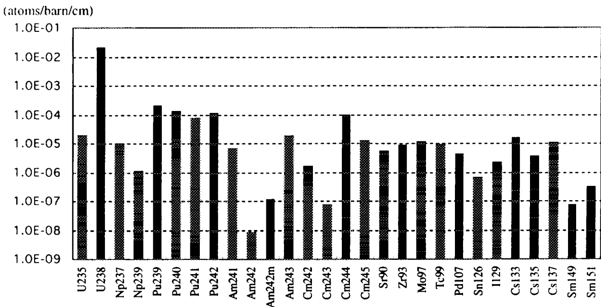
Fig. 5 Nuclide number density of thermal reactor
