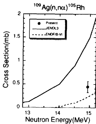
Fig.2.9 Cross section of ^{109}\text{Ag}(n,\alpha)^{105}\text{Rh} .
