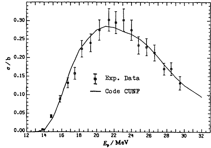
Fig. 25 Cross sections of 57 Fe(p,2n) 56 Co reaction
