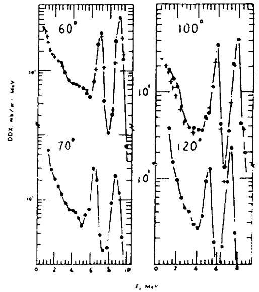
Fig. 4 DDCSs of secondary neutrons of ^9\text{Be} at 10.1 MeV • present work † M. Drake et al.
