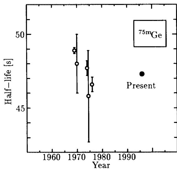
Fig. 3: Result of ^{75m}\text{Ge} and comparison with the previous works.
