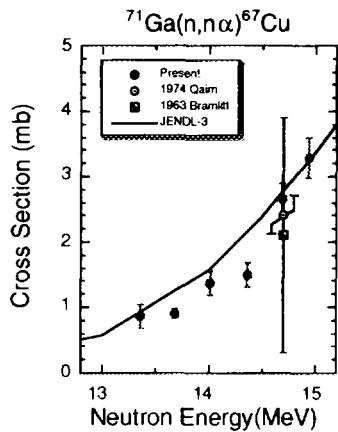
Fig.2.3 Cross section of ^{71}\text{Ga}(n,\alpha)^{67}\text{Cu} .
