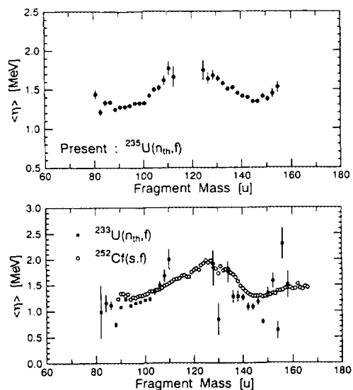
Fig.3 Average neutron energy \langle \eta \rangle(m^*)
