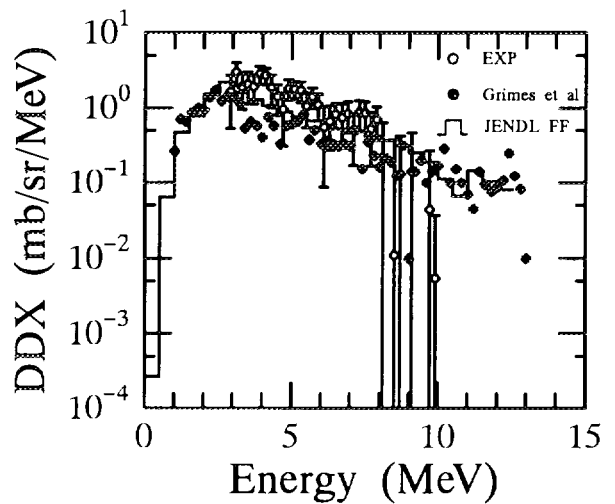
Fig.11 The DDX for V(n,xp) reaction at 70 degree compared with JENDL FF Grimes et al.
