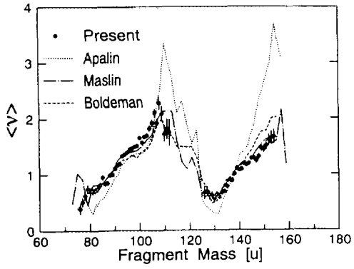
Fig.4 Average neutron multiplicity \langle \nu \rangle(m^*)
