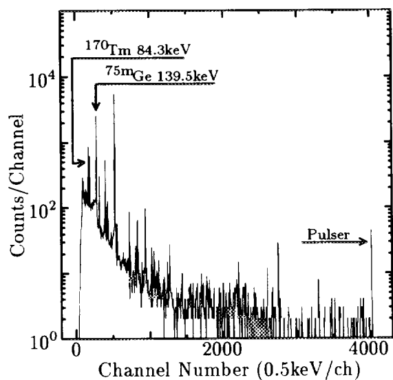
Fig. 1: Gamma-ray spectrum in the decay of ^{75m}\text{Ge} .
