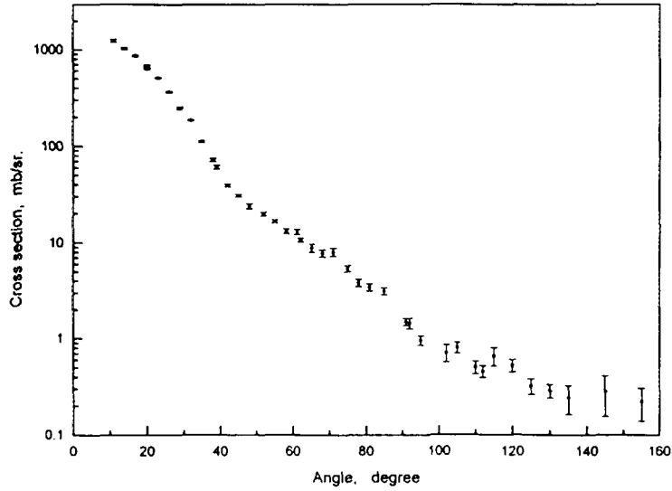
Fig. 8 Angular distribution of 37 MeV neutrons scattered from C
