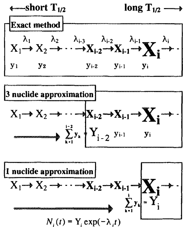
Fig. 2 Approximate summation method.
