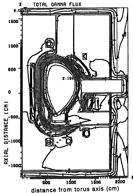
Fig. 5 Gamma-ray flux contour in ITER for the neutron first wall loading of 1\text{MW}/\text{m}^2
