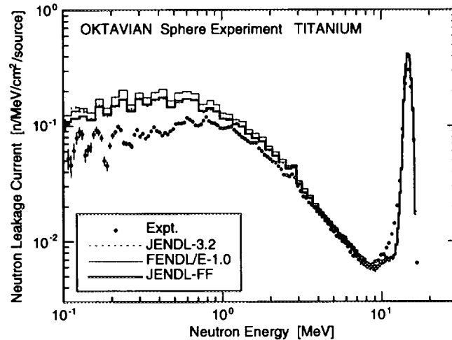
Fig. 2 Neutron energy spectra leaking from the titanium spherical pile measured at OKTAVIAN in comparisons with calculated ones by JENDL-FF, -3.2 and FENDL-1.
