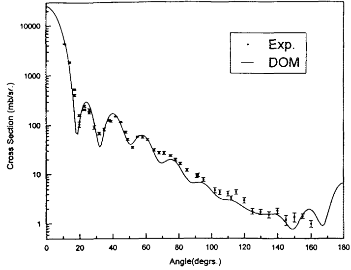
Fig. 7 Angular Distribution of 37 MeV Neutrons Scattered from Bi
