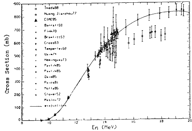
Fig. 10 Cross sections of ^{58}\text{Ni}(n,np+pn+d)^{57}\text{Co} reaction
