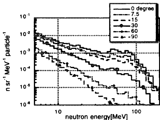
Fig.11: Neutron spectra from 100MeV/u carbon ions in a copper target.
