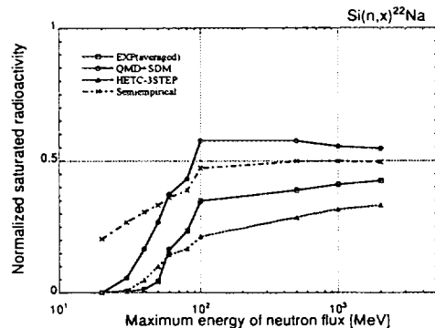
Fig.10 Normalized saturated radioactivity due to \text{Si}(n,x)^{22}\text{Na} reaction. The definition of normalized saturated radioactivity is shown by the equation (2). X-axis shows the maximum energy of neutron flux. Neutron flux is assumed to be proportional to 1/E . The activation cross sections for proton-induced reaction in Fig. 1 are used instead of neutron data.
