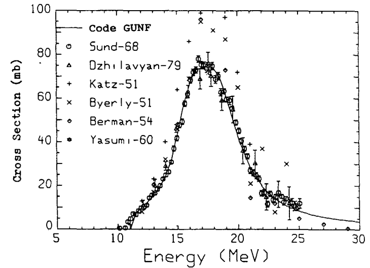
Fig. 26 Cross sections of 63 Cu(g,n) 62 Cu reaction
