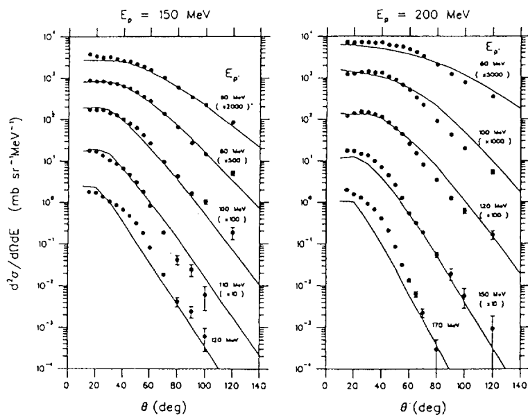
Fig.5 Comparisons of experimental angular distributions for ^{58}\text{Ni}(p,p') at two incident energies E_p and emission energies E_{p'} and results of MSD calculations (solid lines). The figures are taken from Ref. [5].
