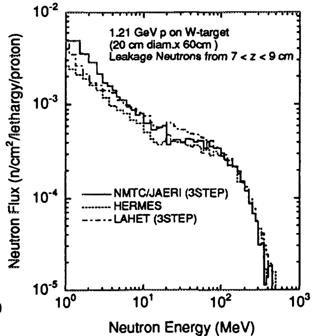
Fig. 2 Calculated neutron leakage spectra on the cylindrical surface at the position between 7 and 9 cm from the front surface of thick tungsten target bombarded with 1.21 GeV protons. The solid, dotted and dot-dashed lines indicate the calculated results of NMTC/JAERI-MCNP-4A, HERMES and LAHET, respectively.
