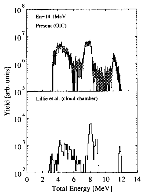
Figure 6: The energy spectra of ^{16}\text{O}(n,\alpha)
