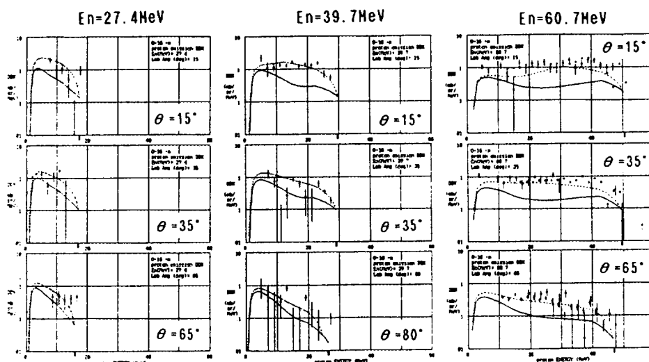
Fig.1 Proton DDXs of the O-16(n, xp) reaction : Comparison of the present calculation and the experimental data measured by Subramanian et al./2/. Solid line:modified EXIFON, Dashed line: modified EXIFOM + Quasi-free (n,p)
