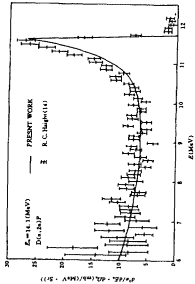
Fig. 20 Measured and evaluated double-differential cross sections for the D(n,p)2N reaction at 1.6 MeV
