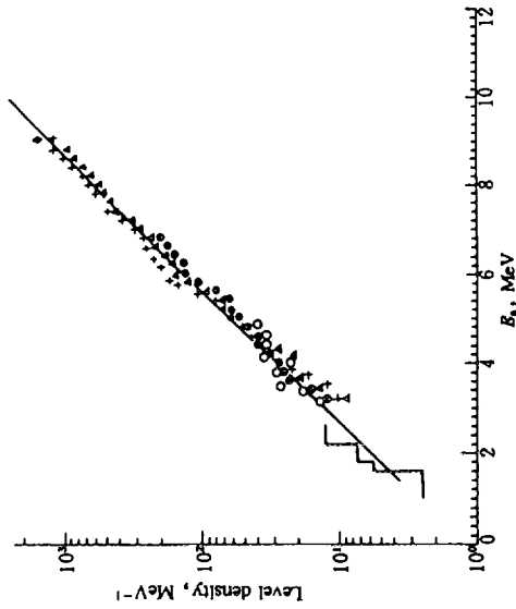
Fig. 13 Level densities of ^{59}\text{Ni} . \circ E_p = 9 MeV; \bullet E_p = 11 MeV; \blacktriangle E_p = 13 MeV; \blacktriangle E_p = 15 MeV; Histogram from Ref. [8]; \blacklozenge from s-wave neutron resonance spacing. Solid line: calculated, a = 6.3 , \delta = 1.0 , \sigma = 3.17 .
