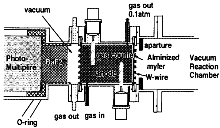
Fig. 8: Gas-BaF2 telescope
