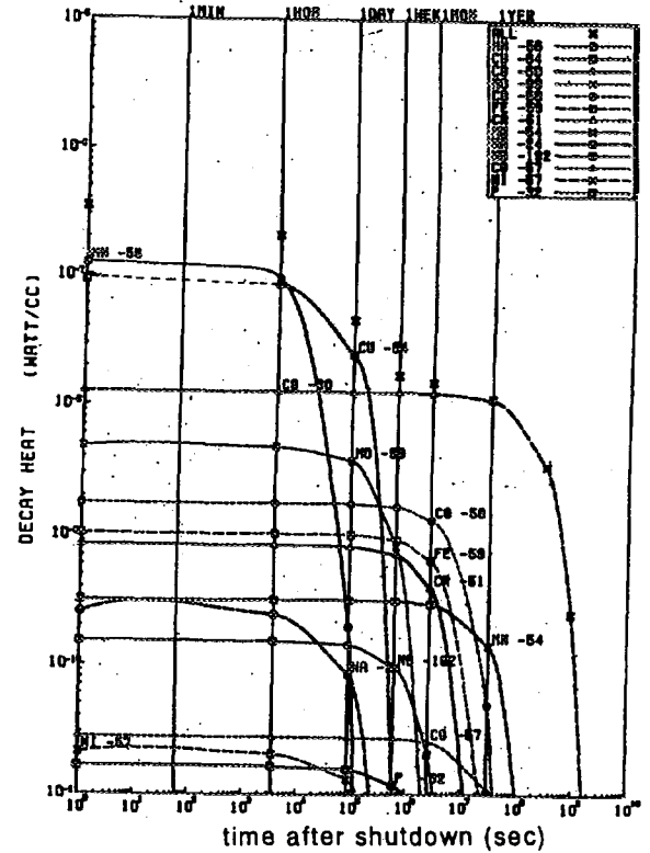
Fig. 13 Decay heat in inboard leg of toroidal coil in ITER
