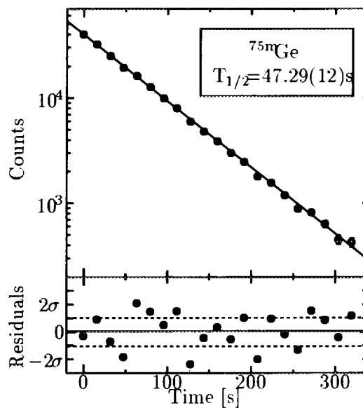
Fig. 2: Decay curve of ^{75m}\text{Ge} and residuals from a least squares fitting curve.
