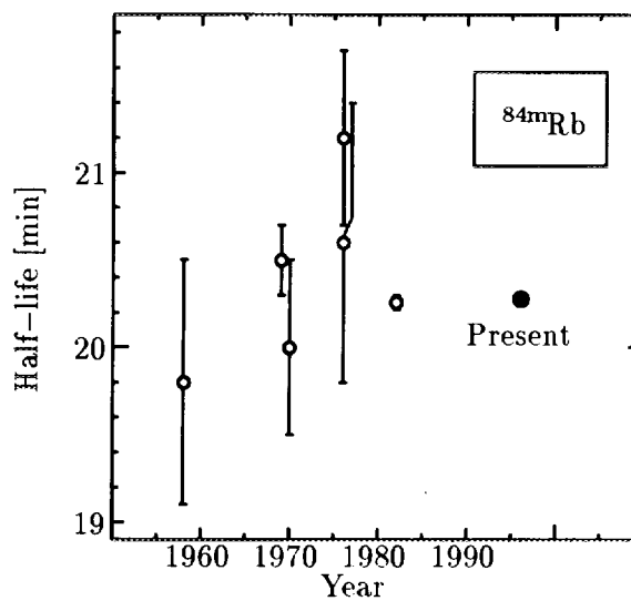
Fig. 4: Result of ^{84m}\text{Rb} and comparison with the previous works.
