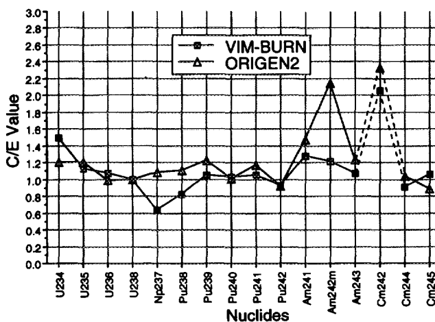
Fig.8 VIM-BURN and ORIGEN2 (High Burn-up UO 2 :54GWd/t)
