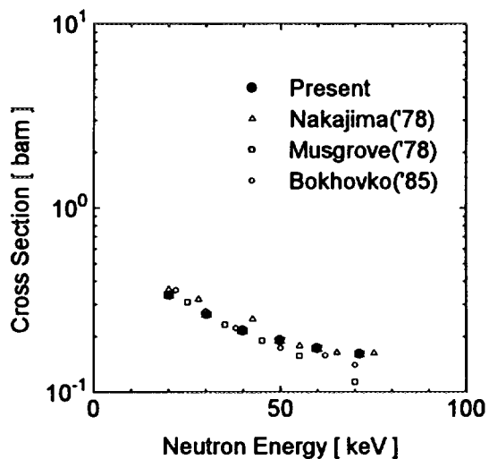
Fig. 4. Capture cross sections of ^{143}\text{Nd} .
