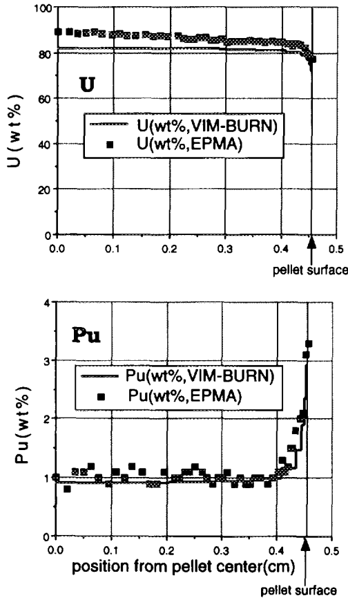
Fig.11 U and Pu distribution (High Burn-up UO 2 )
