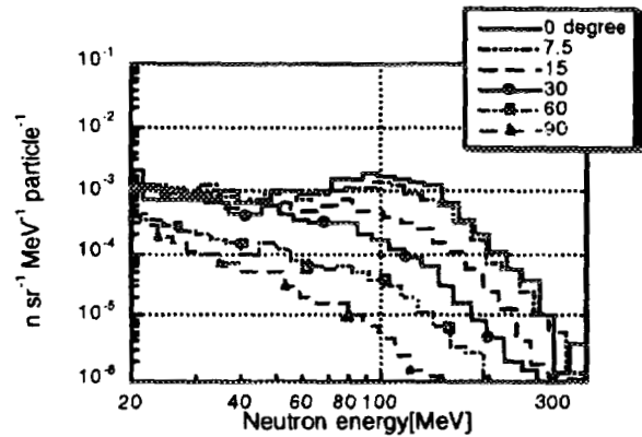
Fig. 8 : Neutron spectra from 180MeV/u carbon ions in a lead target.
