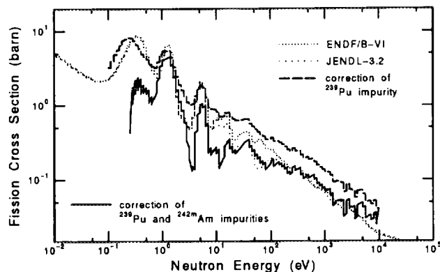
Fig. 3 Corrected cross section for the purchased ^{241}\text{Am} sample.
