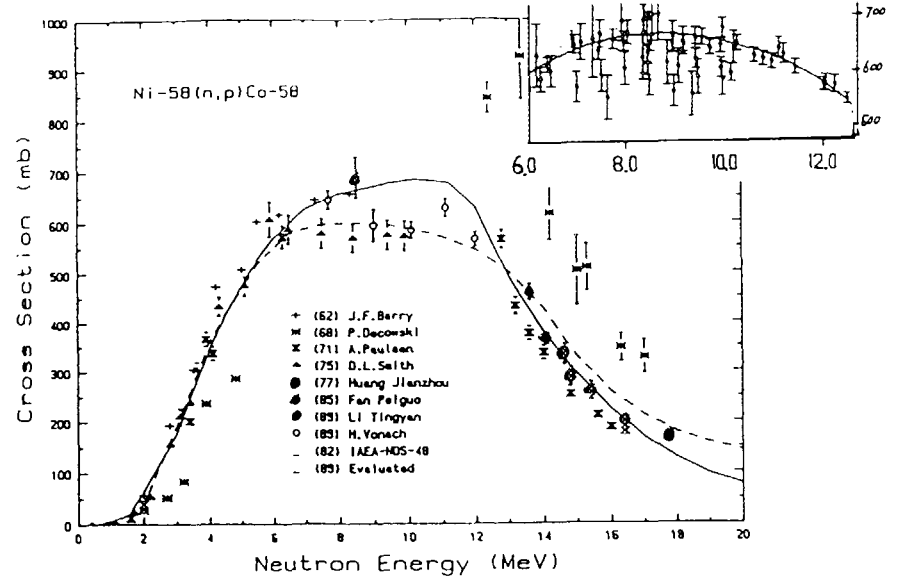
Fig. 9 Cross sections of ^{58}\text{Ni}(n,p)^{58}\text{Co} reaction
