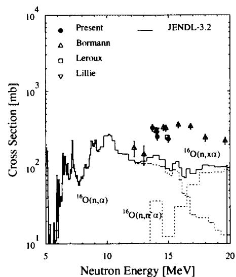
Figure 7: The ^{16}\text{O}(n,\alpha) cross section
