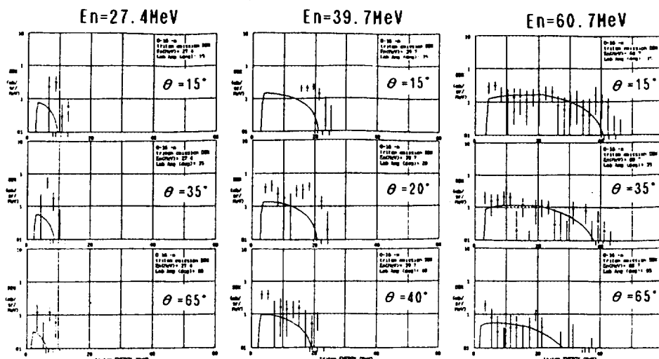
Fig.3 Triton DDXs of the 0-16(n,xt) reaction : Comparison of the present calculation and the experimental data measured by Subramanian et al./2/. Solid line:modified EXIFON
