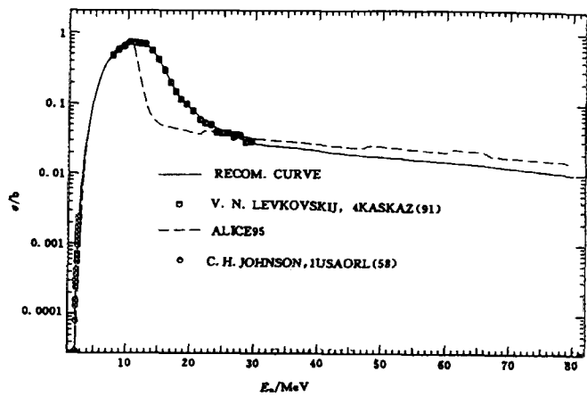
Fig. 24 Comparison of calculated 76 Se(p,n) cross section with exp. data
