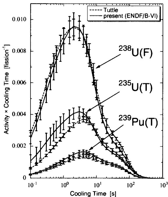
Fig. 5 Delayed neutron activity after a burst fission.
