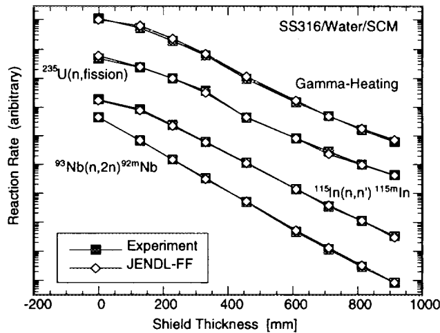
Fig. 6 Reaction rate distributions in the SS316/water/SCM assembly measured at FNS in comparisons with calculated ones by JENDL-FF.
