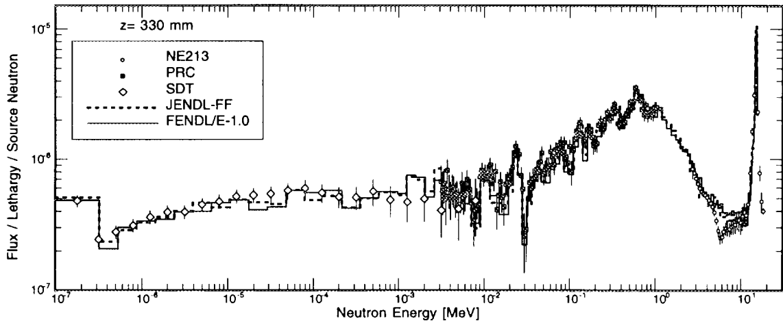
Fig. 5 Neutron energy spectra in the SS316/water shield assembly measured at FNS in comparisons with calculated ones by JENDL-FF and FENDL-1.
