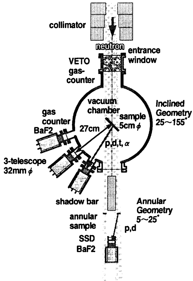
Fig. 9: Schematic view of the new spectrometer
