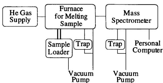
Fig. 2 HAFM Measurement System
