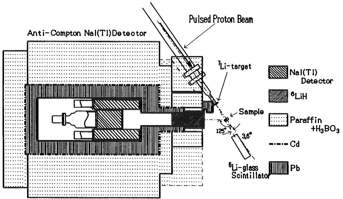
Fig. 1. Typical experimental arrangement.
