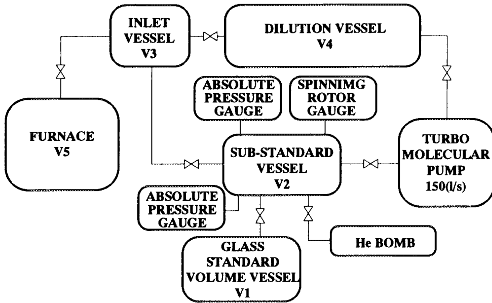
Fig.3. A block diagram of the standard helium supply.
