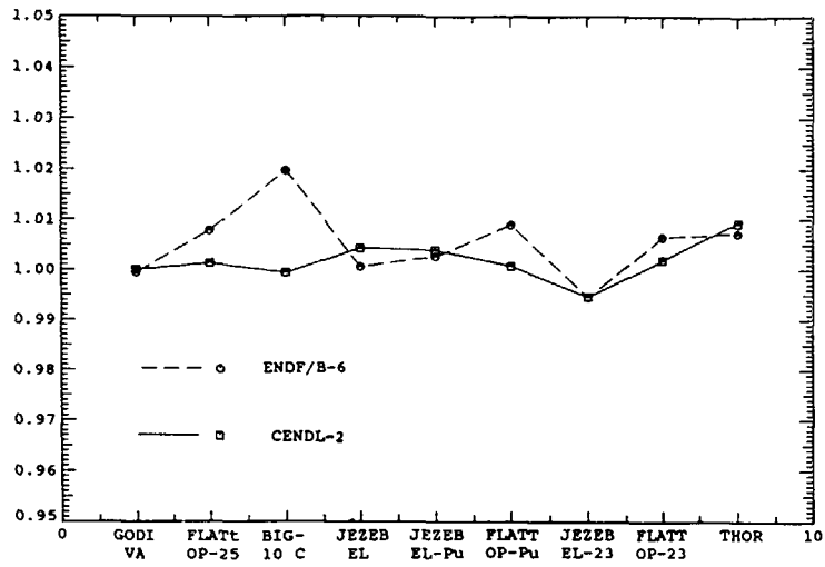
Fig. 23 K eff for homogeneous fast assemblies
