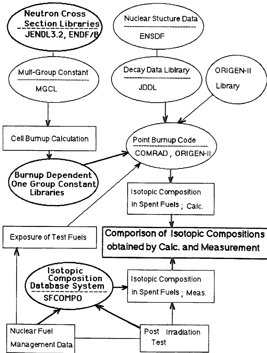
Fig. 1 Flow Diagram for Verification of Burnup Codes
