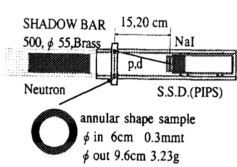
Fig. 3a: annular geometry
