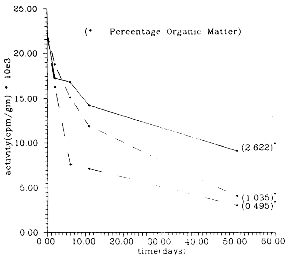
Fig 6. Dissipation of 14 C lindane in soils of different organic matter content.
