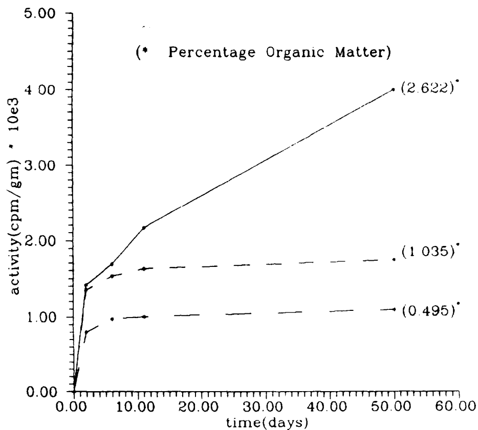
Fig 5. Bound residues of 14 C lindane in soils of different organic matter content.
