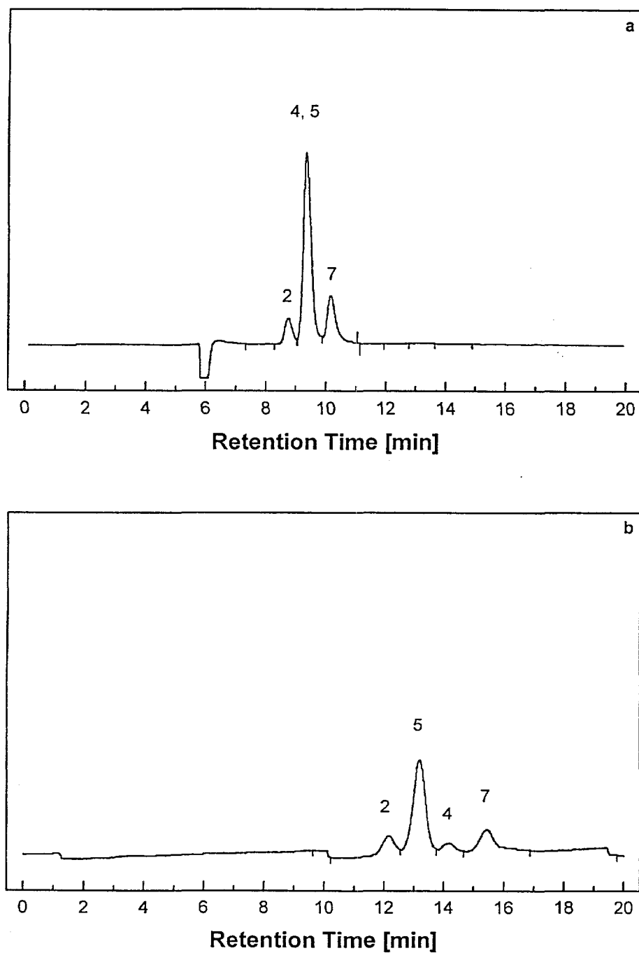
Figure 6. Sugar profiles of wet oxidised wheat straw (B91) after acid hydrolysis and purification as separated by: a) HPLC system 1 (HPX-87H column, 63°C, 0.004 M H 2 SO 4 , 0.6 mL/min.), b) HPLC system 2 (HPX-87P column, 81°C, water, 0.6 mL/min.). 2: Glucose; 4: Galactose; 5: Xylose; 7: Arabinose.
