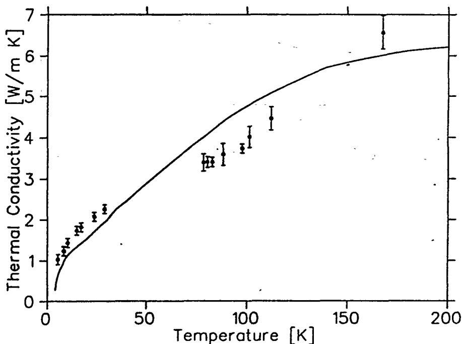
Figure 14: Measured conductivity of SOLEMI2 Nb_3Sn coil block. Solid line - Calculated values
