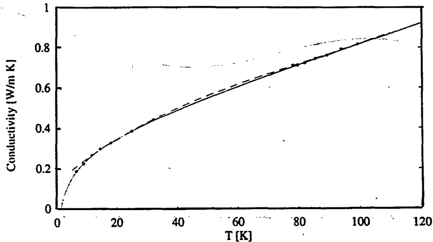
Figure 13: Measured conductivity of LASA5 Nb_3Sn coil. Solid line eq.(26). Dashed line - thermal conductivity determined with TCI fitting using an expansion to the third order.
