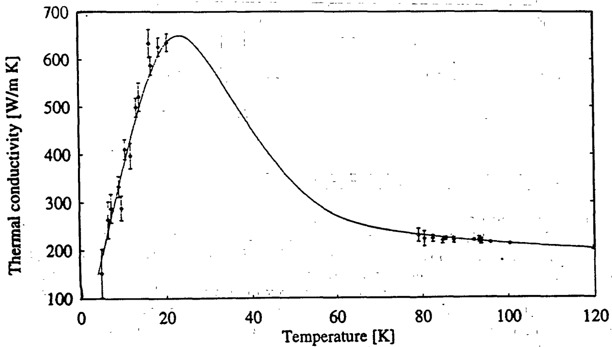
Figure 7: Tungsten thermal conductivity determined with the DAM method. The solid line is the NIST reference curve
