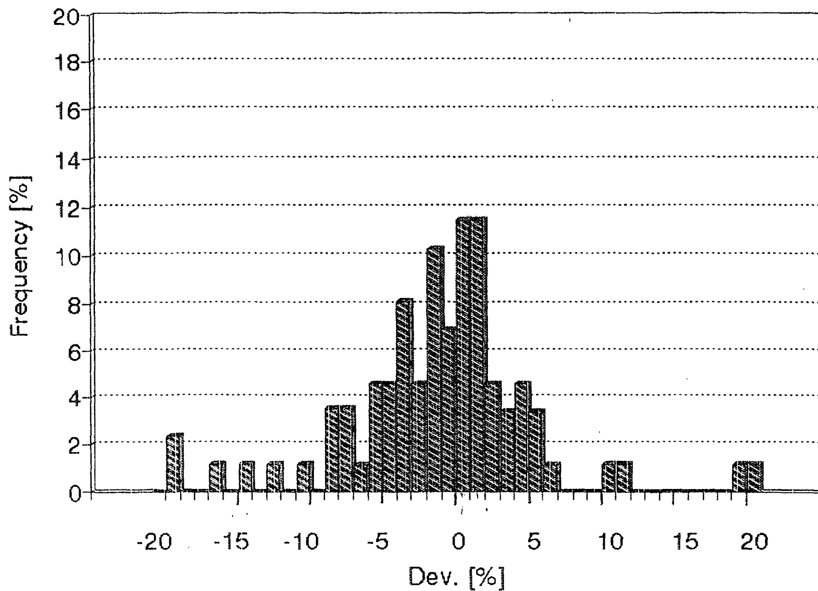
Figure 2. Results of RRC TLD service for cobalt 60 therapy units. Second participation (year 1982 to 1983).
