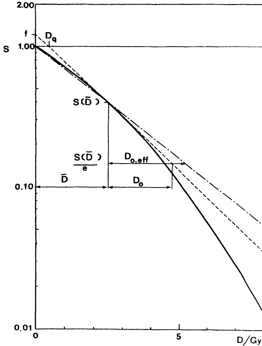
Fig. 2 Comparison of different cell survival curve models. The solid line curve is the linear quadratic relation whereas the dashed line corresponds to a tangent and the dash dotted a secant through the mean dose per fraction.
