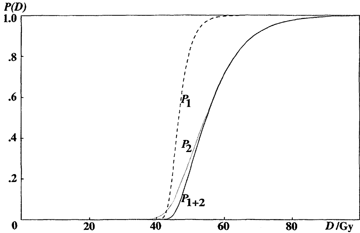
Figure 3 The dose-response relationship for a heterogeneous tumor P_{1+2} consisting of 10^8 'normal' tumor cells with D_0 = 2.5 Gy and 10^3 hypoxic cells with D_0 = 7.5 Gy ( OER = 3 ) with a dose response according to curves P_1 and P_2 respectively. It is seen that the few resistant hypoxic cells lower the slope of the dose-response relationship to a value almost as low as that of the most resistant cell fractions.
