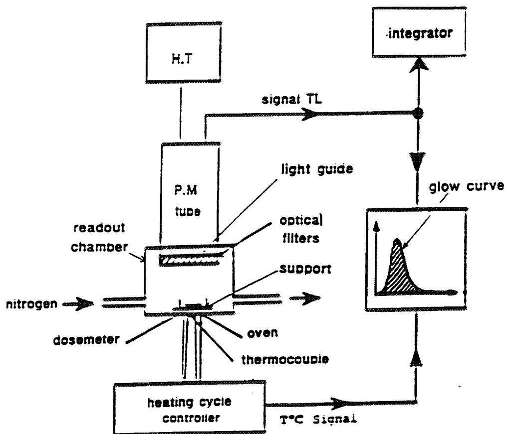
Fig. 4. Principle of a TL reader. After [8].
