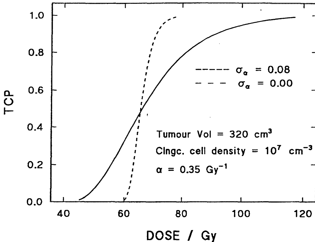
Figure 2. Tumour Control Probability (TCP) as a function of target dose, derived from Eqs 5 and 6, with a = 0.35 , r_{cl} = 10^7 for a 320 cc volume, for s_a = 0.0 and for the clinically more realistic s_a = 0.08 (adapted from [12]).
