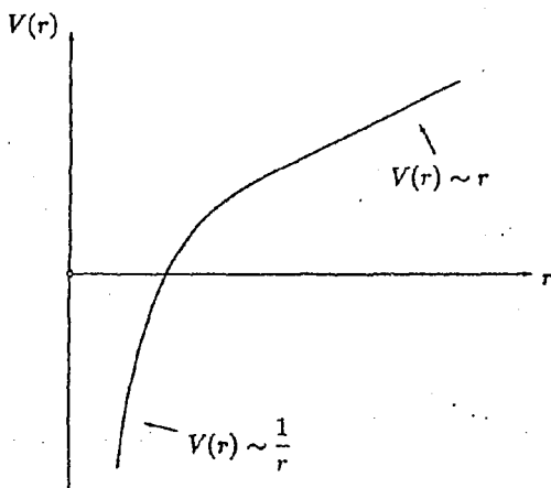
Figure 3.1: Funnel potential.
