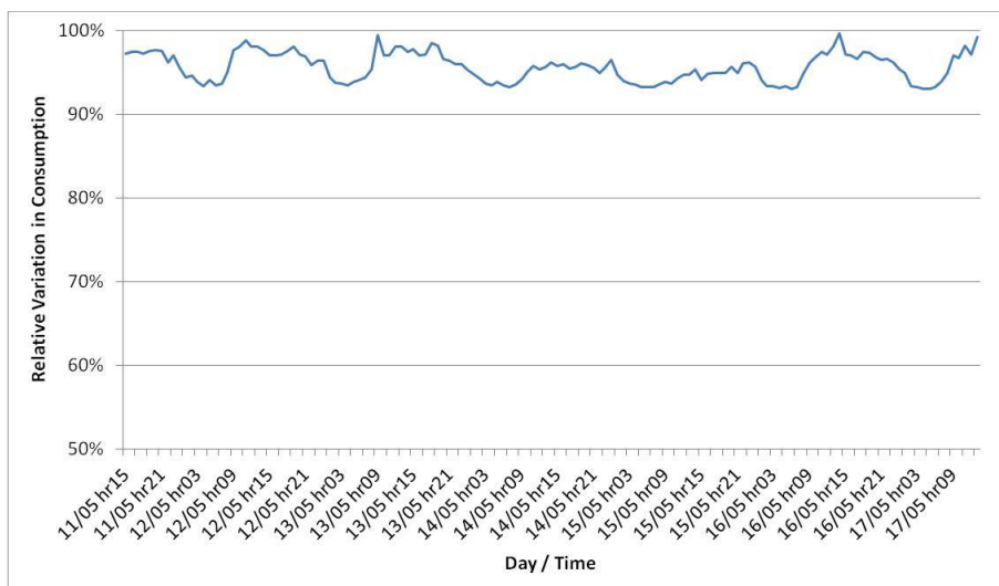
Figure A.4 – Relative variation in power consumption for the urban site. Values are normalized against a maximum value based on the rated power of the equipment.
