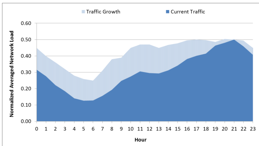
Figure 7.21 – Traffic profile (dark shade) based on traffic statistics extracted from a real network. The traffic is normalized against an assumed maximum of 50% traffic load. The striped area depicts the potential of accommodating traffic growth during different hours. Traffic profile based on [43].
