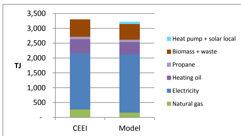
Figure 18: Comparison of 2010 CEEI and BAU residential consumption figures for the CVRD.
