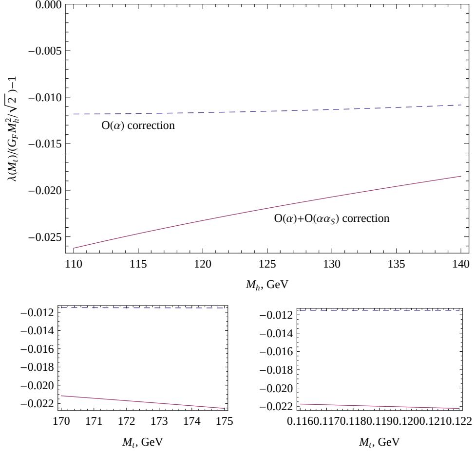
Figure 10: Contributions to the Higgs self coupling constant of the order O(\alpha) and O(\alpha) + O(\alpha\alpha_s) . One parameter is varying, the two others are chosen from M_t = 172.9 \text{ GeV} , \alpha_s = 0.1184 , M_h = 125 \text{ GeV} .
