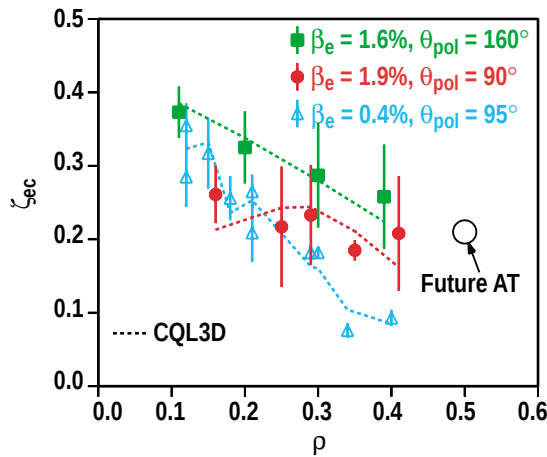
Fig. 3. Experimental dimensionless ECCD efficiency for co injection for scans of the normalized radius of deposition in low beta L-mode and high beta H-mode plasmas. The theoretical dependence calculated by the CQL3D code is also shown (dashed lines).
