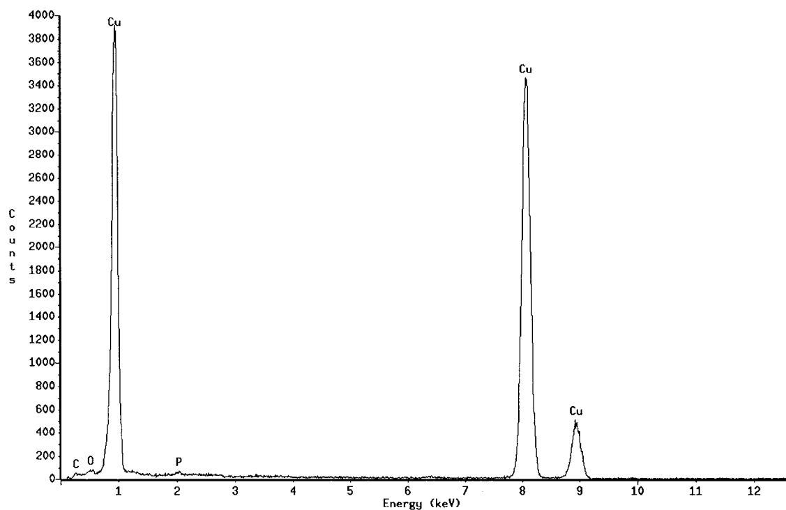
Fig 31. EDS results of the matrix outside the thinned zone in Fig 28a, showing attenuated concentration of P, O and C in comparison with the zone and the boundary film.
