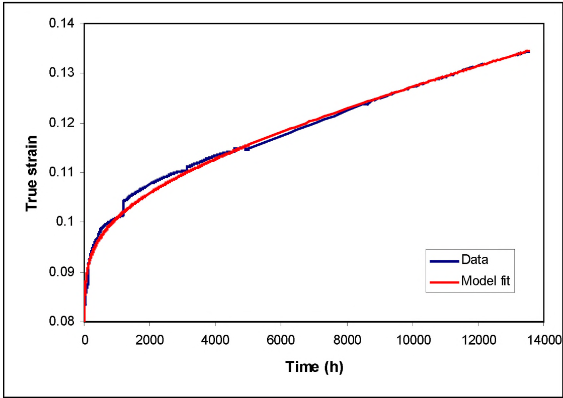
Fig 7. The uniaxial creep curve at 120 MPa/150°C (test V1), and fitted curve using model where total strain is a sum of initial "instantaneous" strain, primary creep strain and steady state strain components: \epsilon = \epsilon_0 + \epsilon_P + \epsilon_S .
