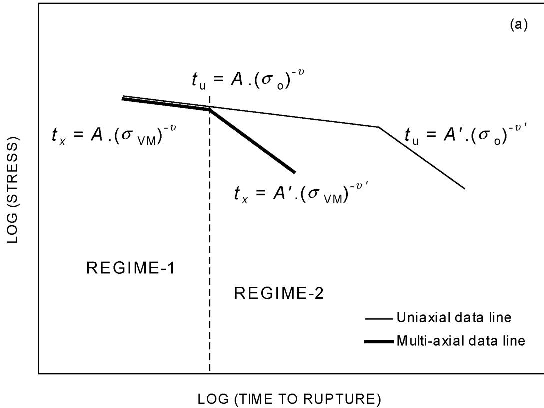
Fig. 4. The principle on shortening of creep life by damage in multiaxial loading. Creep life is described by the simple inverted Norton expression (at constant temperature). Here subscript u refers to uniaxial and subscript x to multiaxial loading; subscript VM refers to v. Mises equivalent stress and subscript o to plain uniaxial case. Regime 2 is the region where grain boundary cavitation can dominate creep damage.
