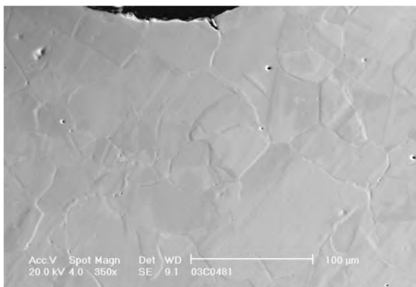
Fig 25. Specimen CT-3 side surface after 10300 h of testing, notch tip on the upper side; a) notch tip area with a partly opened grain boundary, electrolytic polish; b) detail of the same region after mechanical polish and slight etch.
