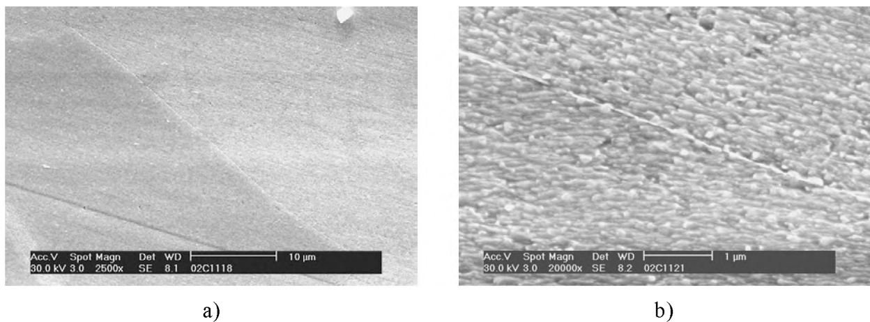
Fig 15. Microstructure of the as-received material after electropolish and slight etch; a) grain boundaries and b) detail of a grain boundary as it can be seen in SEM.
