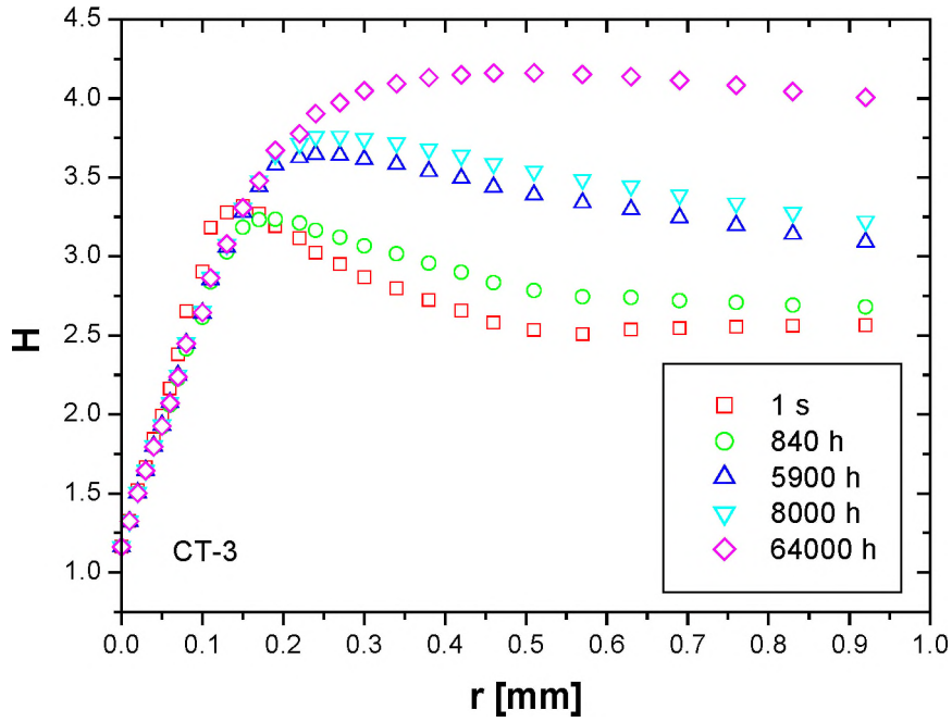
Fig. 13. Evolution of H distribution in front of the notch tip for specimen CT-3 at different times during a simulated test. The case of 64000 h corresponds to a stabilised situation.
