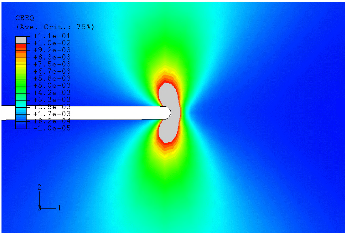
Fig. 11. Distribution of the predicted equivalent creep strain for specimen CT-3 at 64000 h.
