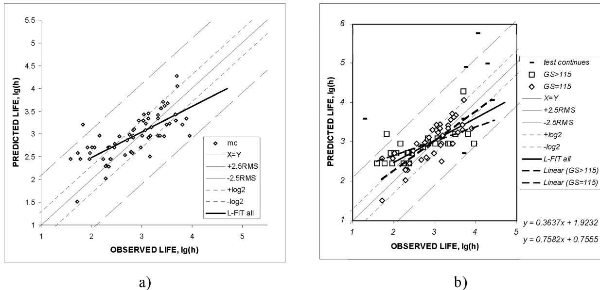
Fig. 33. Comparison of predicted and observed uniaxial creep rupture life from available data (best fit with MC parametric model). The fitted (least squares) line includes only test data > 100 h; a) all data; b) effect of grain size (GS).
