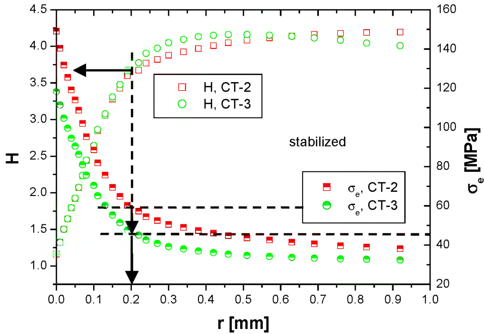
Fig. 14. Distributions of the stabilised values of H and v. Mises equivalent stress \sigma_e in front of the notch tip for specimens CT-2 and CT-3. At the corresponding values of reference stress of 59 MPa (CT-2) and 46 MPa (CT-3), the distance from the notch tip is 0.2 mm.
