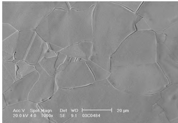
Fig 27. Specimen CT-3 side surface after 10300 h of testing, about 0.2 mm below the notch tip; electrolytic polish and slight etch; a) grain boundary with a cavity (arrow); b) magnification of the same cavity indication; note the film-like feature crossing the boundary region at the cavity indication.
