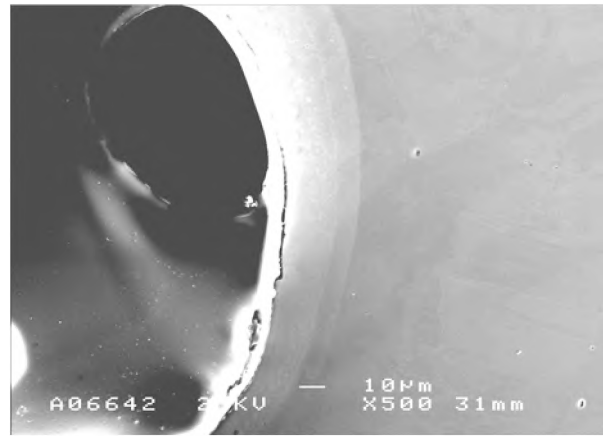
Fig 18. Specimen CT-2 (150 °C/59 MPa) side surface after 1003 h of testing, electrolytic polish, no etch; a) general view near the notch tip; b) magnification of the tip root area.
