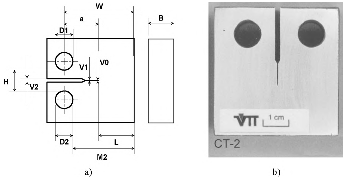
Fig. 3. a) The compact tension (CT) specimen for multiaxial creep testing; the dimensions W , B , a/W and V0 are given in the text, b) specimen CT-2 before testing
