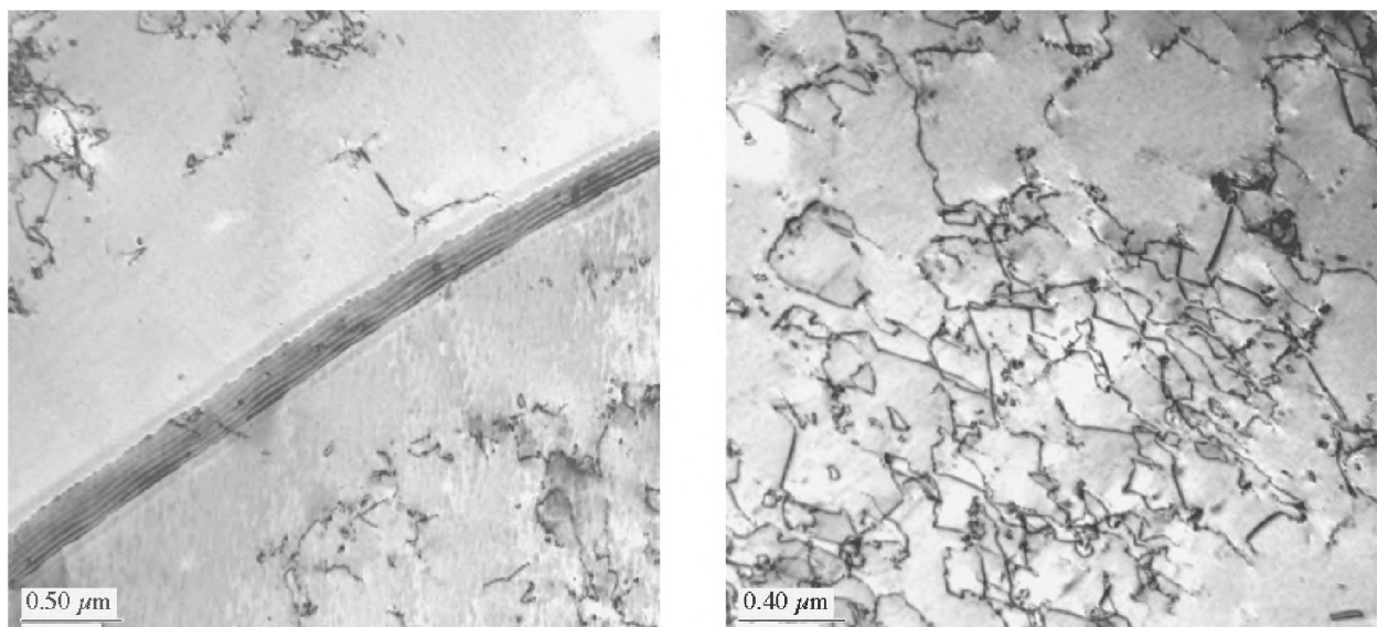
Fig 15. Microstructure of the as-received material after electropolish and slight etch; a) grain boundaries and b) detail of a grain boundary as it can be seen in SEM.
