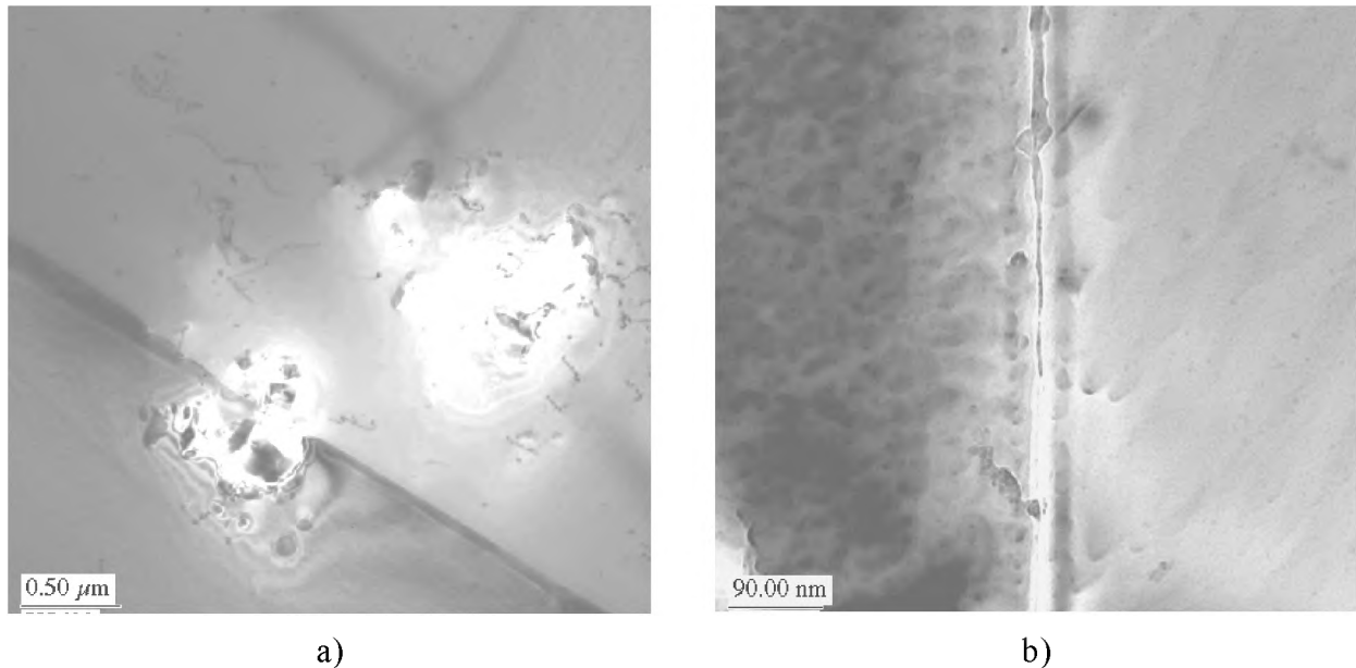
Fig 17. a) CuS inclusions appear in groups, some in grain boundaries; b) film with high oxygen and phosphorus content on a grain boundary of the as-received material (TEM).
