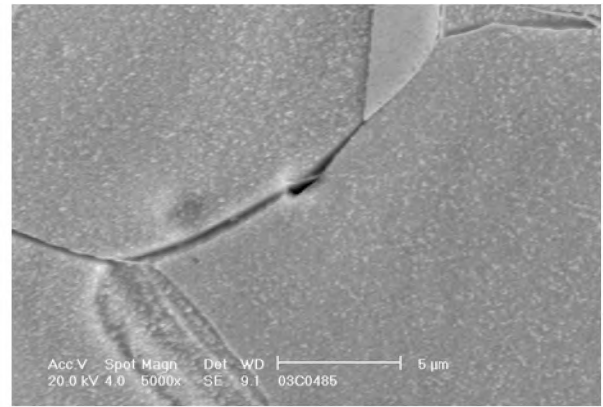
Fig 27. Specimen CT-3 side surface after 10300 h of testing, about 0.2 mm below the notch tip; electrolytic polish and slight etch; a) grain boundary with a cavity (arrow); b) magnification of the same cavity indication; note the film-like feature crossing the boundary region at the cavity indication.
