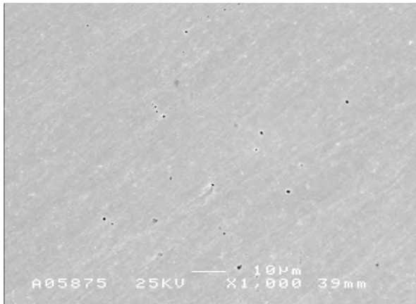
Fig 19. Specimen CT-2 (150 °C/59 MPa) side surface after 1003 h of testing; mechanical polish, no etch; a) region near the notch tip, showing cavity-like indications; b) typical area with no cavity indications.
