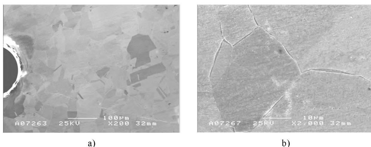
Fig 22. Specimen CT-3 side surface after 5018 h of testing, electrolytic polish and slight etch; a) notch tip region; b) magnification below the tip root area. Note the structure of some grain boundaries, suggesting an additional phase.
