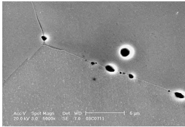
Fig 26. Specimen CT-3 mid-section after 10300 h of testing; a) gb cavity indications near the notch tip; b) a cavity indication in a low stress region (ligament side corner).
