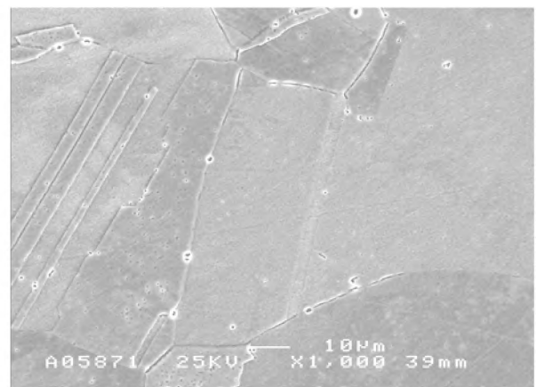
Fig 20. The side surface of specimen CT-2 (150 °C/59 MPa) after 1003 h of testing, with ferric chloride etch; a) notch tip region; b) several mm away from the tip. Note relatively abundant false cavity indications on grain boundaries and elsewhere.
