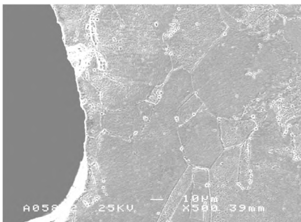
Fig 20. The side surface of specimen CT-2 (150 °C/59 MPa) after 1003 h of testing, with ferric chloride etch; a) notch tip region; b) several mm away from the tip. Note relatively abundant false cavity indications on grain boundaries and elsewhere.
