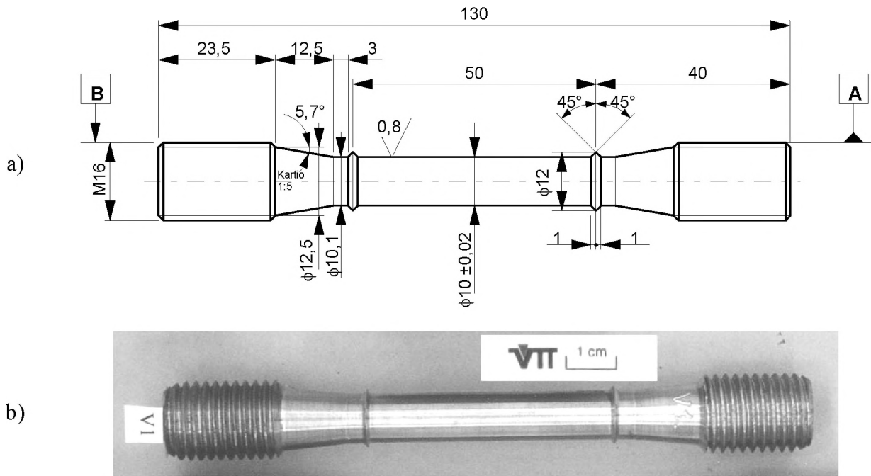
Fig. 2. a) dimensions and b) actual specimen (V1) for the uniaxial creep testing.
