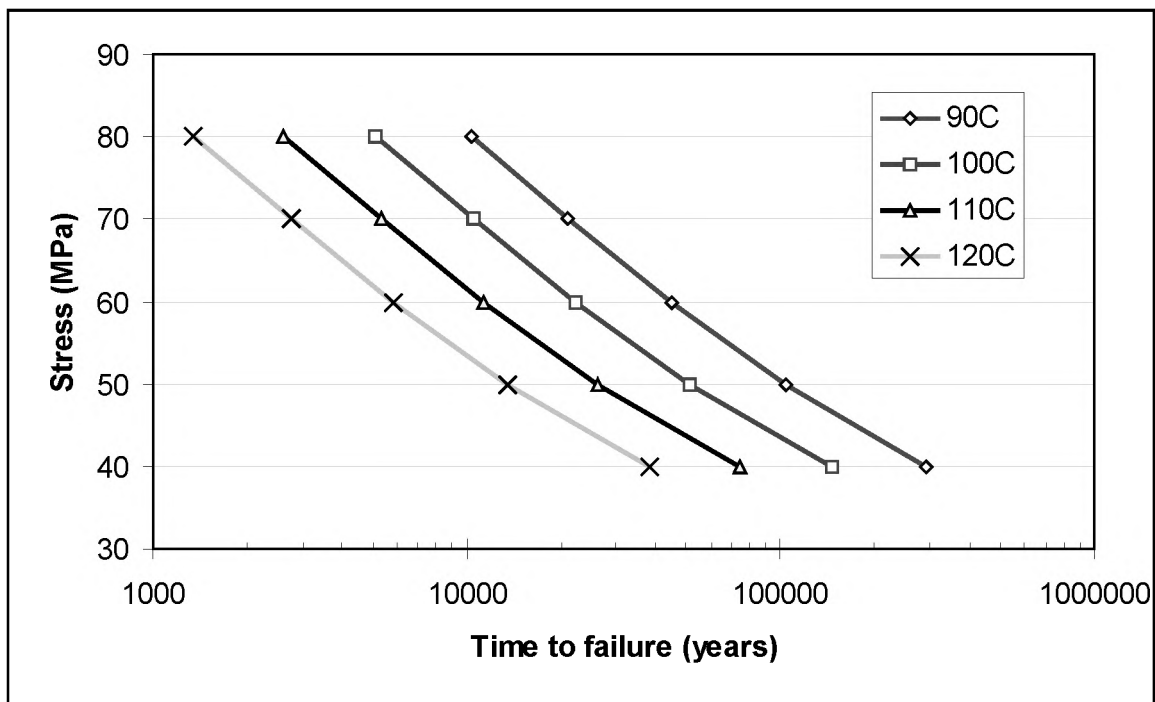
Fig 35. The predicted isothermal uniaxial creep life from the MC expression (eq. 6) for a range of 90-120 °C / 40-80 MPa.
