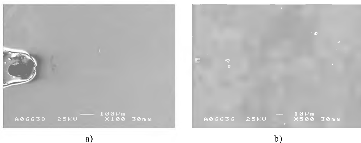
Fig 21. Specimen CT-3 (150 °C/46 MPa) side surface after 3000 h of testing, electrolytic polish; a) general view near the notch tip; b) magnification below the tip root area.
