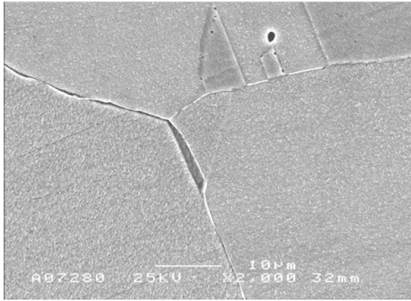
Fig 23. Specimen CT-3 side surface after 5018 h of testing, electrolytic polish and slight etch; a) grain boundary (gb) phase; b) gb phase, detail.
