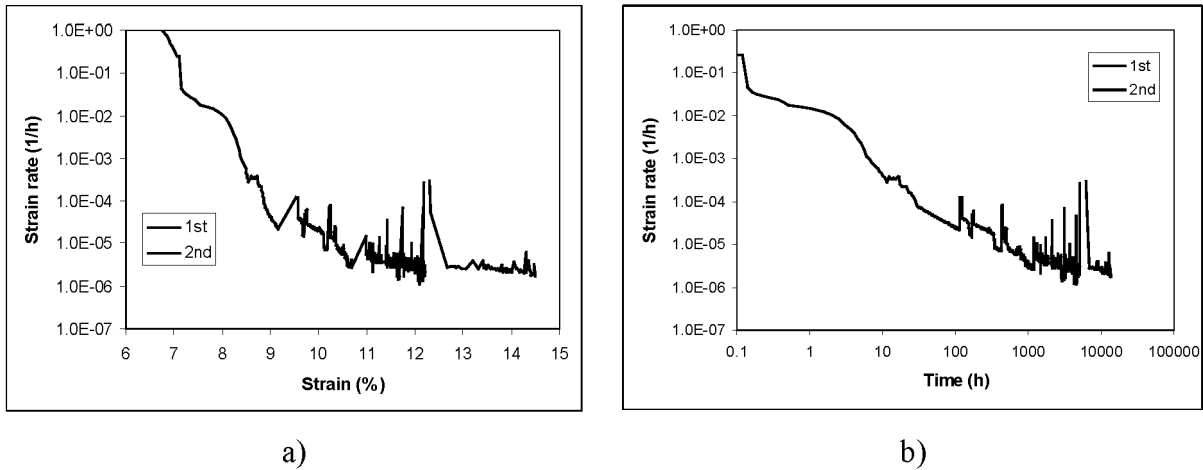
Fig. 6. Strain rate in the test (V1) of Fig 5, as a function of a) strain and b) time. The 1st and 2nd phases refer to the curve sections before and after interruption at 5011 h.
