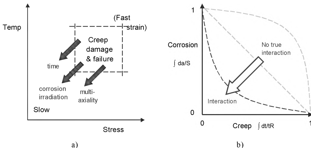
Fig 36. a) Additional potential or likely factors promoting creep and creep damage; b) types of interaction between damage mechanisms (example on corrosion and creep).
