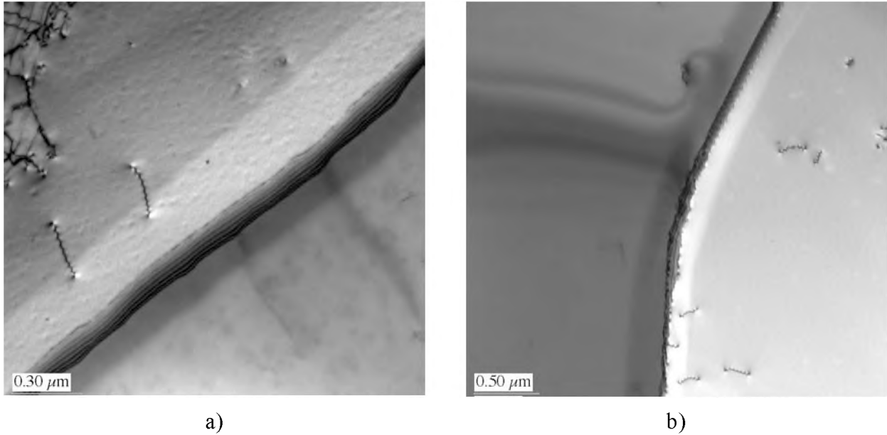
Fig 32. CT-3 after 10300 h, notch root mid-section, two TEM images showing thinned "segregation zones" along grain boundaries, with dislocations crossing the zone-matrix boundary.
