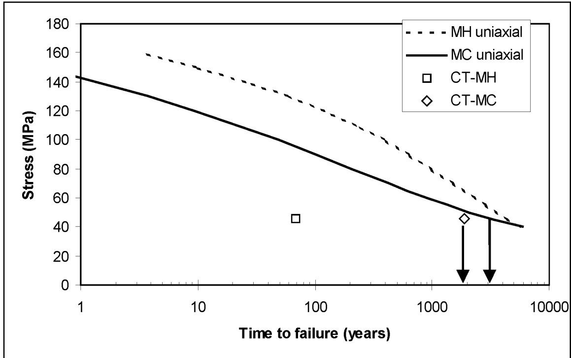
Fig 34. The estimated uniaxial creep life at 150 °C/46 MPa from the multiaxial test (CT-MH) in comparison with the predicted life from the MH expression of Lindblom et al (1995, MH uniaxial), and the corresponding comparison from the same multiaxial test (CT-MC) and from the MC expression of the present work (MC uniaxial). The latter pair gives the values of predicted life within a factor of two at 46 MPa.
