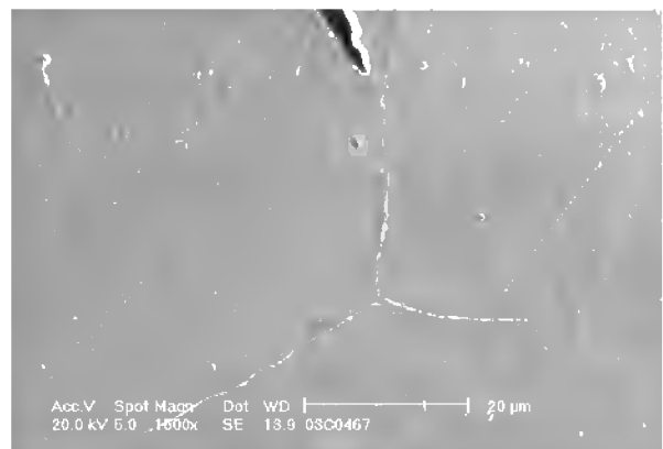
Fig 25. Specimen CT-3 side surface after 10300 h of testing, notch tip on the upper side; a) notch tip area with a partly opened grain boundary, electrolytic polish; b) detail of the same region after mechanical polish and slight etch.
