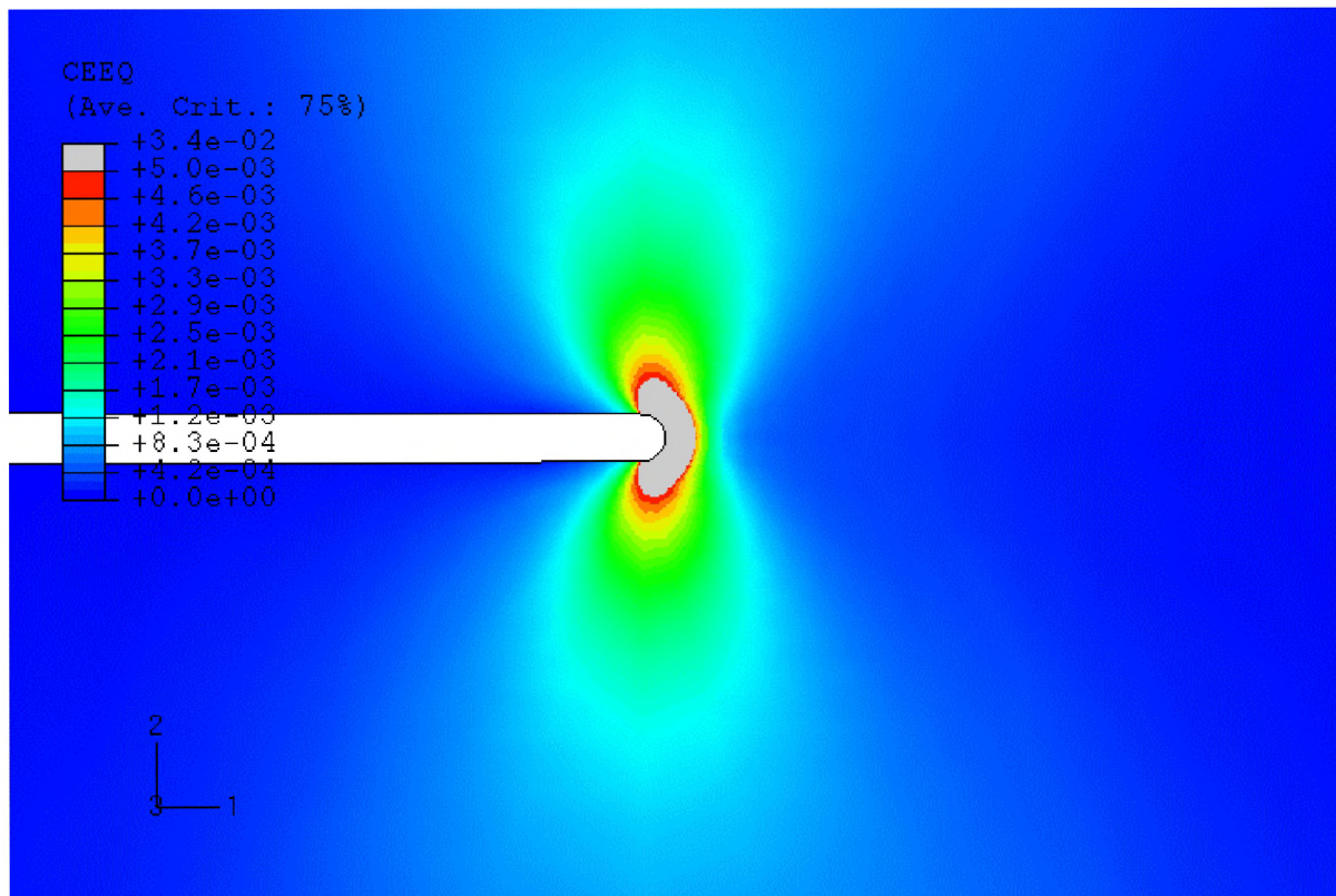
Fig. 10. Distribution of the equivalent strain for the specimen CT-3 at 6000 h.
