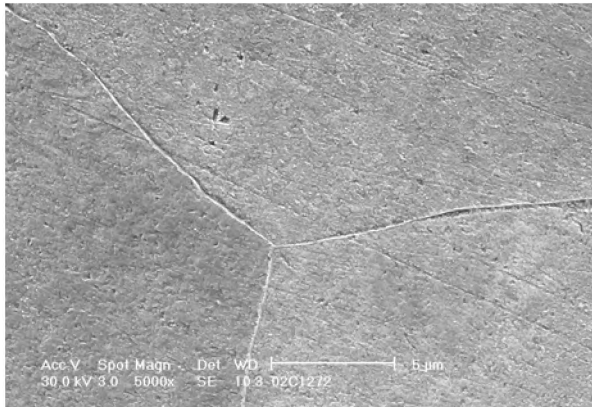
Fig 24. Specimen CT-3 side surface after 7900 h of testing, electrolytic polish and slight etch; a) grain boundaries; b) a cavity indication on a grain boundary.
