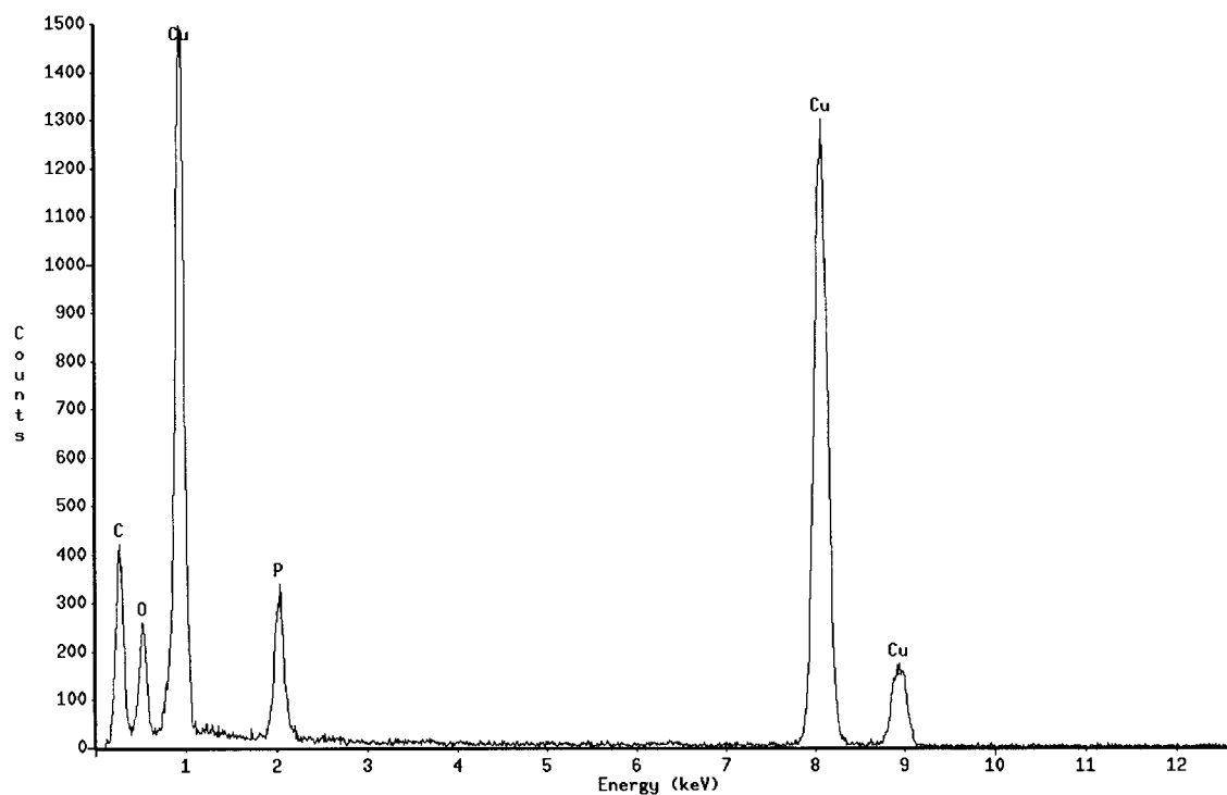
Fig 30. EDS results of the grain boundary film of Fig 28a, showing elevated concentration of P, O and possibly C at somewhat higher level than in the thinned zone (Fig 29).
