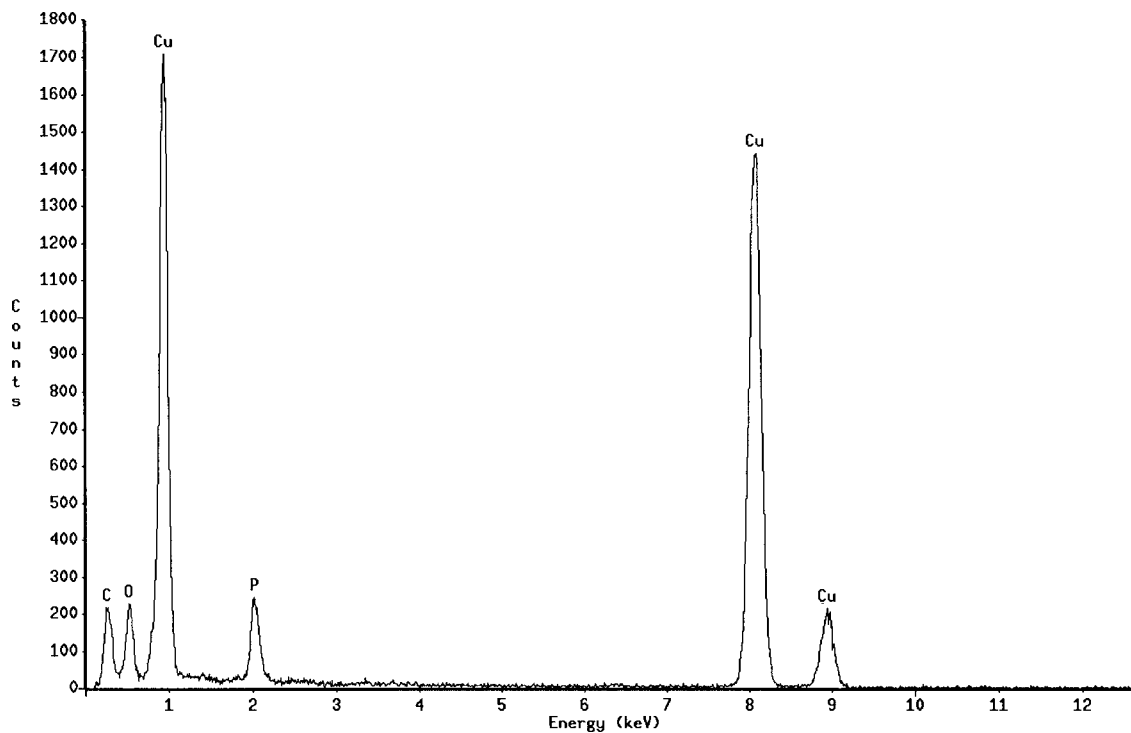
Fig 29. EDS analysis results of the thinned region adjacent to the grain boundary from Fig 28a, showing elevated concentration of P, O and possibly C (note that some indicated carbon is expected as a electron beam contaminant).
