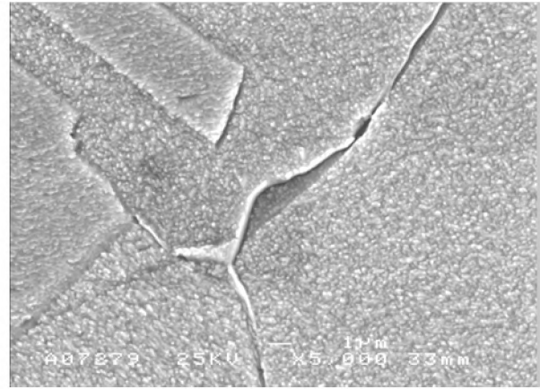
Fig 23. Specimen CT-3 side surface after 5018 h of testing, electrolytic polish and slight etch; a) grain boundary (gb) phase; b) gb phase, detail.
