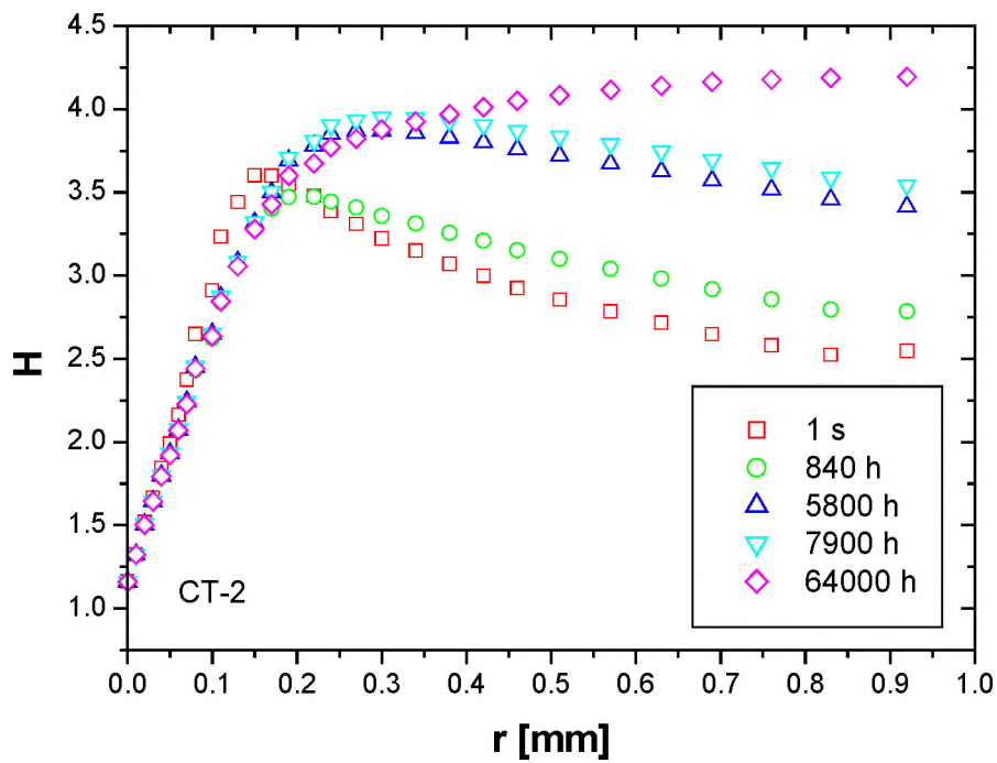
Fig. 12. Evolution of H distribution in front of the notch tip for specimen CT-2 at different times during a simulated test. The case of 64000 h corresponds to a stabilised situation.
