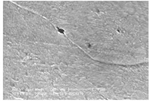
Fig 24. Specimen CT-3 side surface after 7900 h of testing, electrolytic polish and slight etch; a) grain boundaries; b) a cavity indication on a grain boundary.
