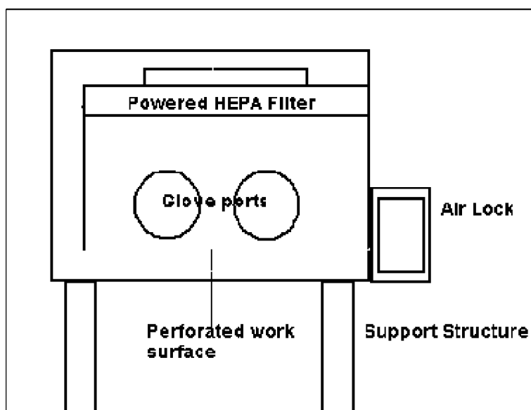
FIG. 1. Glove box.
