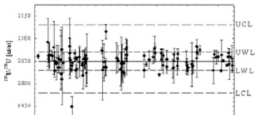
FIG. 2. Results of loading blank measurements of 233 U enriched spike IRMM 04/01 on the Finnigan MA T262.
