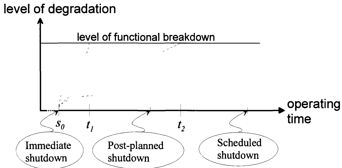
Figure 10. Time points related to the operational maintenance decision options and realisations of the failure time ( t_1 , t_2 ) measured from the time of observation of an incipient failure ( s_0 ).
