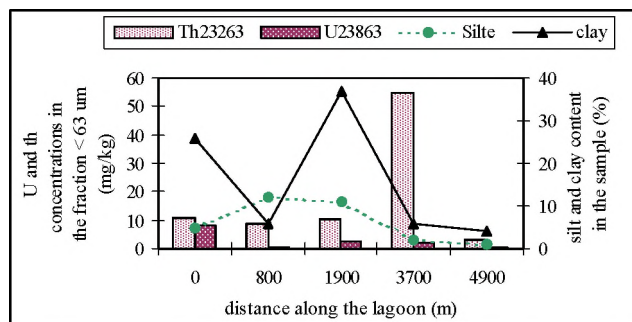
Figure 9. Distribution of U and Th in the fraction < 63 μm of the sediment.
