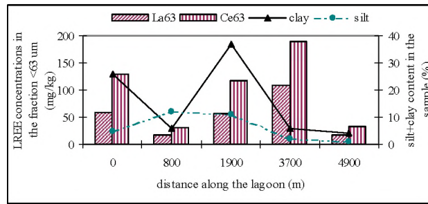
Figure 7. Distribution of LREEs in the fraction < 63 μm of the sediment.
