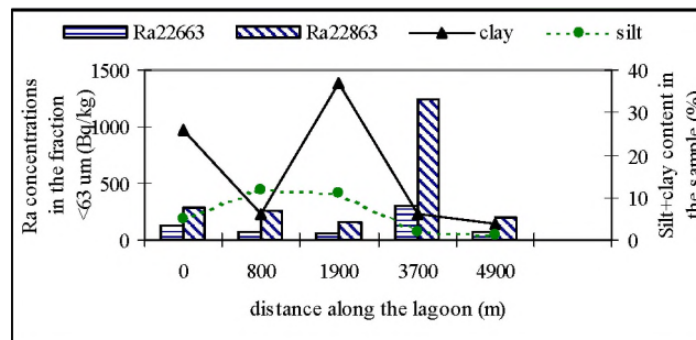
Figure 8. Distribution of radium isotopes in the fraction < 63 μm of the sediment.
