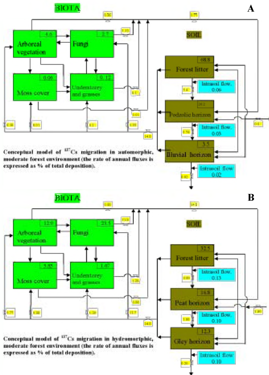
Fig. 5. Conceptual models of ^{137}\text{Cs} migration in forest environments in autormorphic (A) and hydromorphic (B) areas (30-km exclusion zone, 1998).
