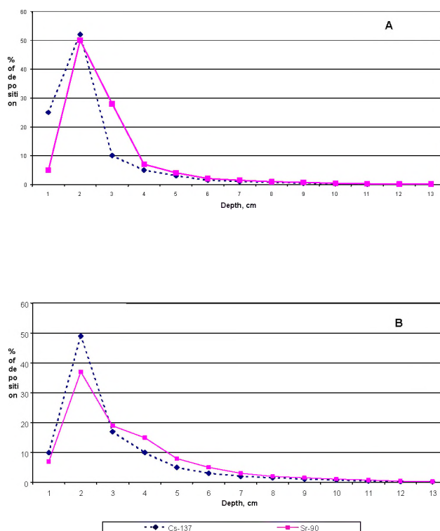
FIGURE 4. Vertical distribution of 137 Cs and 90 Sr in (A) automorphic and (B) hydromorphic soils. Key plots 1 and 2, respectively (1998).
