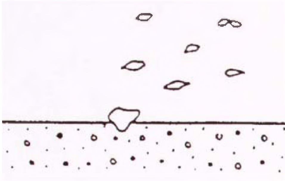
FIG. 2.20. Pop-out due to reactive aggregate and high humidity.
