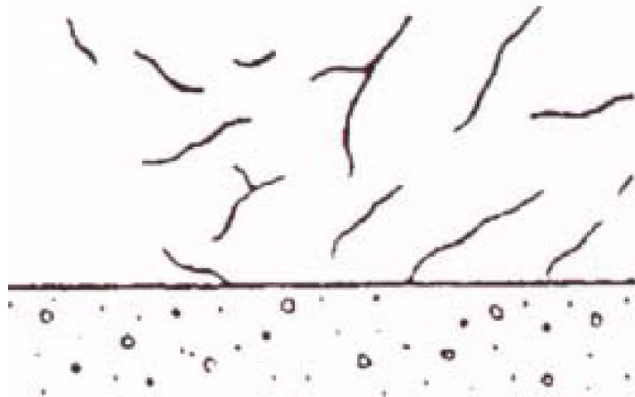
FIG. 2.13. Cracks due to abnormal set of cement.
