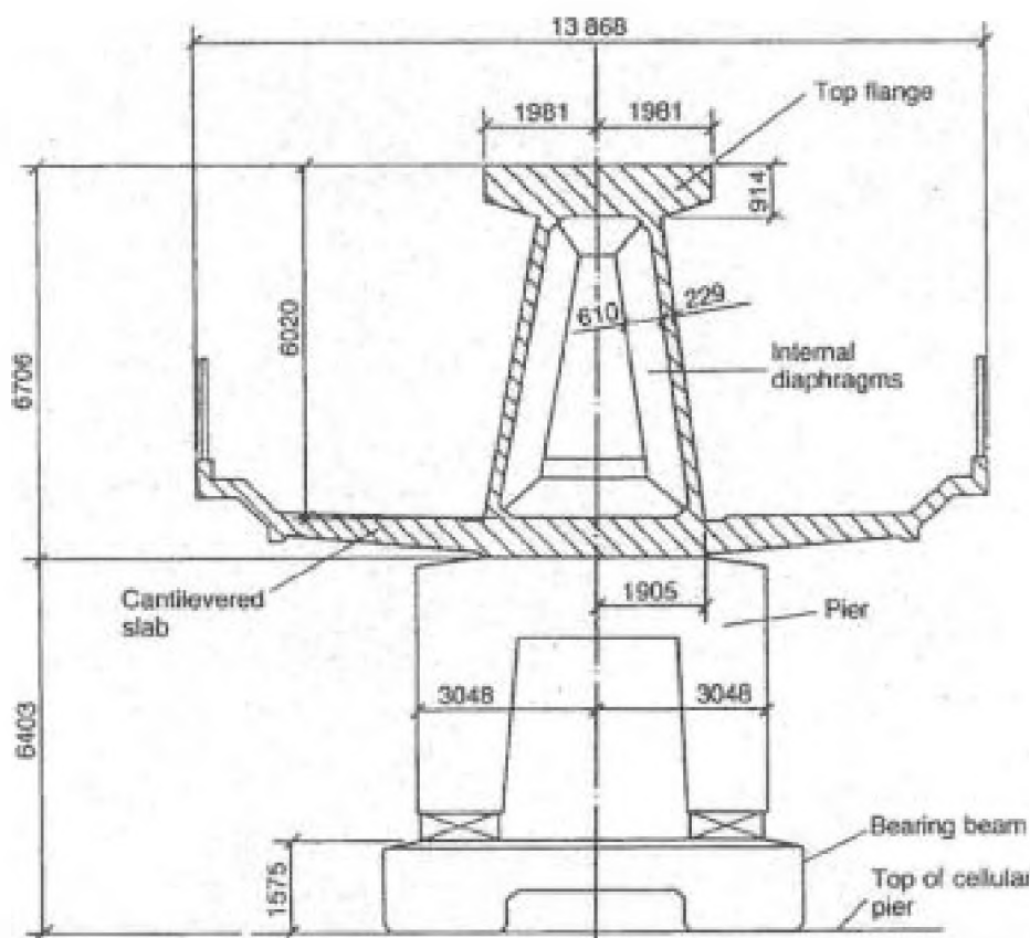
FIG. 17.12. Cross-section of Besses o' th' Barn Bridge.
