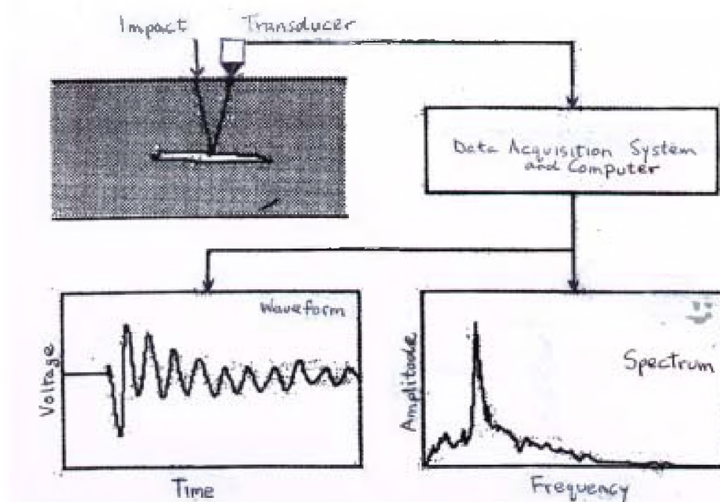
FIG. 11.9. Schematic diagram showing how impact-echo works.
