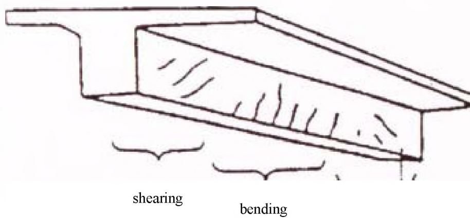
FIG. 2.10. Cracks due to bending and shear stresses.
