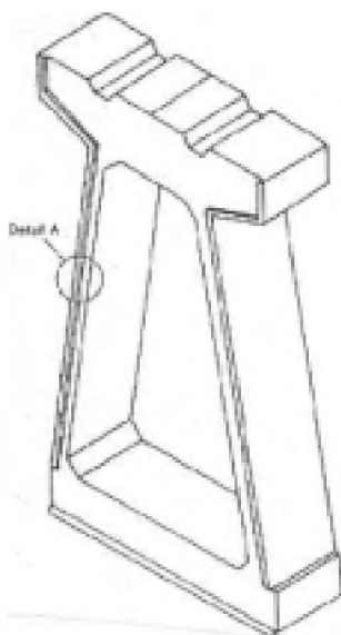
FIG. 17.13. Pre-cast unit details.
