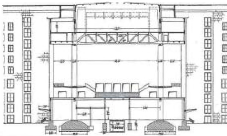
FIG. 17.5. Airport hall at Berlin Tempelhof Airport.
