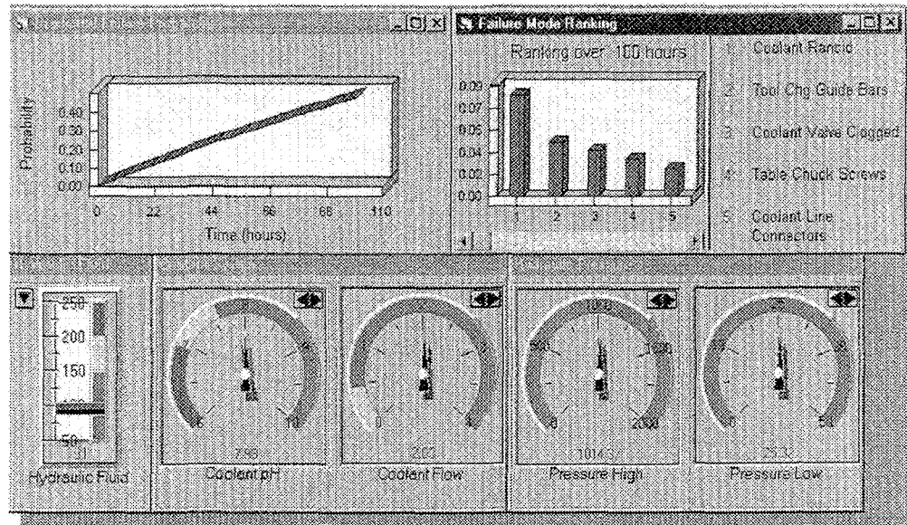
FIG. 5. Example man-machine interface for a smart component.
