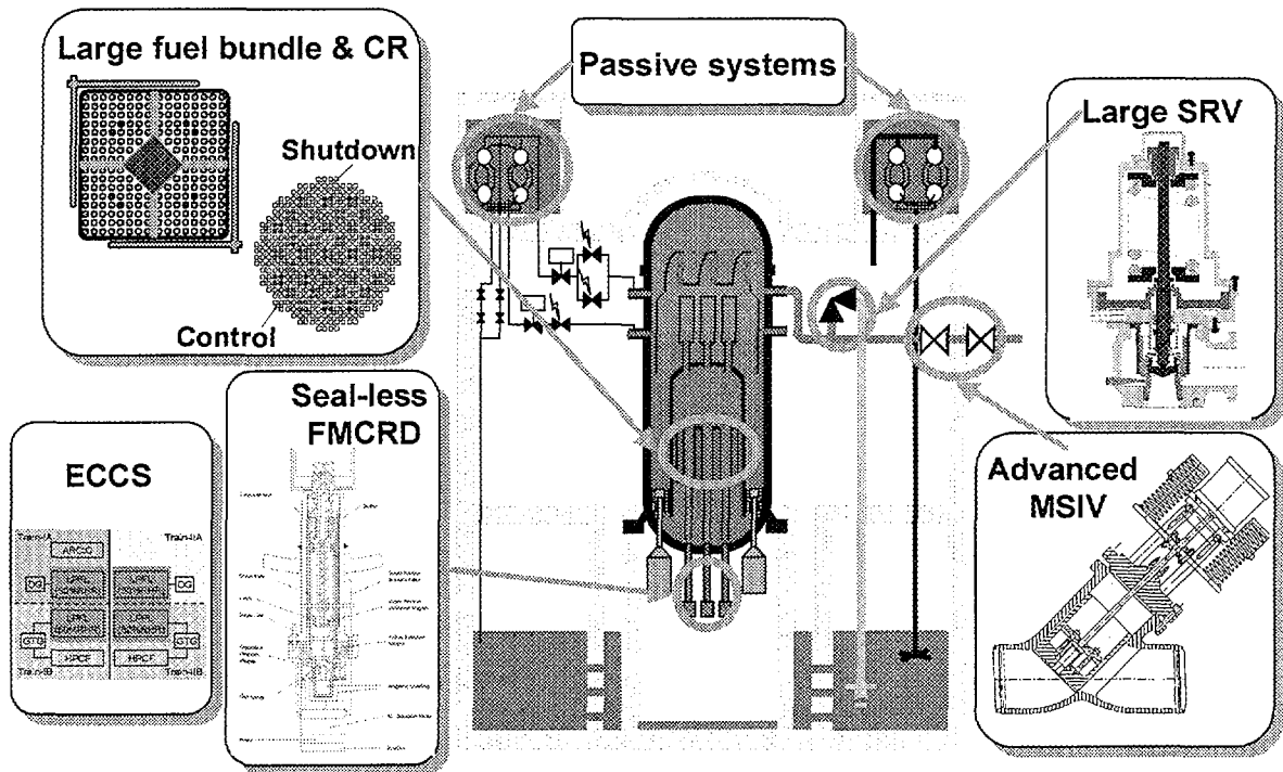
FIG. 2. ABWR-II design features.
