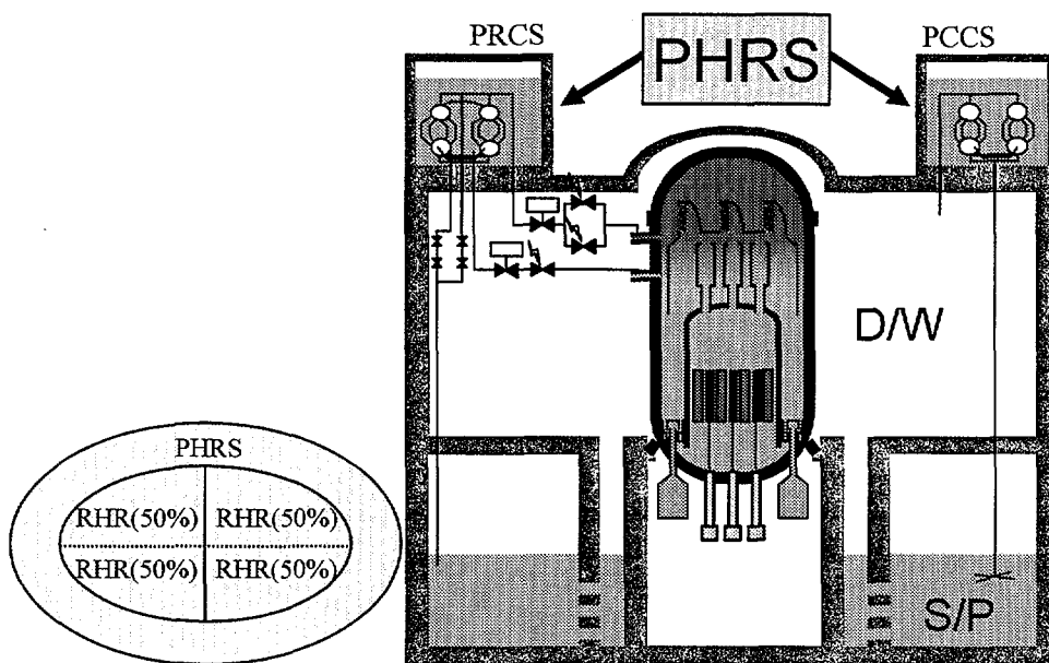
FIG. 10. Passive heat removal system.
