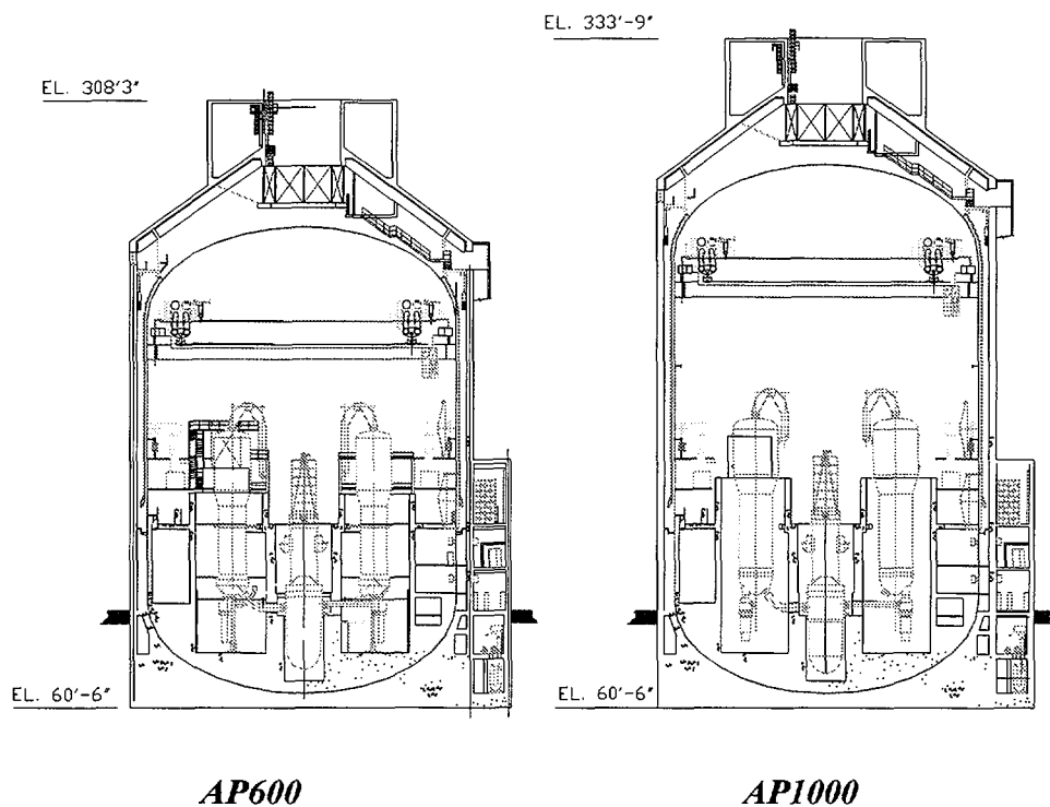
FIG. 1. Westinghouse AP1000 and AP600 plants (section).
