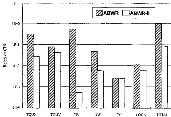
FIG. 11. Results of level 1 PSA for the ABWR-II and the ABWR [3]
