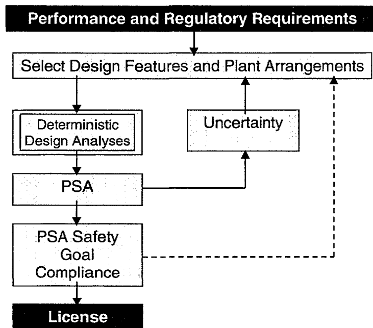
FIG. 1. Overview of the risk-based design and regulatory process.
