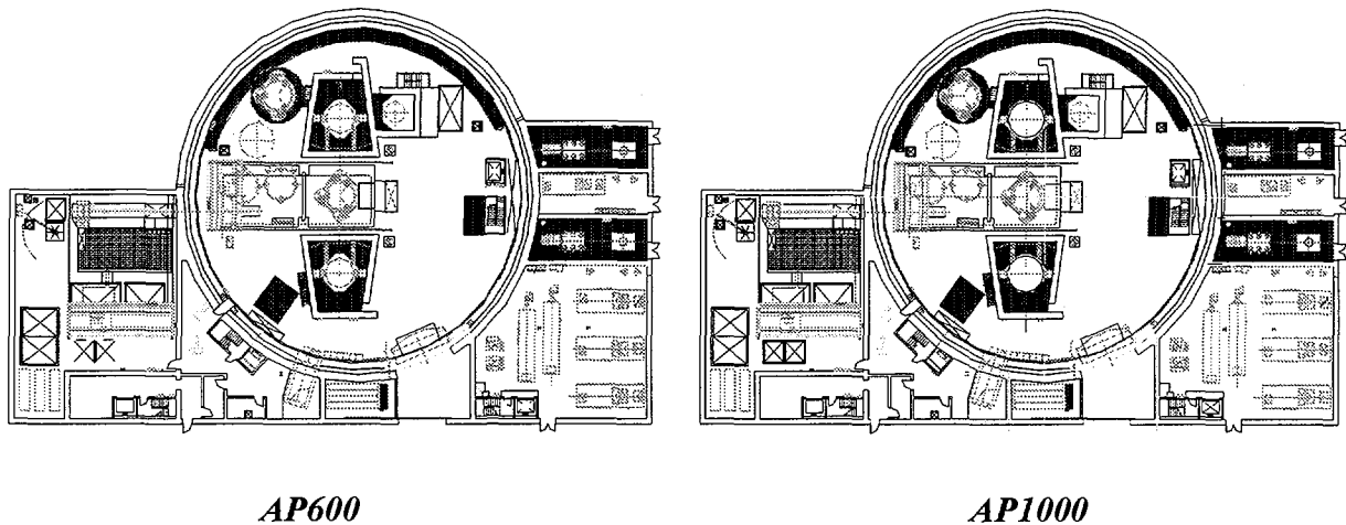
FIG. 2. Westinghouse AP1000 and AP600 plants (plan).
