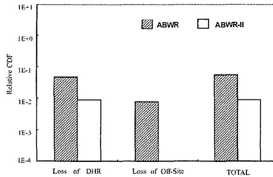
FIG. 13. Results of shutdown PSA for the ABWR-II and the ABWR [3].
