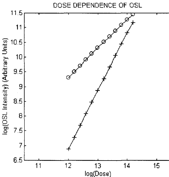
Figure 3: Dose dependence of pulse OSL when only one trapping state and one kind of recombination center are involved. (+) represents the results when the excitation starts with empty traps and (o) the results when n_0 = 0.9N . The values of the chosen parameters are given in the text.
