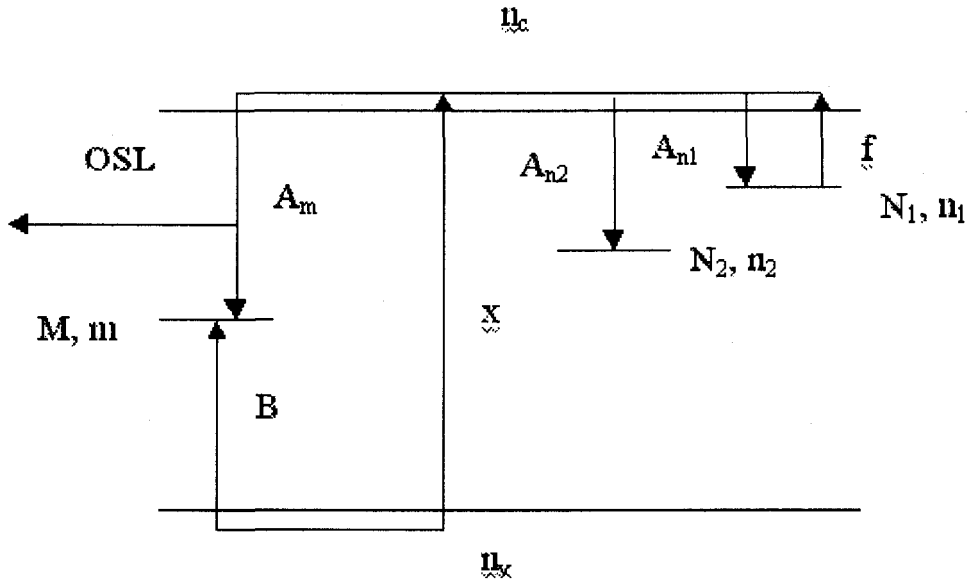
Figure 1. Energy level scheme for excitation and stimulation of OSL. An active trapping state, N_1 , and a center, M , are involved, as well as a disconnected competing trapping state, N_2 . For the case of only one trapping state, N replaces N_1 .
