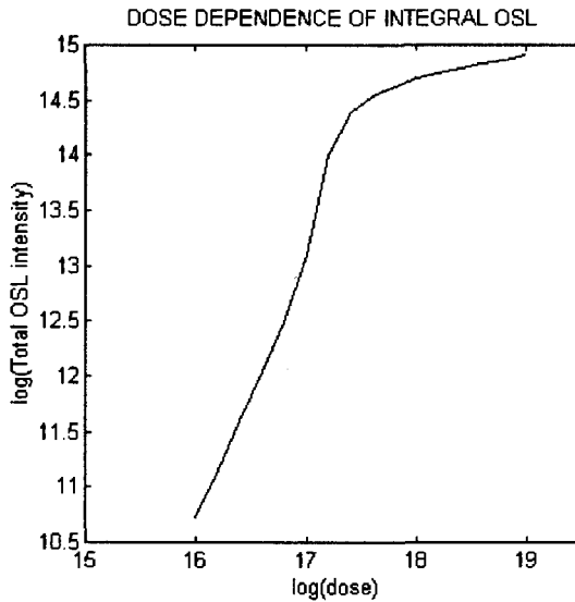
Figure 5: Simulated dose dependence of integrated OSL for the case of two trapping states and one kind of recombination center. The parameters are given in the text.
