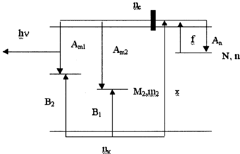
Figure 2: Energy level scheme for excitation and stimulation of OSL. An active trapping state N and two centers, one radiative, M_1 and one nonradiative, M_2 are involved.
