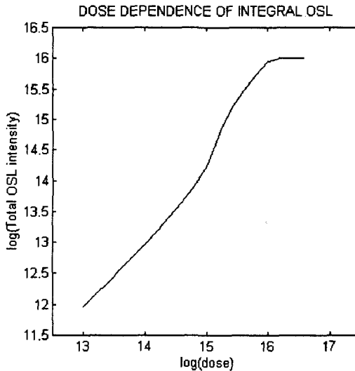
Figure 7: Simulated dose dependence of integrated OSL on the dose in the case of two kinds of recombination center and a single trapping state. The parameters are given in the text.
