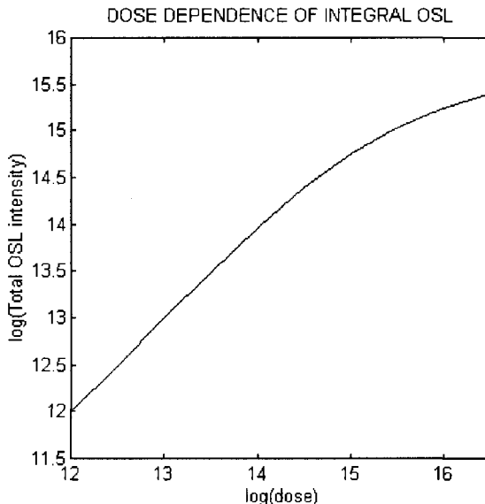
Figure 4: Dose dependence of the integral OSL under the same conditions as in Fig. 3.
