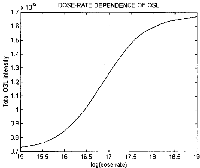
Figure 6: Dose-rate dependence of integral OSL in the case of two trapping states and one kind of recombination center. The chosen parameters are the same as in Fig. 5.
